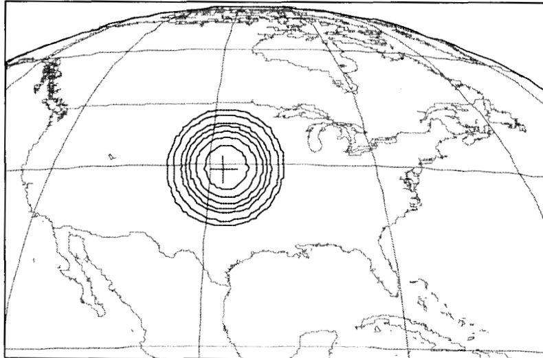
Figure A.6-1. Regional Beam Uplink Gain Contours - Sample Beam.
