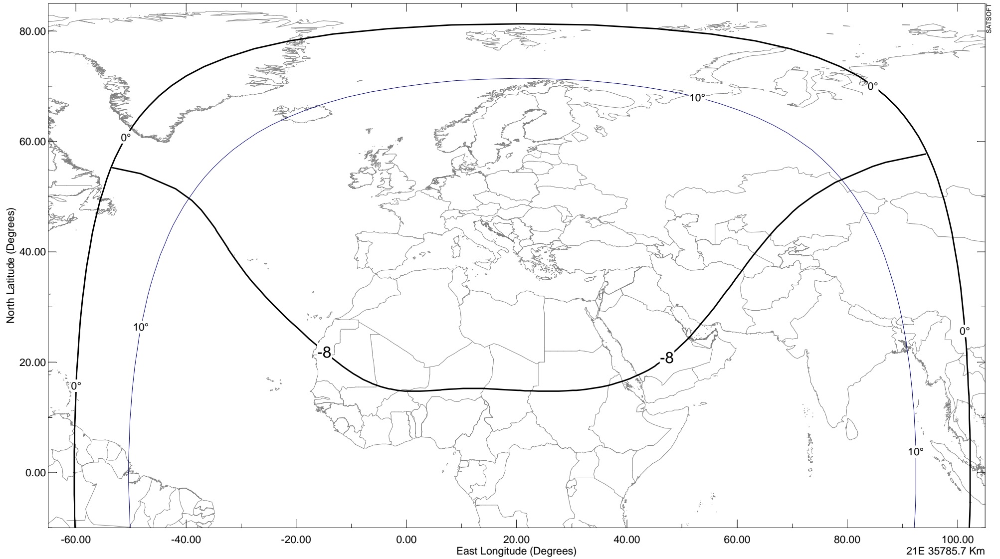
Figure 2: Downlink Service Area (-8 dB Contour)
