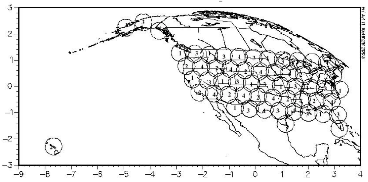
Figure 4-4 – Rainbow Ka Four Color Frequency Reuse – Eastern Orbital Slot
