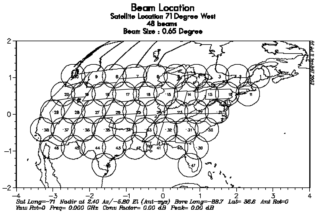
Figure 4-4 – Rainbow Ka Four Color Frequency Reuse – Eastern Orbital Slot
