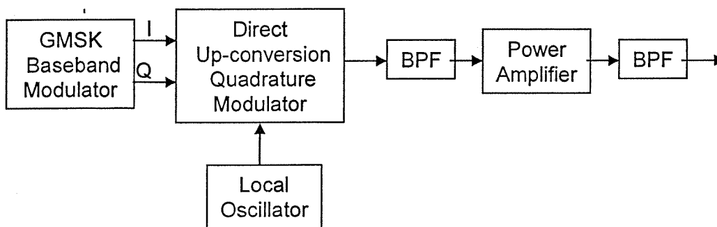
Figure 1 Transmitter Architecture
