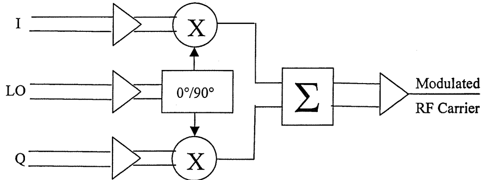
Figure 4 Direct Up-conversion Quadrature Modulator
