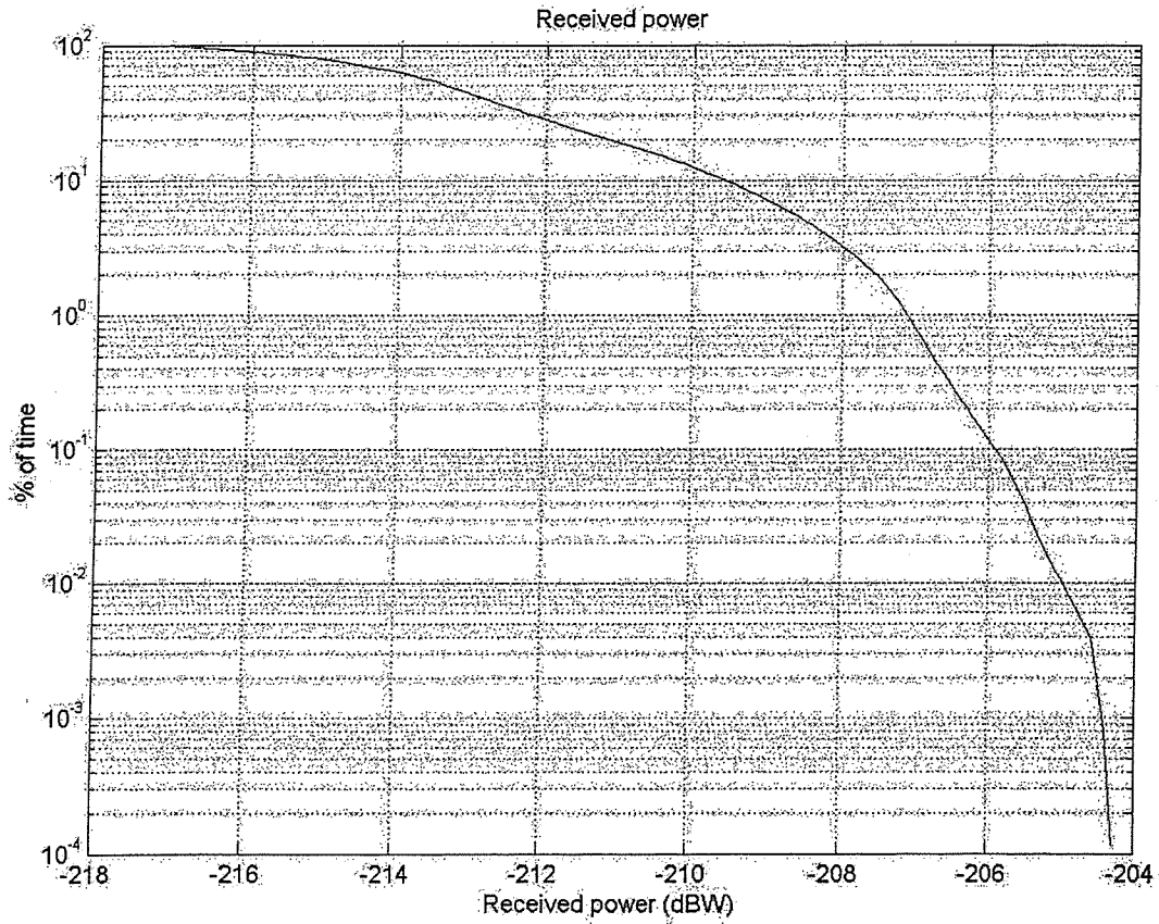
FIGURE 6 HYDROS - Measurement period
