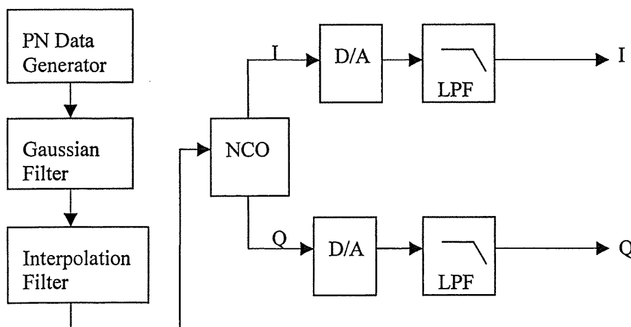
Figure 2 GMSK Baseband Modulator
