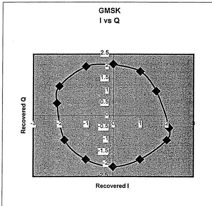
Fig. 1.2.13a. FACS modulator #1
