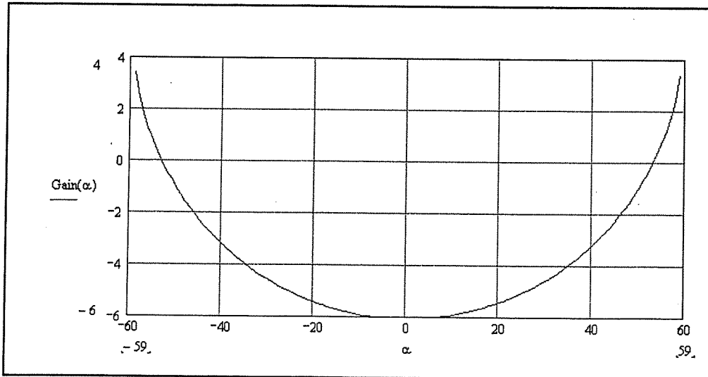
FIGURE 2 Non-GSO MSS Satellite Receive and Transmit Antenna Patterns
