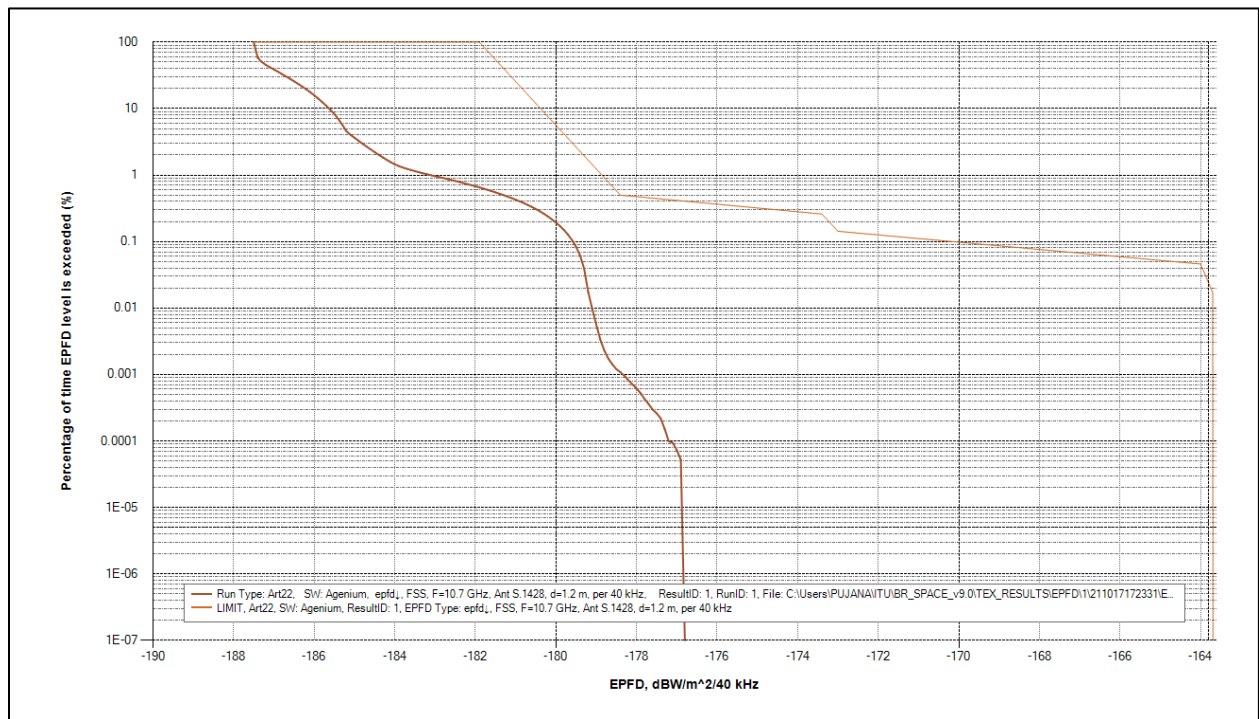
Figure 2: Compliance with RR Table 22-1A for 1.2m antenna, 40 kHz reference bandwidth
