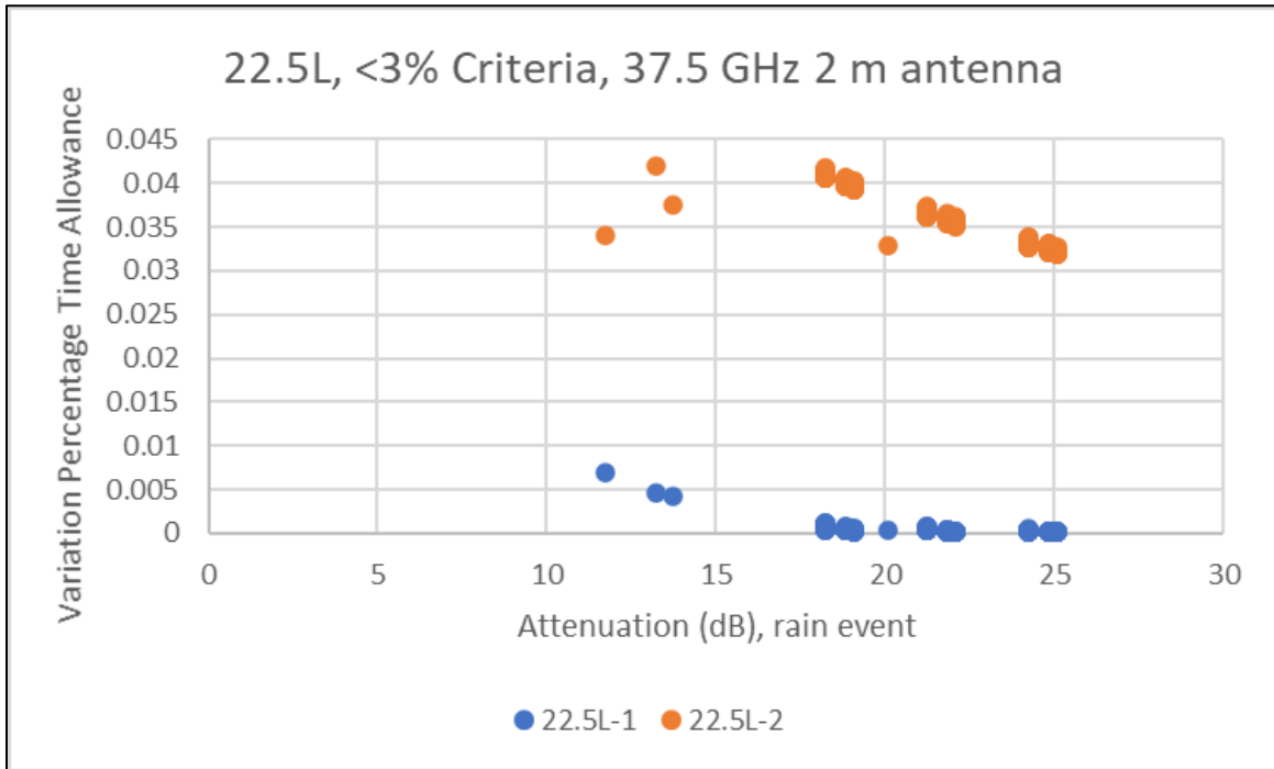
Figure 3: Variation in Percentage of Time Allowance for 22.5L-1 (C/N) Criteria and 22.5L-2 (spectral efficiency) Criteria for the 2m Antenna
