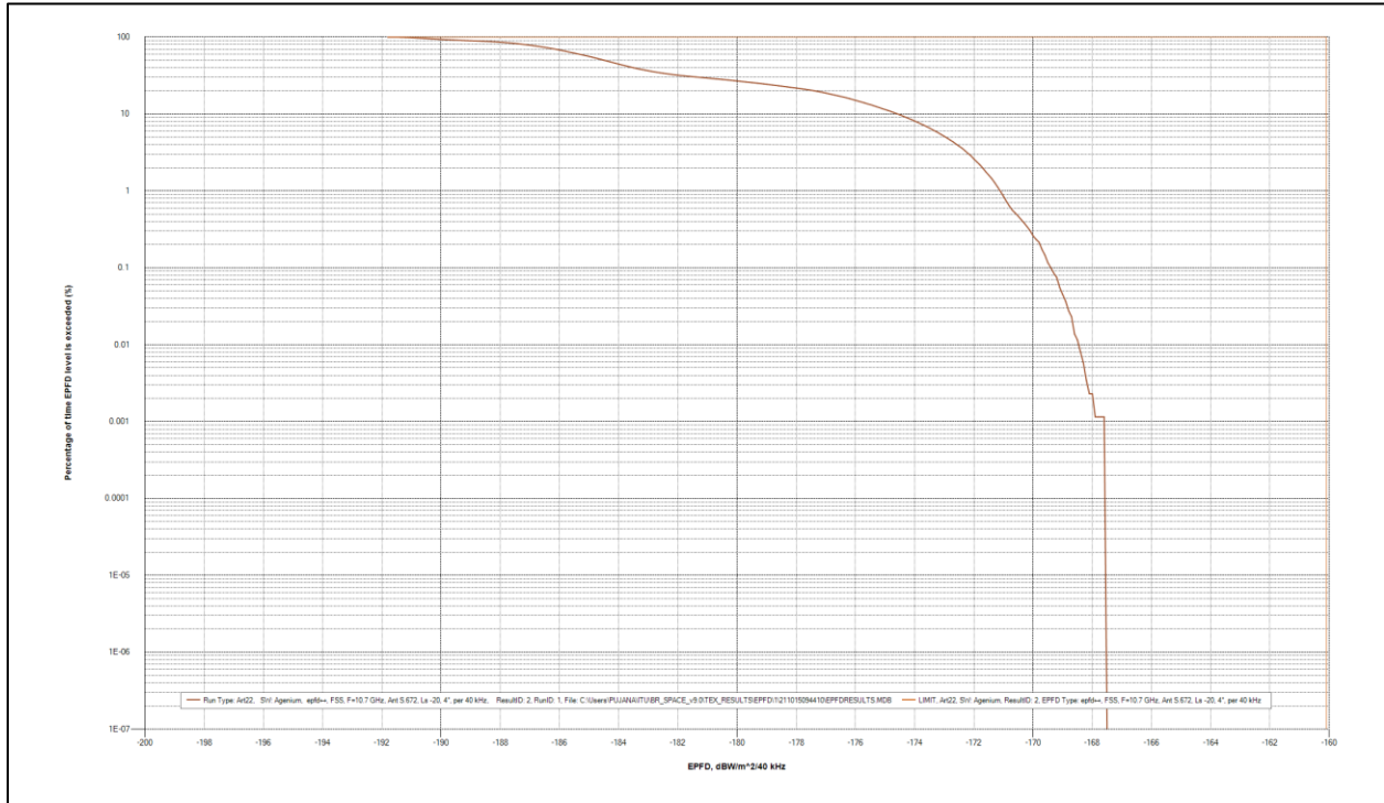
Figure 14: 10.7 GHz, 40 kHz Reference Bandwidth, Beamwidth of 4°, FSS downlink
