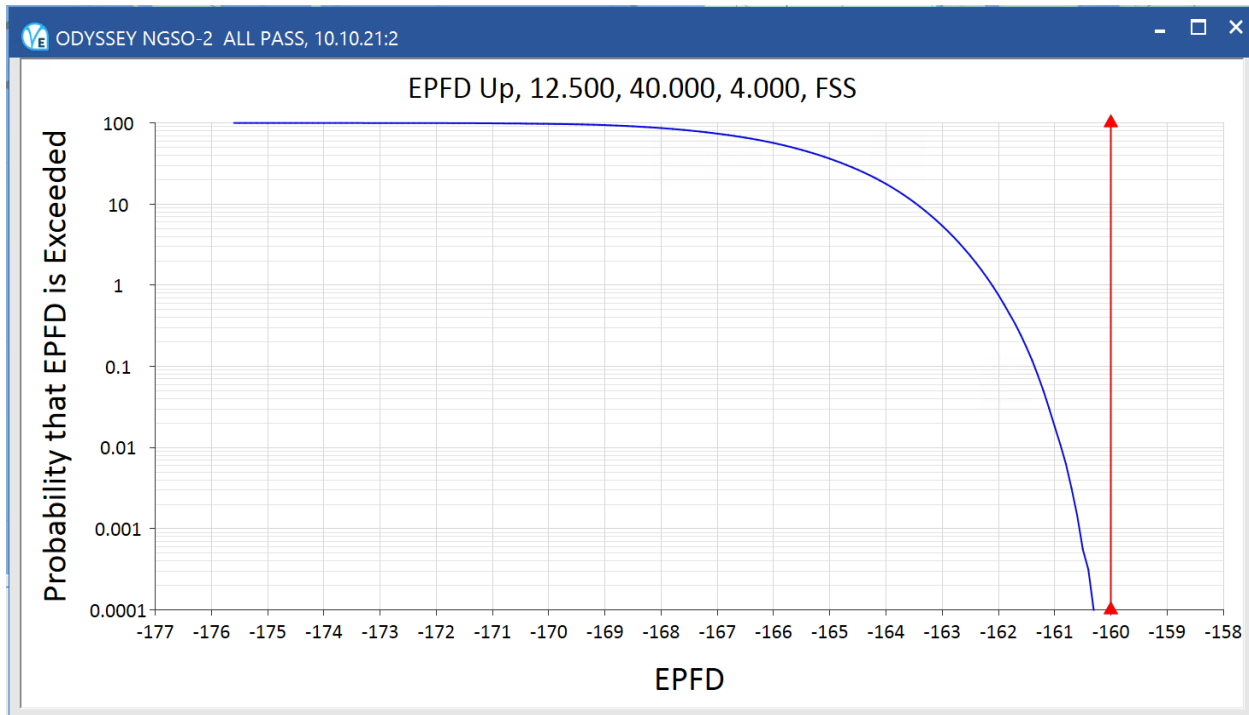
Figure 13: 12.5 GHz, 40 kHz Reference Bandwidth
