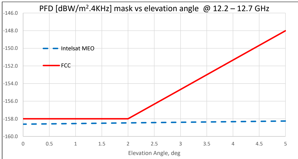
Figure 4: PFD Mask vs. Elevation Angle at 12.2-12.7 GHz for User Beams
