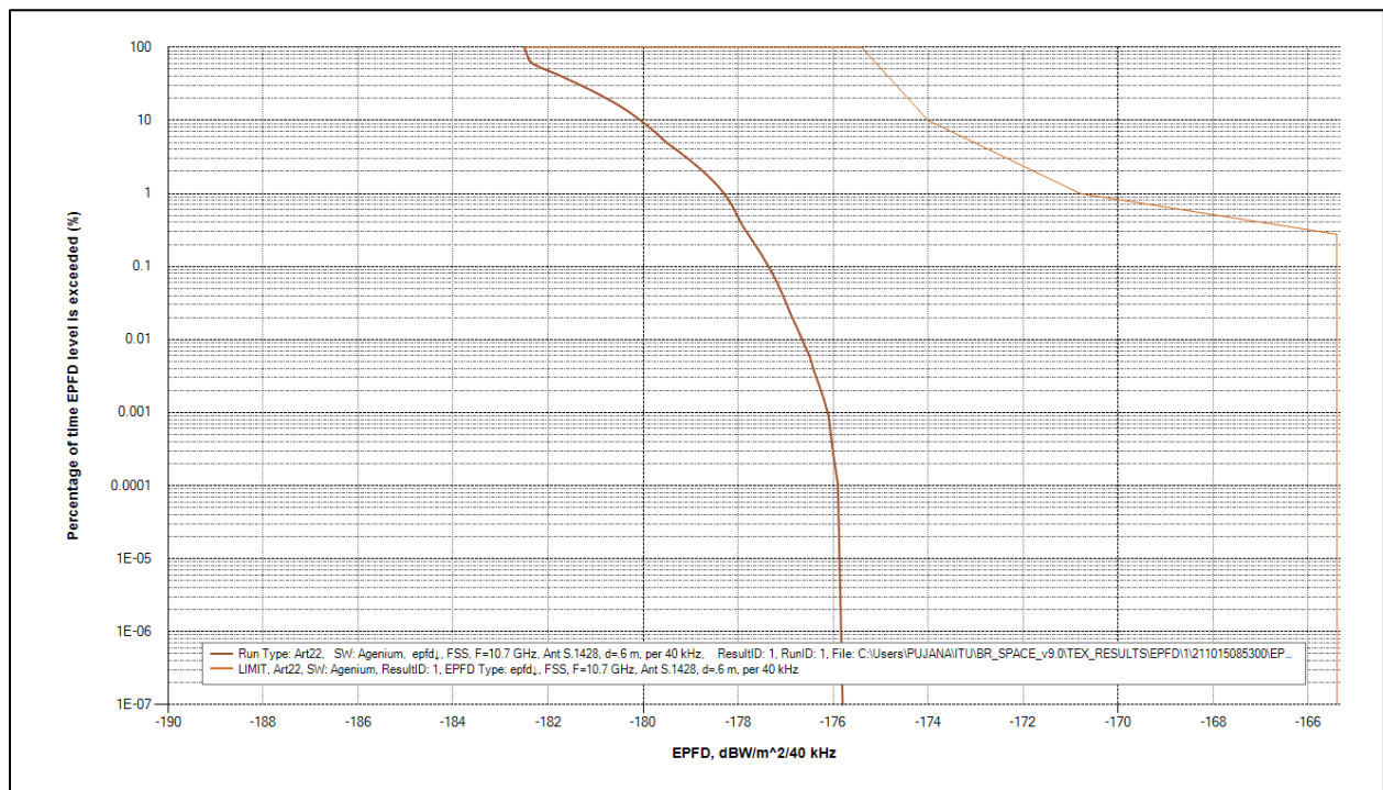
Figure 1: Compliance with RR Table 22-1A for 60cm antenna, 40 kHz reference bandwidth
