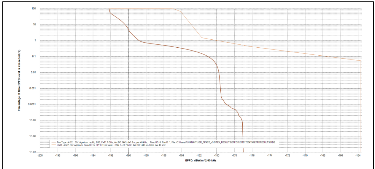
Figure 10: Compliance with RR Table 22-1D for 1.8m antenna, 40 kHz reference bandwidth
