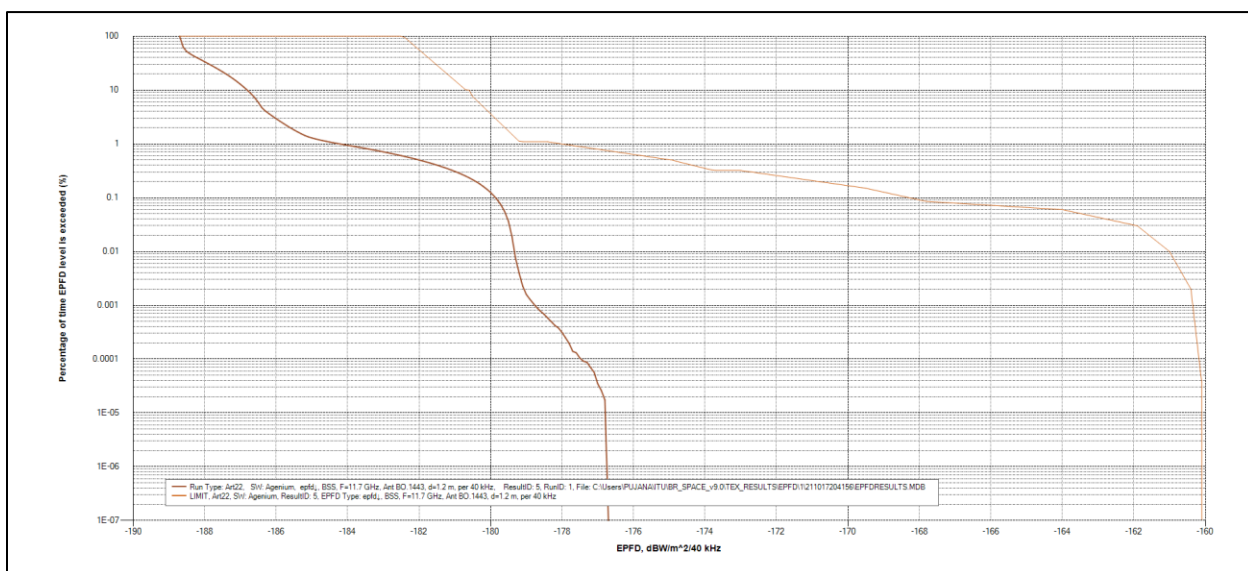
Figure 9: Compliance with RR Table 22-1D for 1.2m antenna, 40 kHz reference bandwidth
