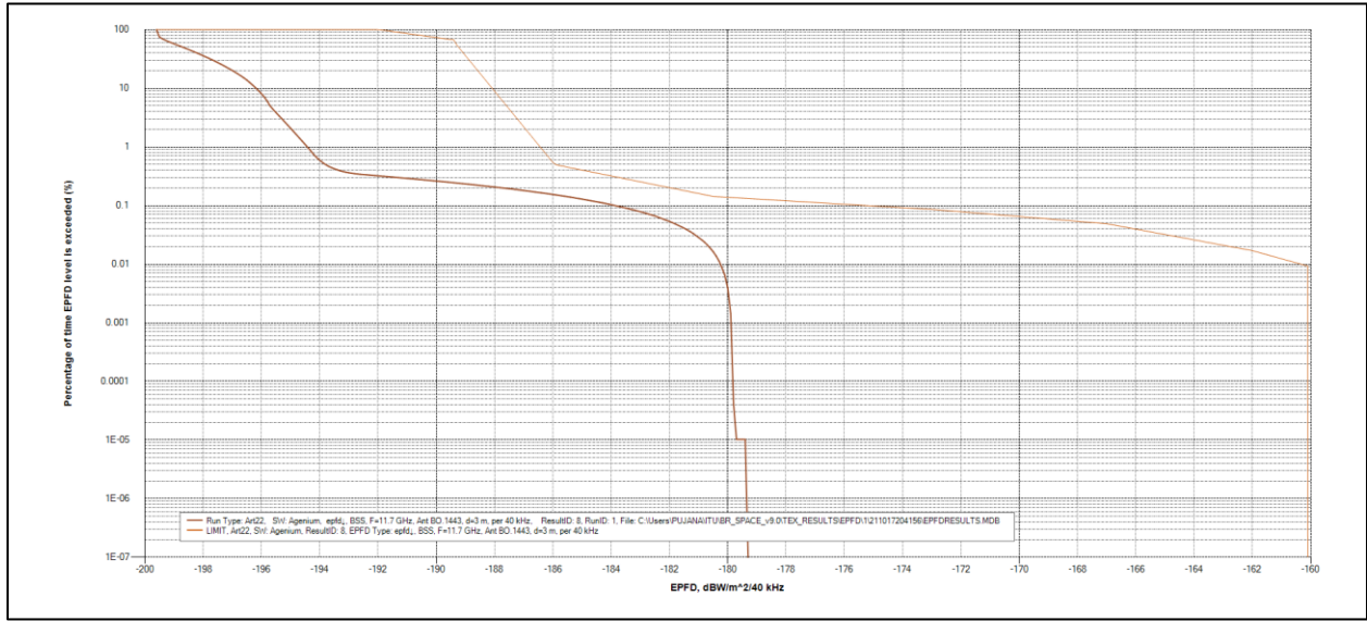
Figure 12: Compliance with RR Table 22-1D for 3m antenna, 40 kHz reference bandwidth
