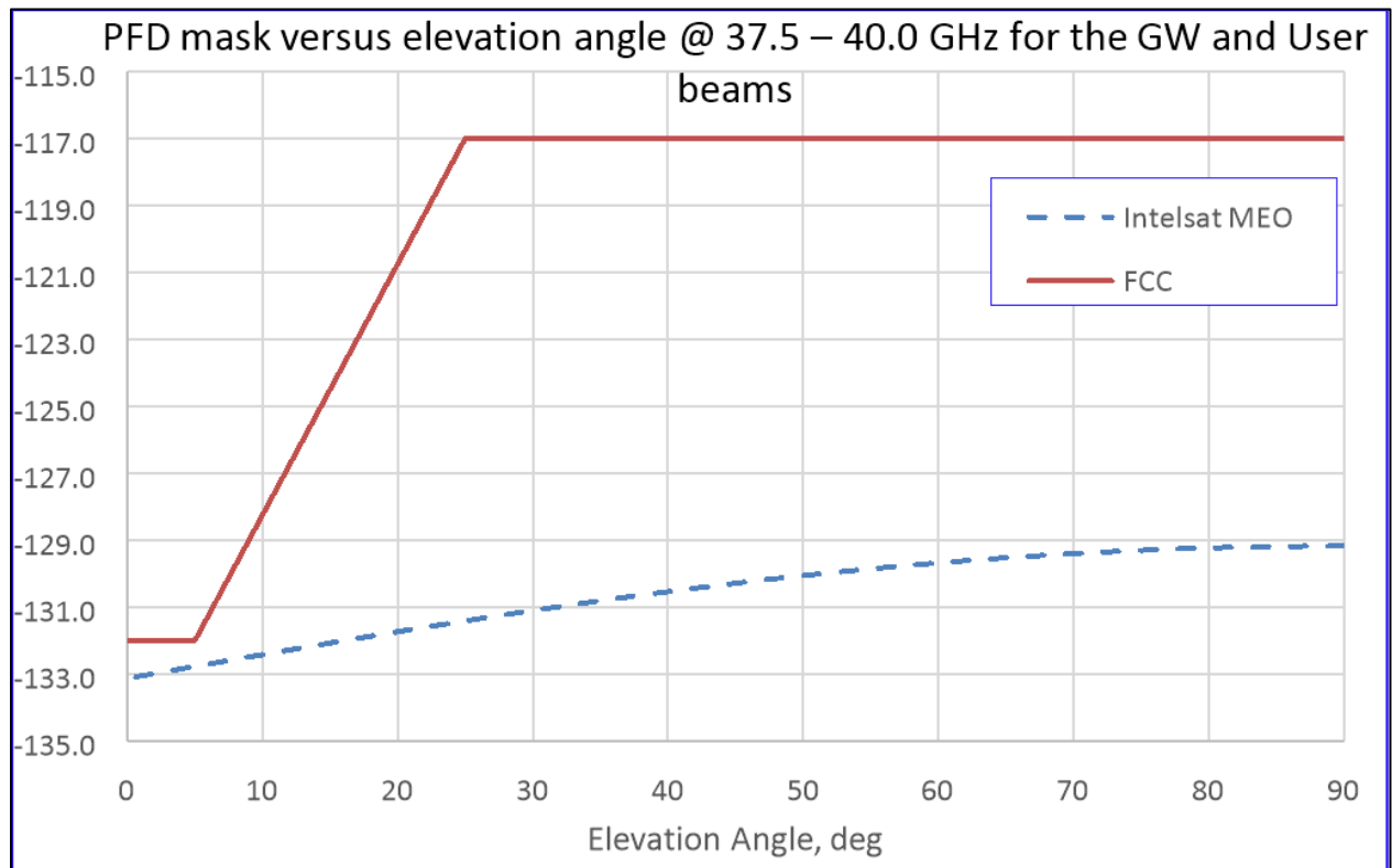
Figure 5: PFD Mask vs. Elevation Angle at 37.5-40.0 GHz for Gateway and User Beams
