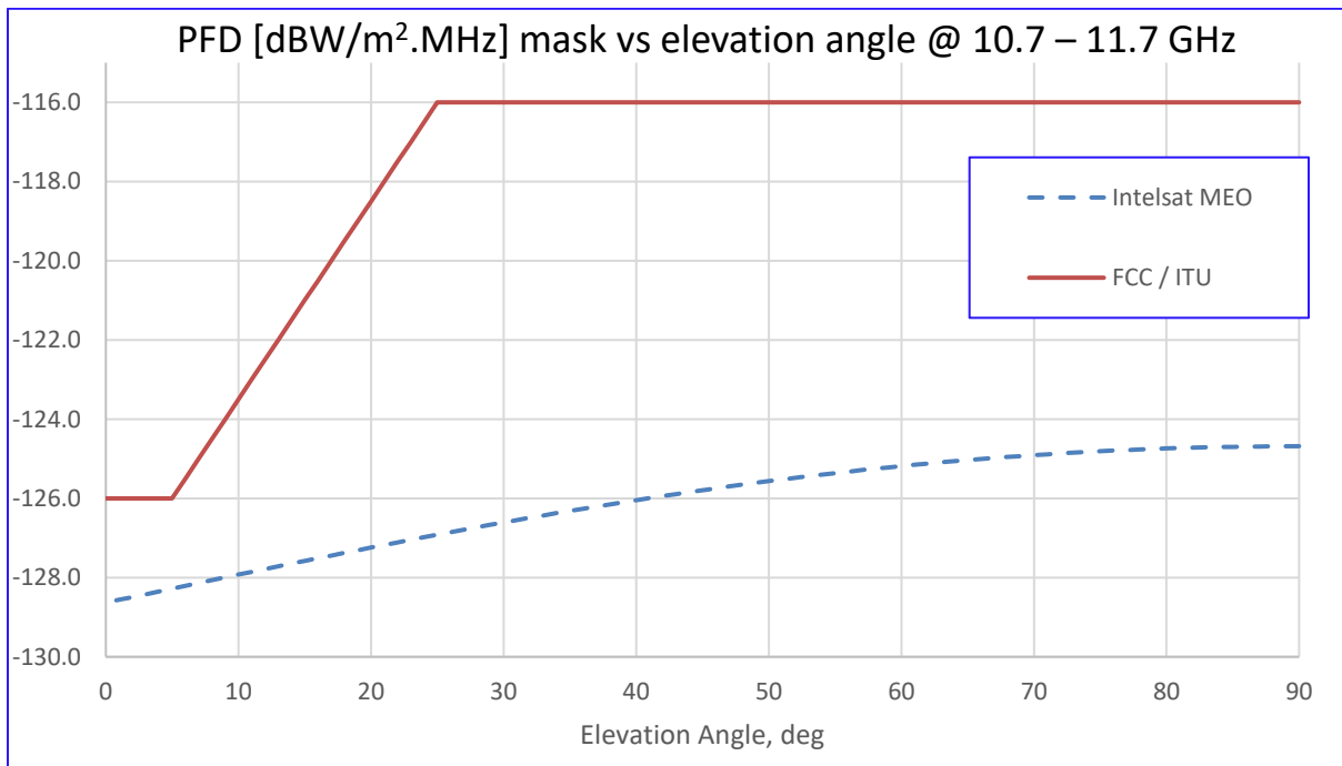
Figure 2: PFD Mask vs. Elevation Angle at 10.7-11.7 GHz for User Beams
