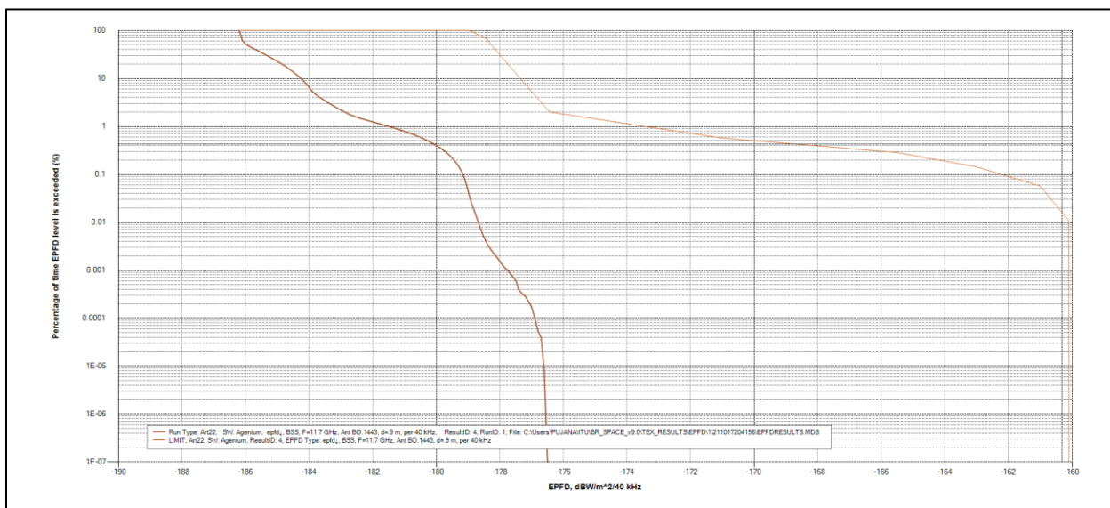
Figure 8: Compliance with RR Table 22-1D for 90cm antenna, 40 kHz reference bandwidth
