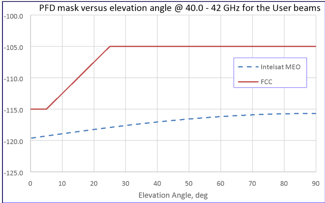
Figure 6: PFD Mask vs. Elevation Angle at 40.0-42.0 GHz for User Beams
