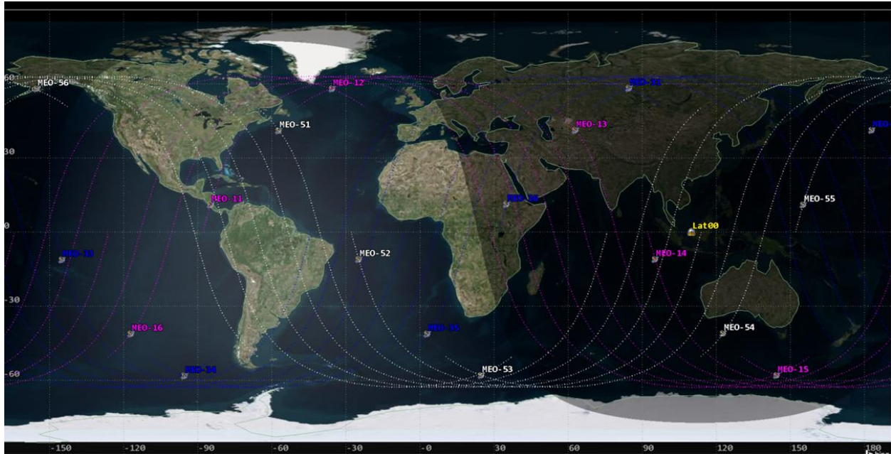
Figure 1: Snapshot of a Subset of the Intelsat MEO Constellation Shown in Table 1
