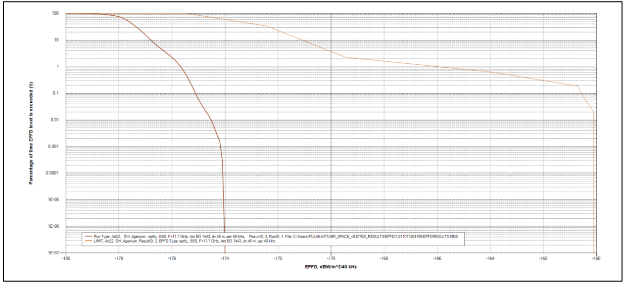
Figure 6: Compliance with RR Table 22-1D for 45cm antenna, 40 kHz reference bandwidth
