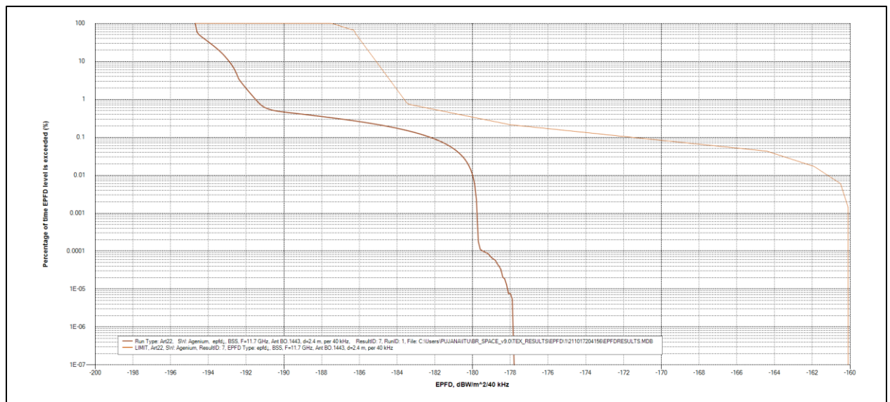
Figure 11: Compliance with RR Table 22-1D for 2.4m antenna, 40 kHz reference bandwidth
