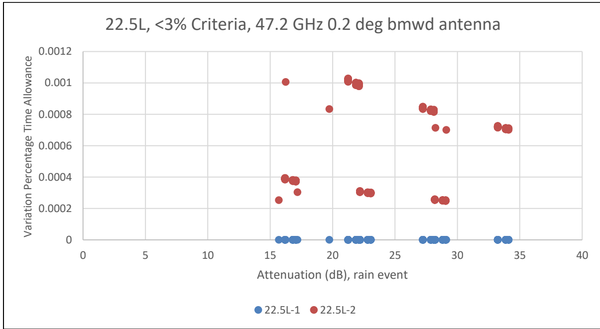
Figure 1: Variation in Percentage of Time Allowance for 22.5L-1 (C/N) Criteria and 22.5L-2 (spectral efficiency) Criteria for the 0.2° Beamwidth GSO Antenna
