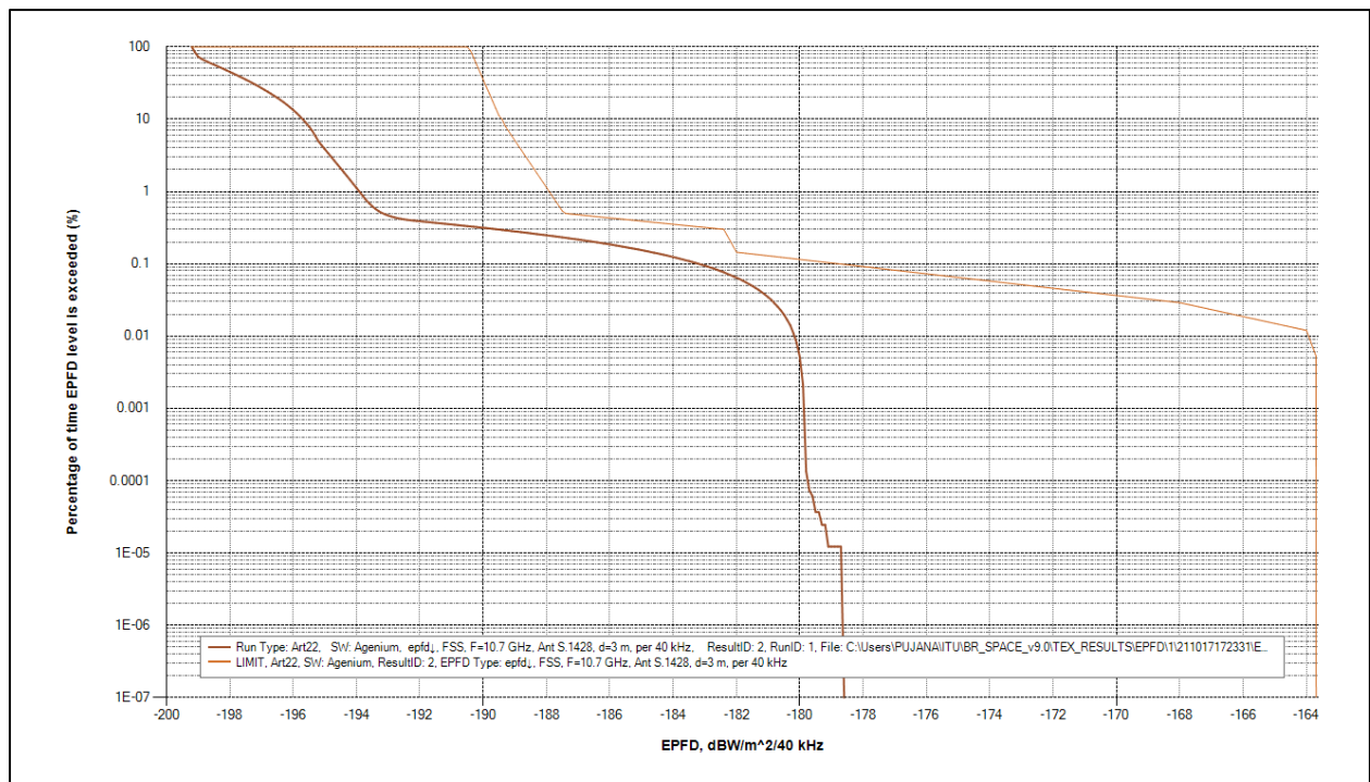
Figure 3: Compliance with RR Table 22-1A for 3m antenna, 40 kHz reference bandwidth
