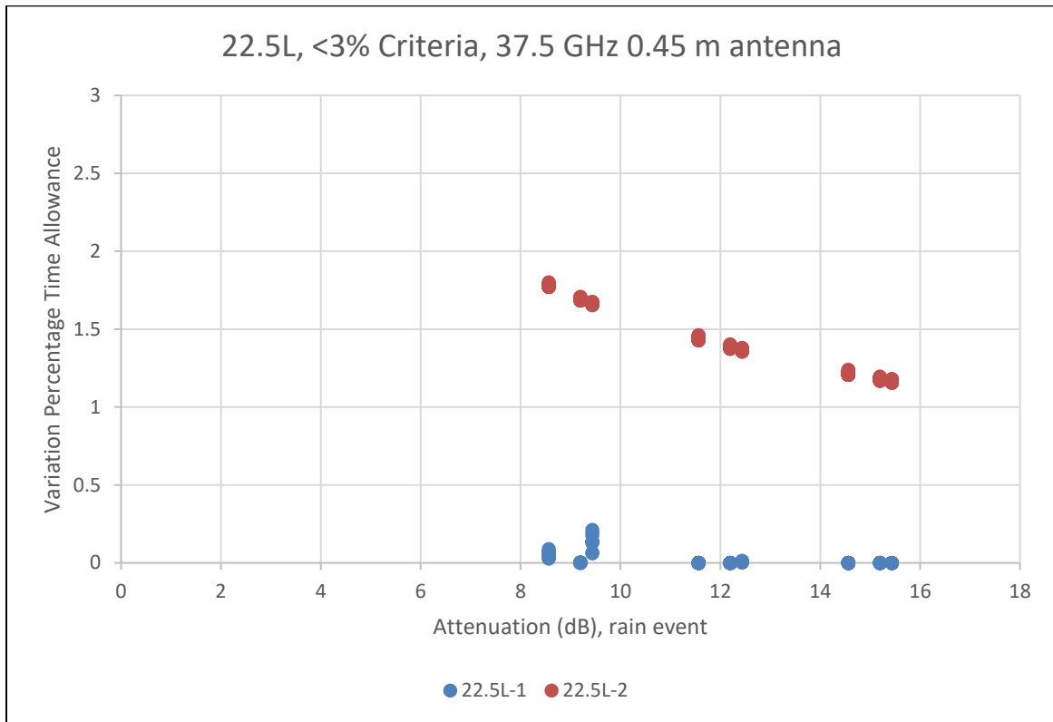
Figure 2: Variation in Percentage of Time Allowance for 22.5L-1 (C/N) Criteria and 22.5L-2 (spectral efficiency) Criteria for the .45m Antenna
