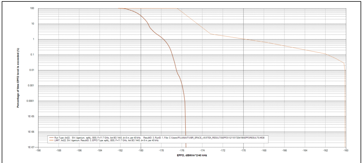
Figure 7: Compliance with RR Table 22-1D for 60cm antenna, 40 kHz reference bandwidth
