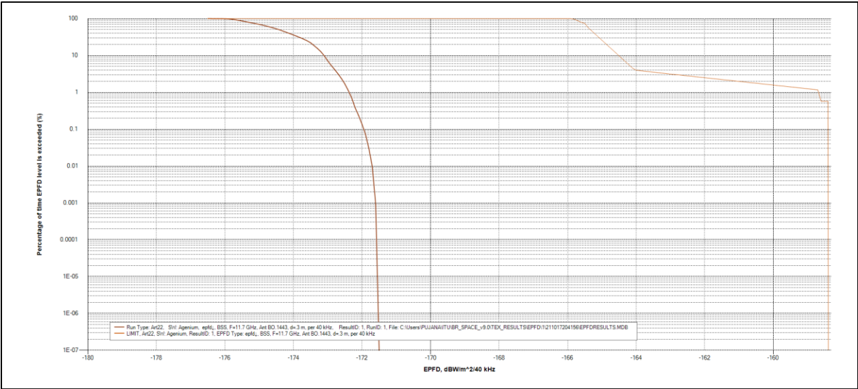
Figure 5: Compliance with RR Table 22-1D for 30cm antenna, 40 kHz reference bandwidth
