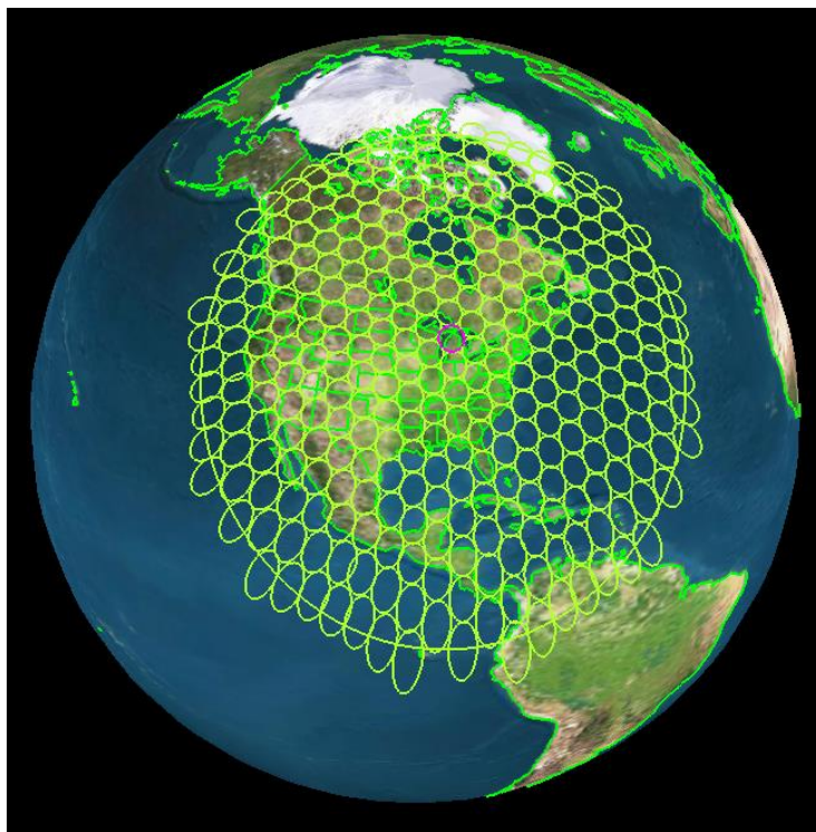
Beam Pack of service link beams of ENA satellite at nominal altitude over North America. Note: Alaska is covered by an adjoining Pacific satellite's beams.
