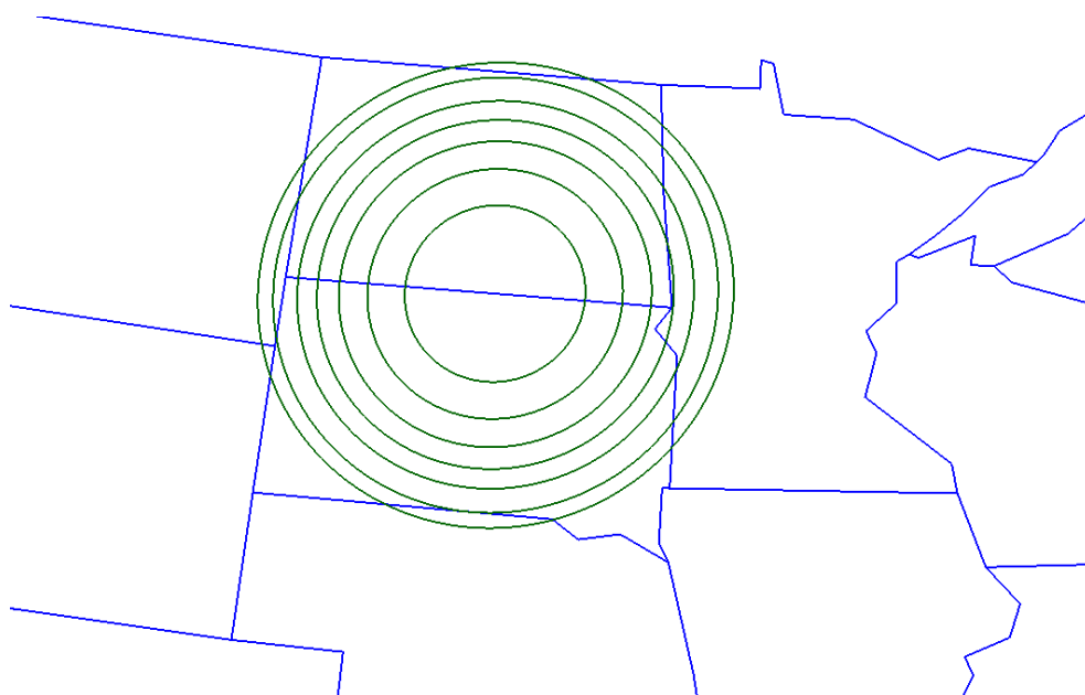
Contours of a single nadir pointing service link downlink spot beam, showing -2, -4, -6, -8, -10, -15, -20 dB contours from peak. Uplink spot beams are congruent with downlink spot beams. Ku-band TT&C channels uses these spot beams.
