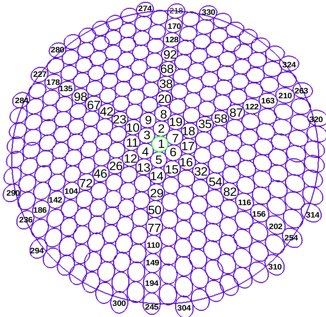
The 313 PLEIADES service spot beam arrangement and numbering.
