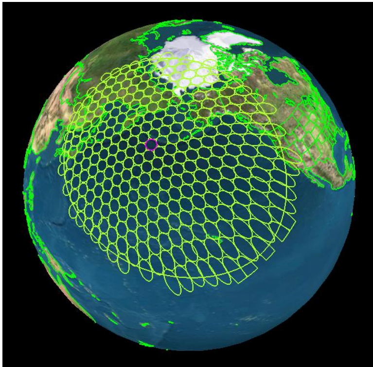
Figure 17, Beam array from the N Pacific active arc, nominal case
