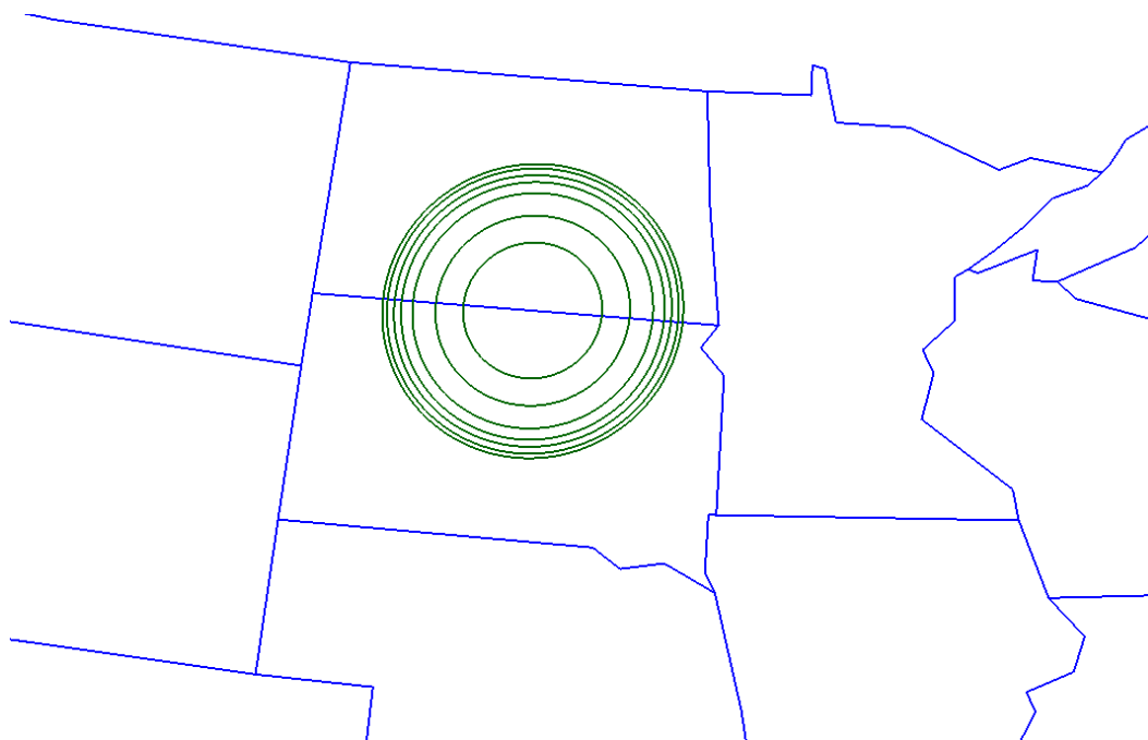
Figure 19, Representative single feeder link nadir pointing downlink 19 GHz beam contours, showing -2, -4, -6, -8, -10, -15, and -20 dB contours from peak. Uplink Feeder 19 GHz link beams are congruent with this.
