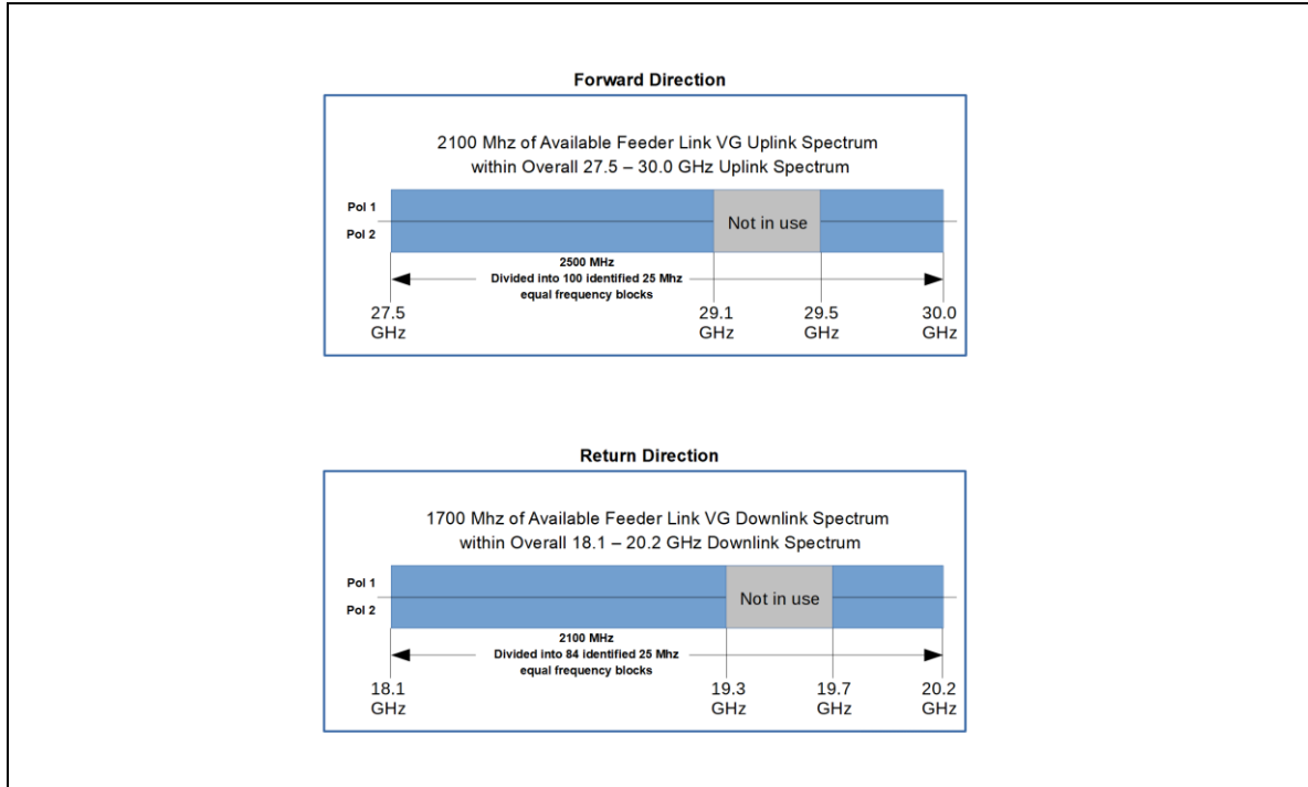
Figure 12, PLEIADES feeder link spectrum
