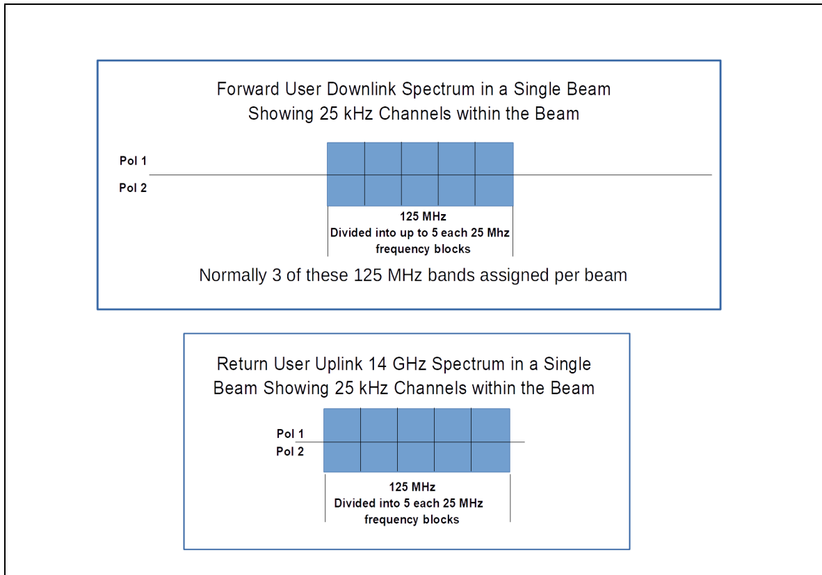
Figure 13, Channels within user link beam spectrum.
