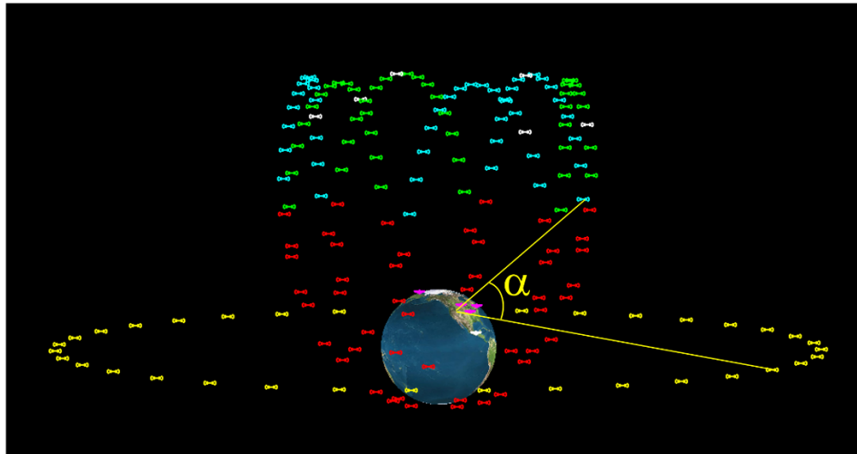
Figure 1, A snapshot view of the Virtual Geo framework from space , positions to scale, shown populated with a large number of satellite systems sharing the framework. A single system might only use one or two satellites per active arc or lobe shown. The Blue and green lobes are active arcs and are geostationary. Red satellites here are inactive and in transit between active arcs, only the blue or green satellites shown are active and radiate. This also illustrates the substantial angular separation “ \alpha ” between the closest active framework satellites and any GSO satellite ( \alpha > 39^\circ ). Southern active arc satellites in the framework, not shown here to simplify the illustration, are similar, except the active satellites operate to the South of the Earth by equal distances.
