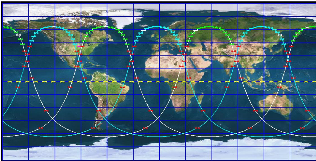
Figure 4, The ground tracks for the Northern Virtual Geo framework, shown in blue and white for the 2 Northern ground tracks. Southern ground tracks are similar but inverted by latitude and displaced 20.3 degrees East. As before, active satellites are blue or green depending on the ground track, inactive satellites are red. All satellites shown are evenly spaced in time. Note the relatively even geographic satellite spacing within the active arc and the rapid satellite acceleration outside of them
