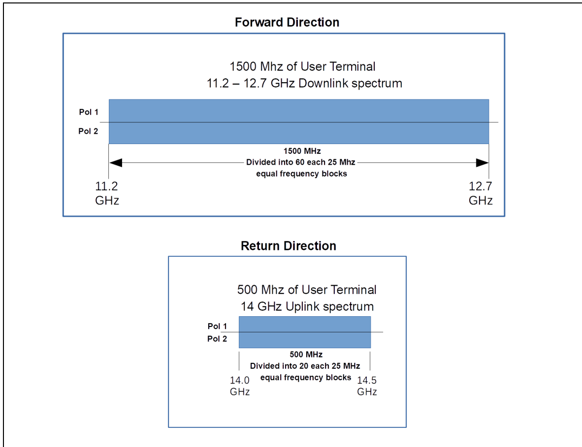
Figure 11, PLEIADES user link spectrum
