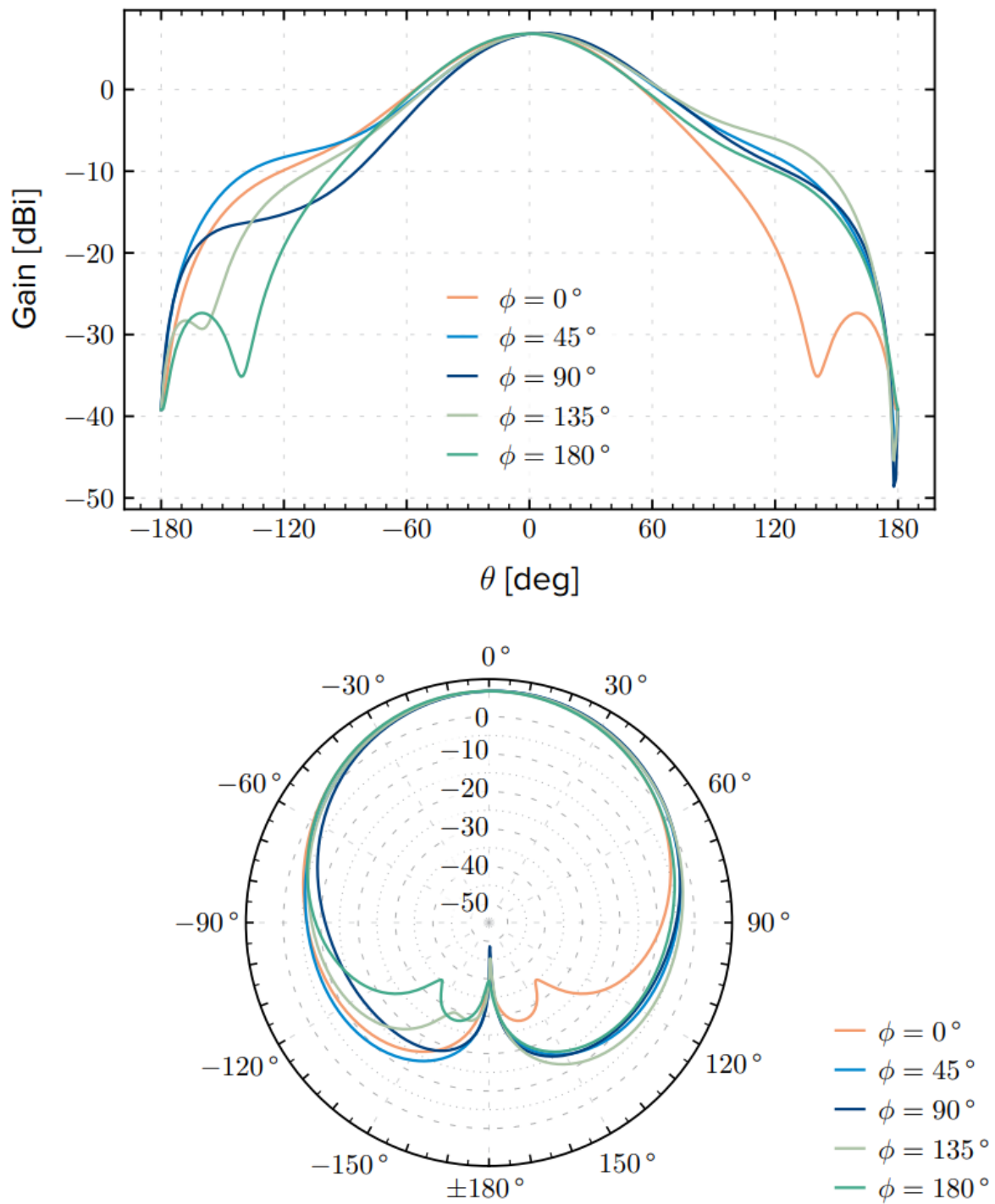
Figure 6: Simulated Radiation Pattern of the antenna at 2.245 GHz
