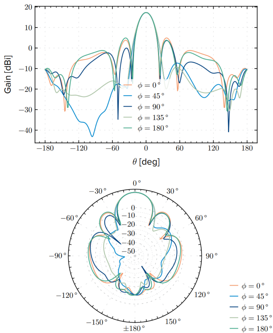
Figure 5: Simulated Radiation Pattern
