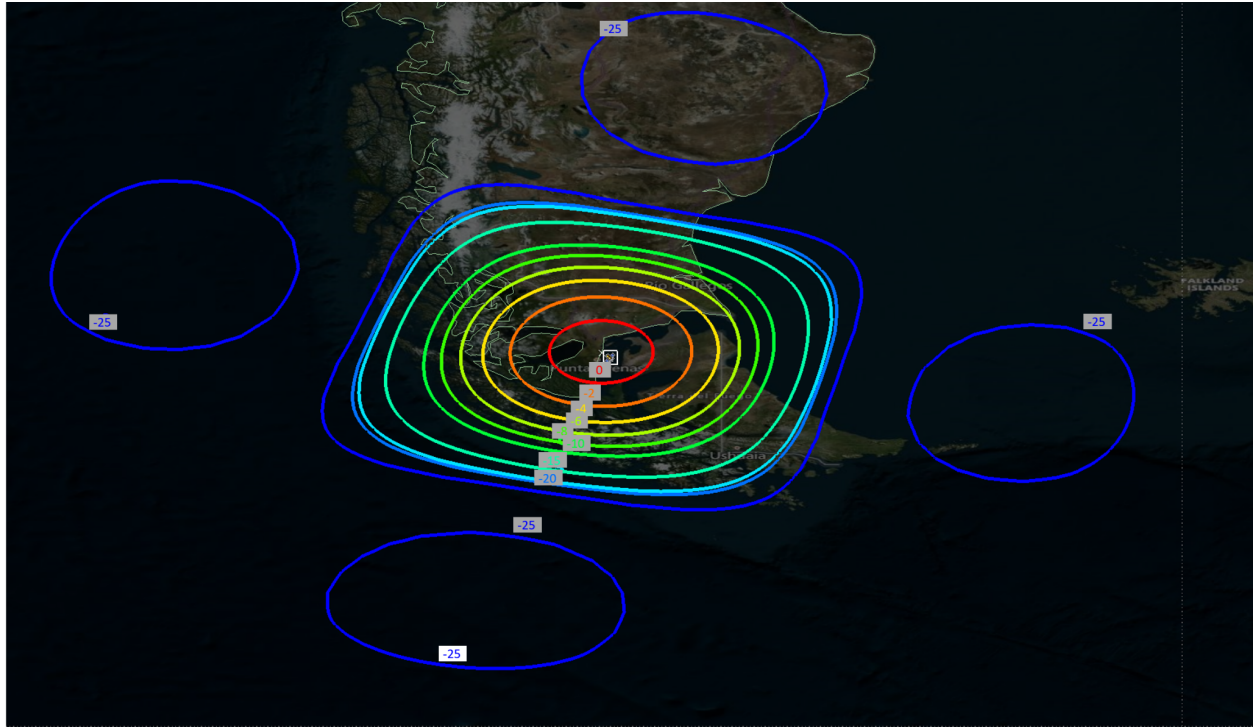
Projection of Nadir X-band Downlink Beam (XDA and XDB) over Punta Arenas, Chile.
