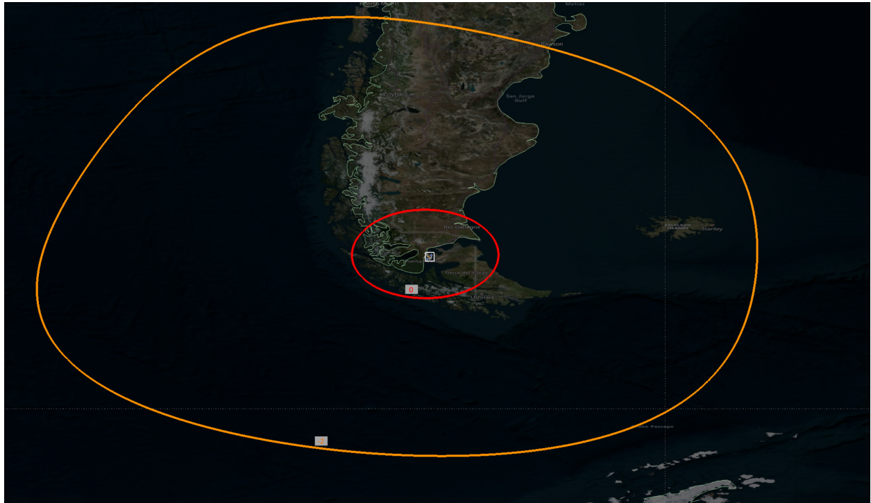
Projection of S-band Uplink (SUA) and Downlink Beam (SDA) over Punta Arenas, Chile. Note: S-Band antenna gain contours at -4 dB below max gain are beyond the horizon and, accordingly, are not shown in the images.
