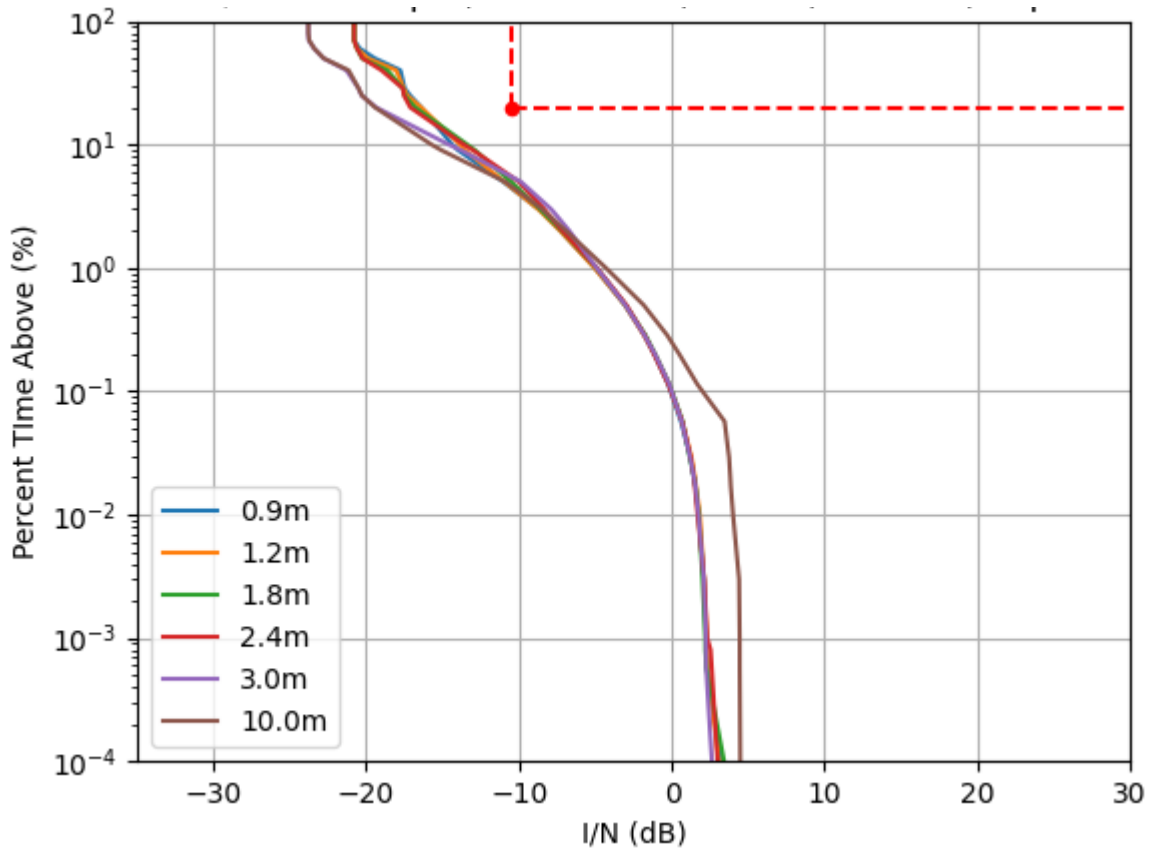
Figure A-2. Gen 2 Kuiper Satellite Downlink I/N CCDF
