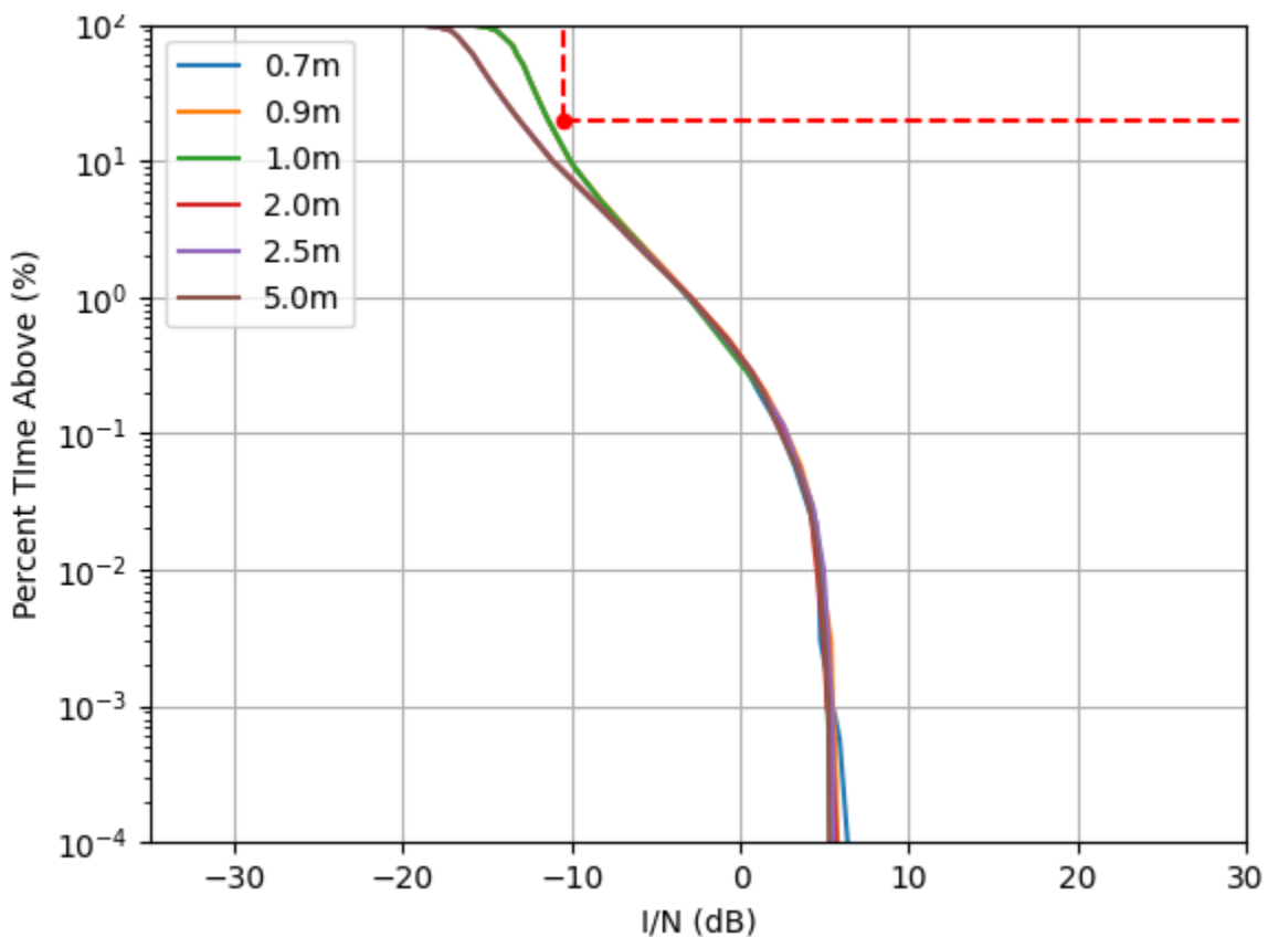
Figure A-1. Gen 2 Kuiper Satellite Downlink I/N CCDF
