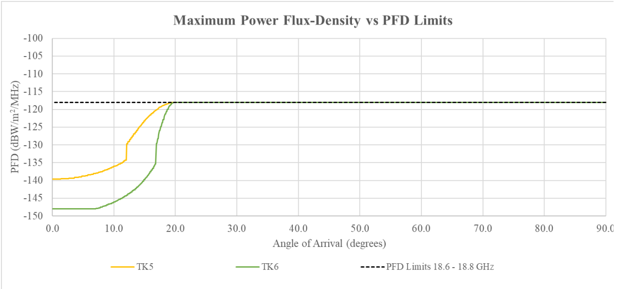
Figure 2. Gen 2 Kuiper Satellite CT Downlink Power Flux-Density Levels in the 18.6 – 18.8 GHz Band
