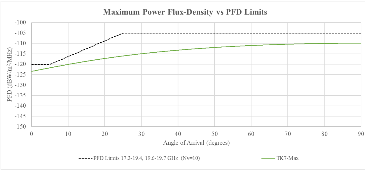
Figure 3. Gen 2 Kuiper Satellite TT&C Downlink Power Flux-Density Levels in the 19.25 – 19.4 GHz Band
