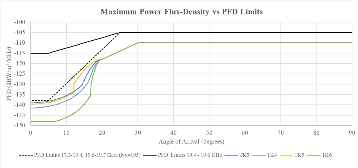
Figure 1. Gen 2 Kuiper Satellite GW and CT Downlink Power Flux-Density Levels in the 17.3 – 19.7 GHz Band
