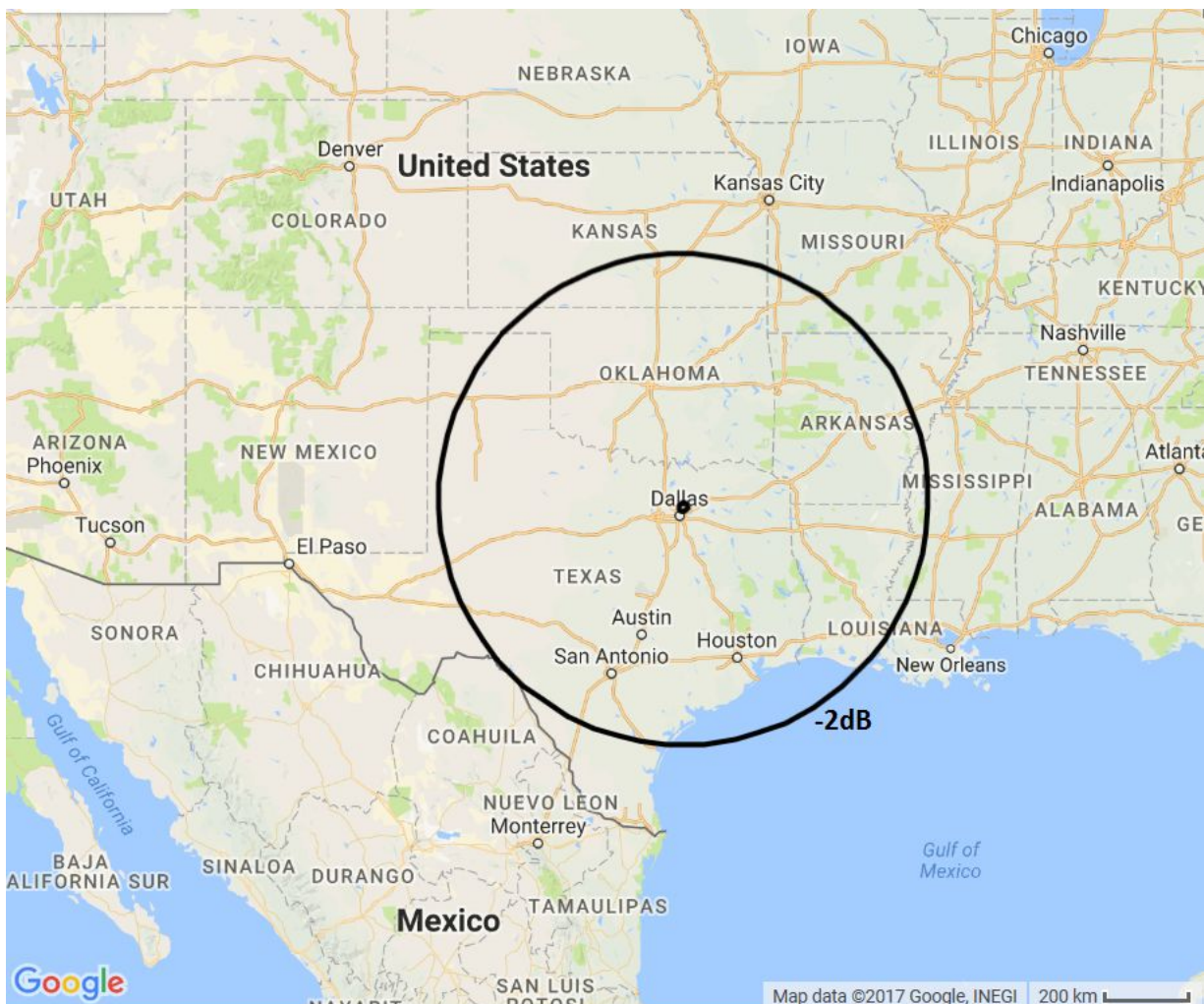
Figure 4: Orbital plane 4- Apogee 450Km
