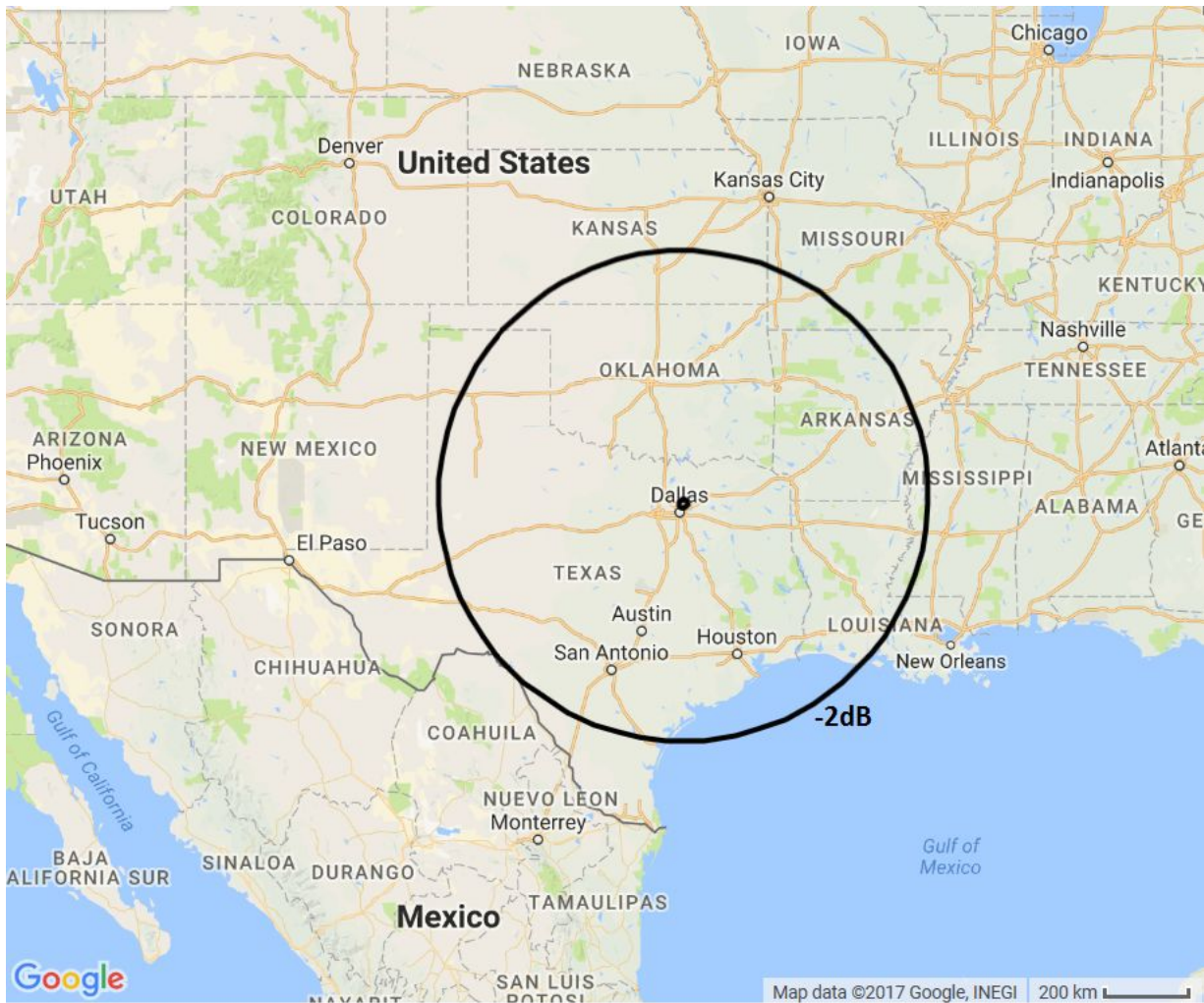
Figure 2: Orbital plane 2- Apogee 450Km
