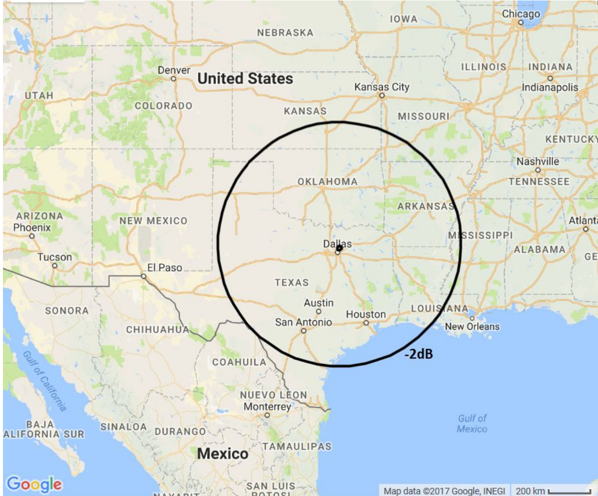
Figure 3: Orbital plane 3- Apogee 450Km
