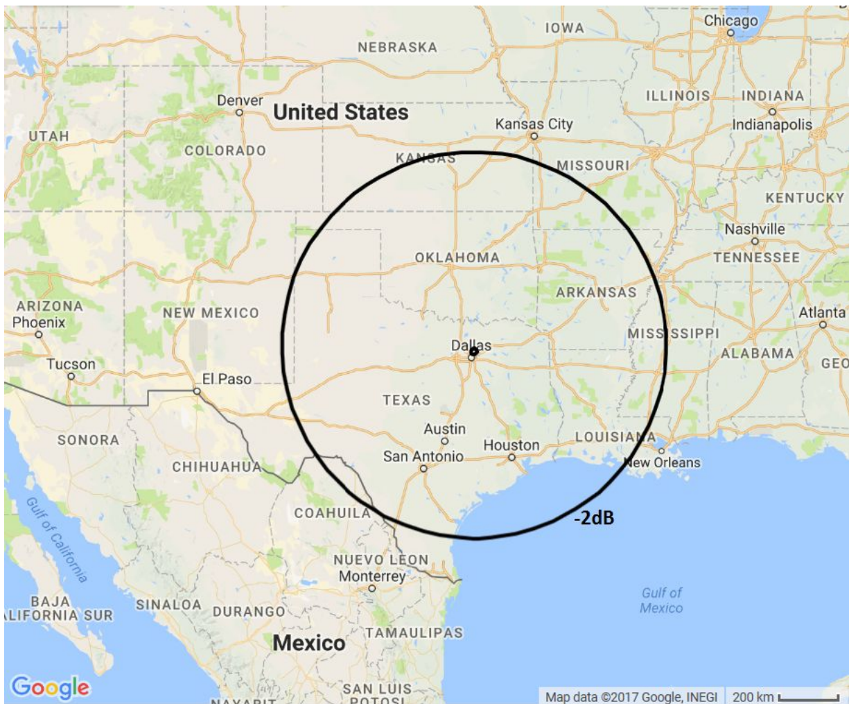
Figure 5: Orbital plane 5- Apogee 500Km
