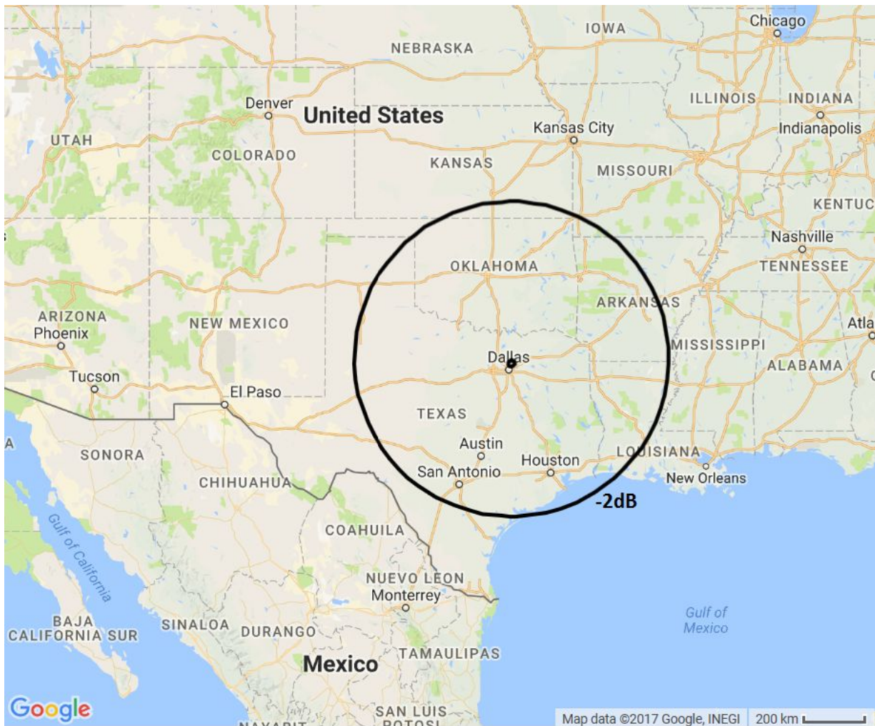
Figure 1: Orbital plane 1- Apogee 400Km
