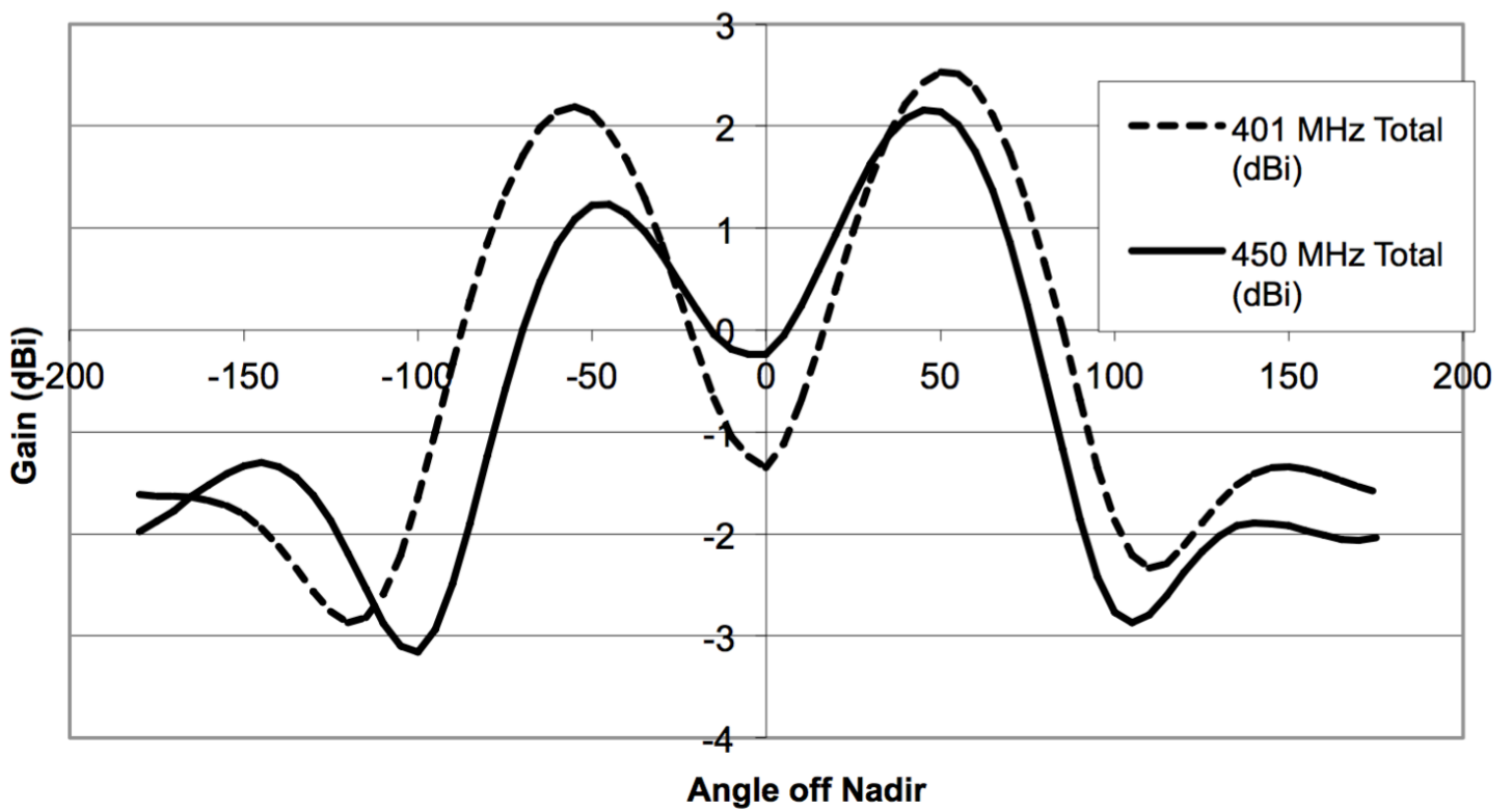
UHF Antenna - Horizontal Cut
