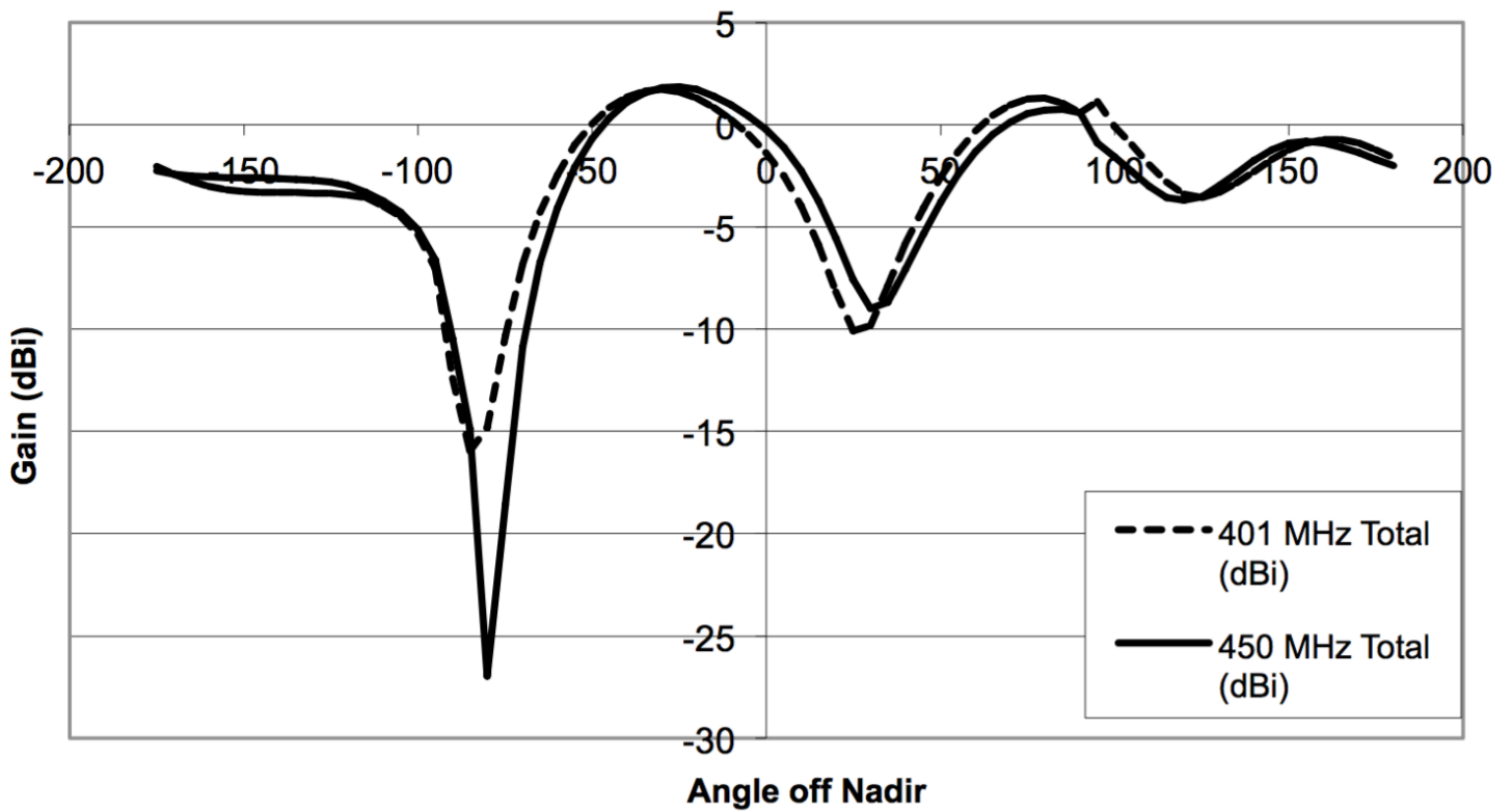
UHF Antenna - Vertical Cut
