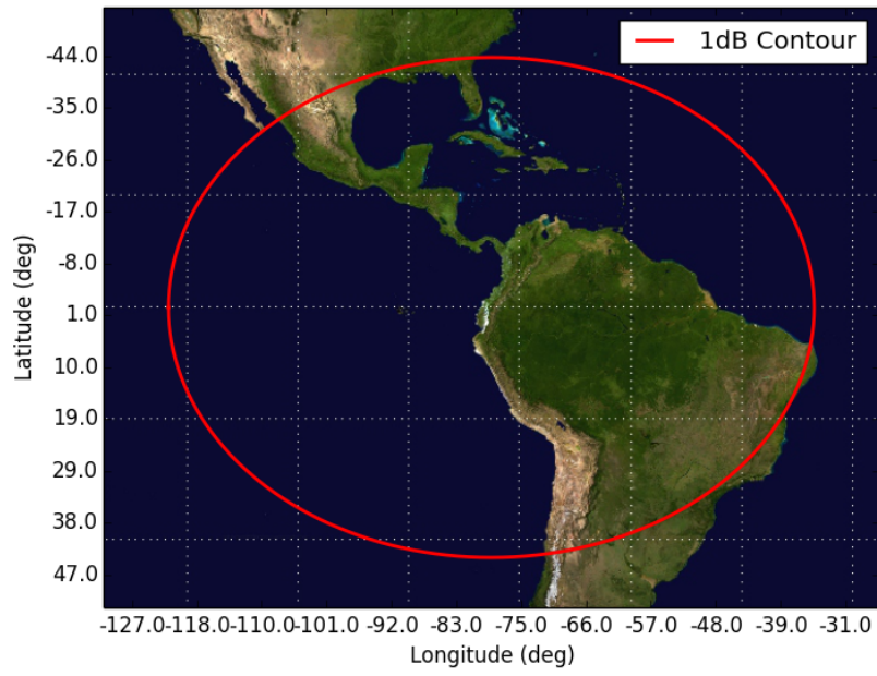
Figure 10: Orbit 10, Beam AIR1 AIR1 - Orbit 10 Apogee (500km)
