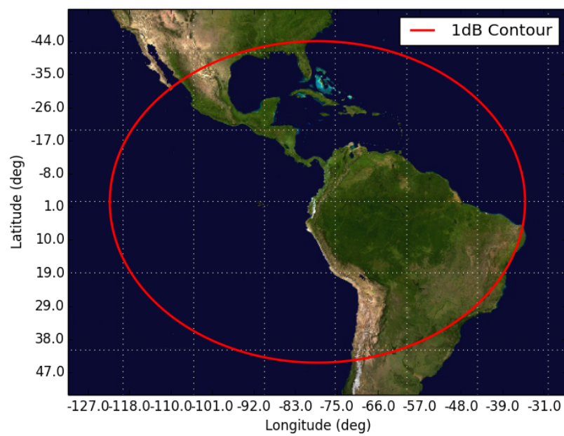
Figure 11: Orbit 11, Beam AIR4 AIR4 - Orbit 11 Apogee (575km)
