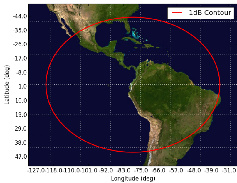
Figure 8: Orbit 8, Beam AIR4 AIR4 - Orbit 8 Apogee (450km)
