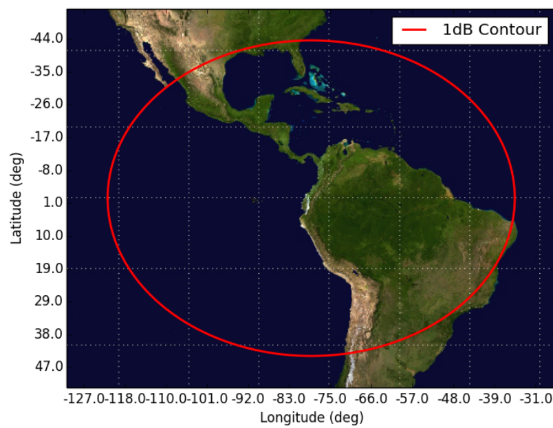
Figure 13: Orbit 13, Beam AIR4 AIR4 - Orbit 13 Apogee (450km)
