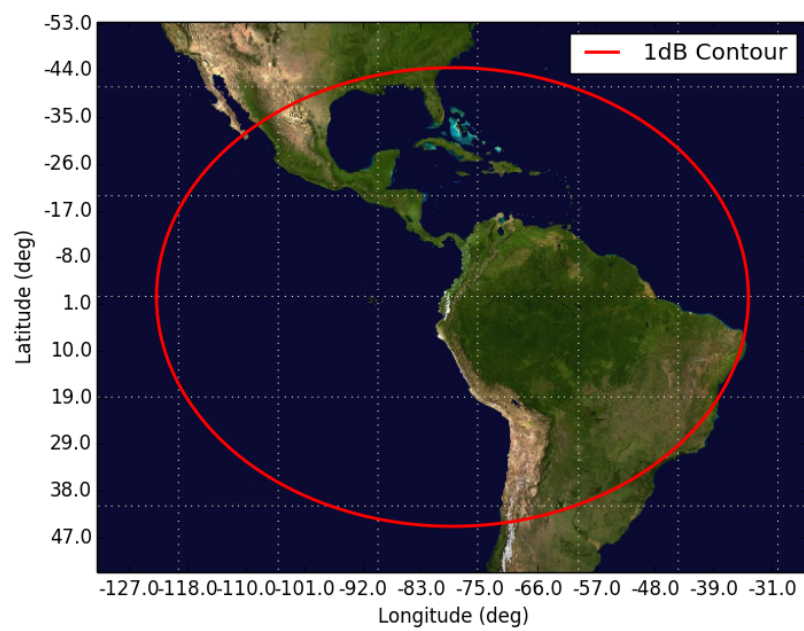
Figure 1: Orbit 1, Beam AIR4 AIR4 - Orbit 1 Apogee (720km)
