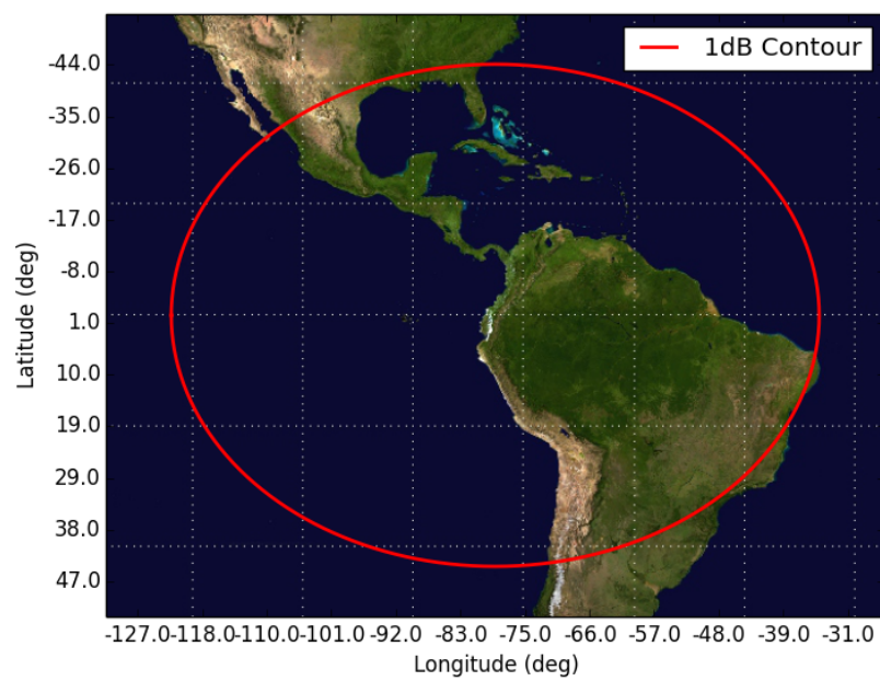
Figure 5: Orbit 5, Beam AIR4 AIR4 - Orbit 5 Apogee (600km)
