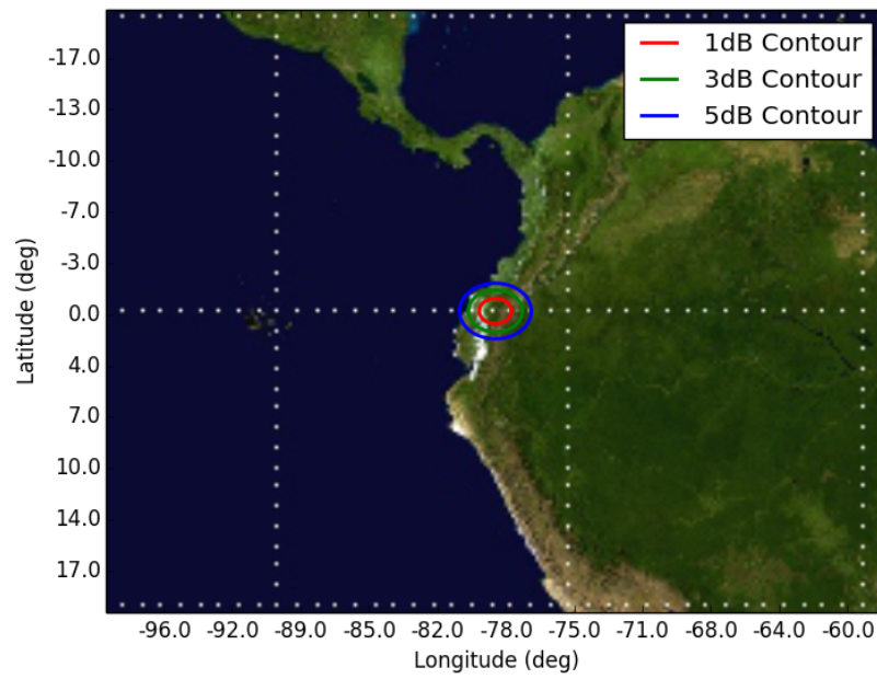
Figure 16: Orbit 16, Beam GAR4 GAR4 - Orbit 16 Apogee (400km)
