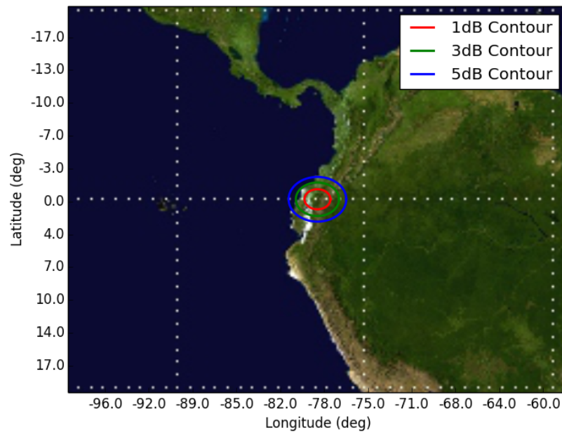
Figure 12: Orbit 12, Beam GAR4 GAR4 - Orbit 12 Apogee (500km)
