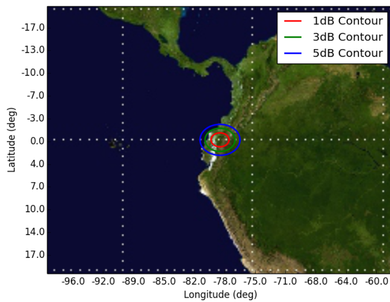
Figure 4: Orbit 4, Beam GAR4 GAR4 - Orbit 4 Apogee (500km)
