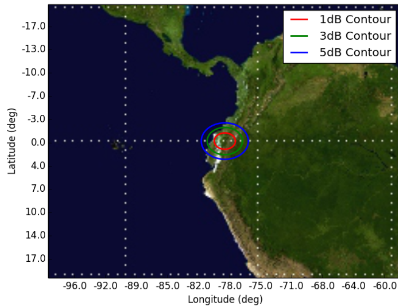
Figure 11: Orbit 11, Beam GAR4 GAR4 - Orbit 11 Apogee (575km)
