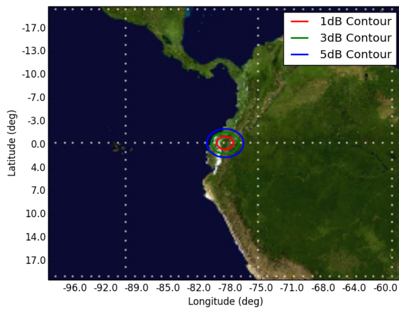
Figure 9: Orbit 9, Beam GAR4 GAR4 - Orbit 9 Apogee (450km)
