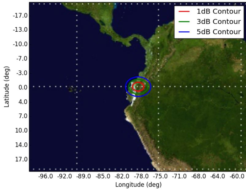
Figure 4: Orbit 4, Beam GLR3 GLR3 - Orbit 4 Apogee (500km)
