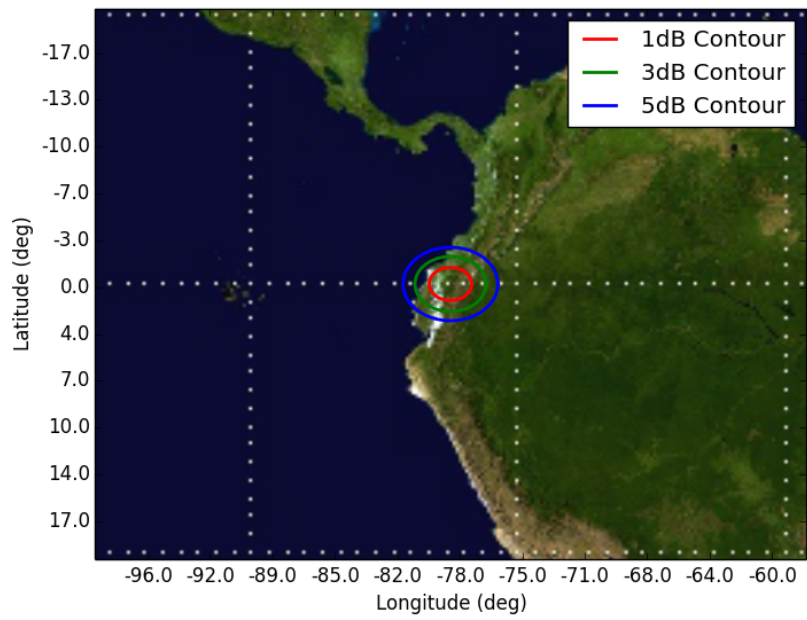
Figure 11: Orbit 11, Beam GLR3 GLR3 - Orbit 11 Apogee (575km)
