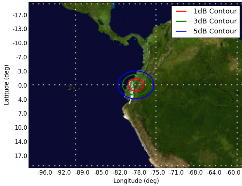
Figure 1: Orbit 1, Beam GLR3 GLR3 - Orbit 1 Apogee (720km)
