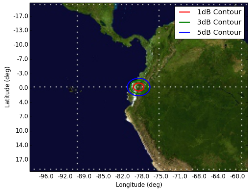
Figure 8: Orbit 8, Beam GLR3 GLR3 - Orbit 8 Apogee (450km)
