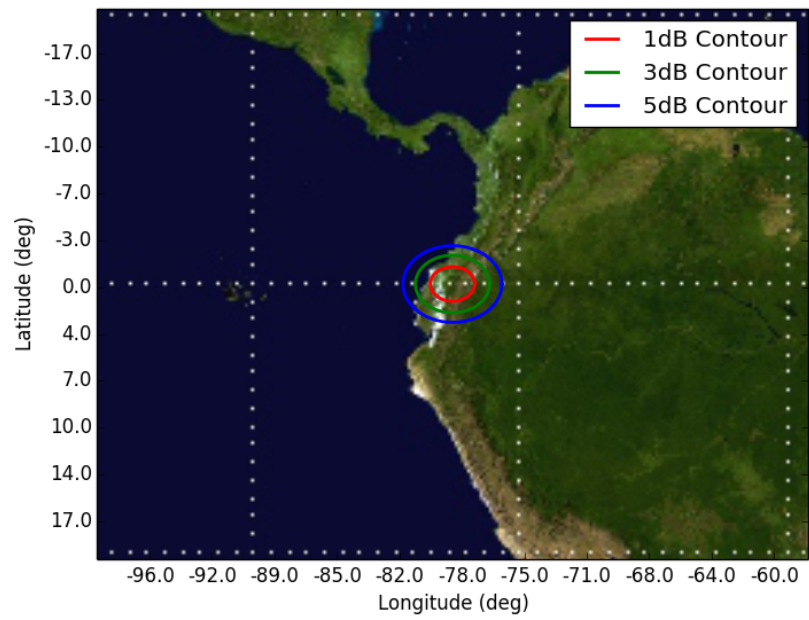
Figure 3: Orbit 3, Beam GLR3 GLR3 - Orbit 3 Apogee (600km)
