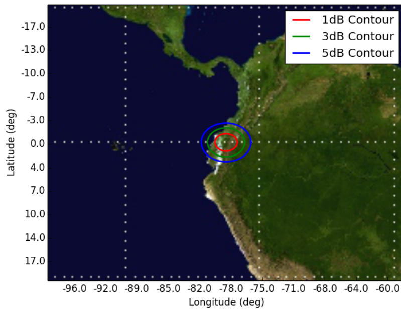
Figure 7: Orbit 7, Beam GLR3 GLR3 - Orbit 7 Apogee (600km)
