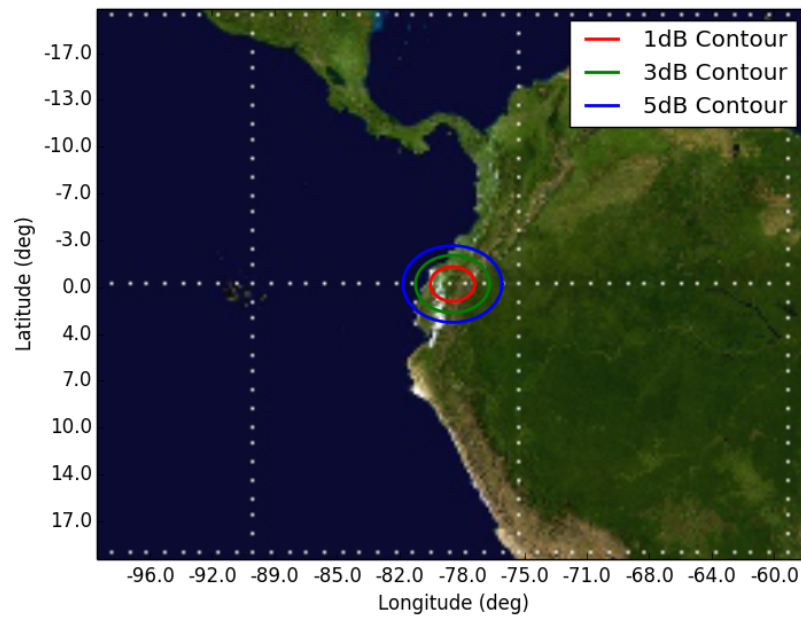
Figure 6: Orbit 6, Beam GPR1 GPR1 - Orbit 6 Apogee (600km)
