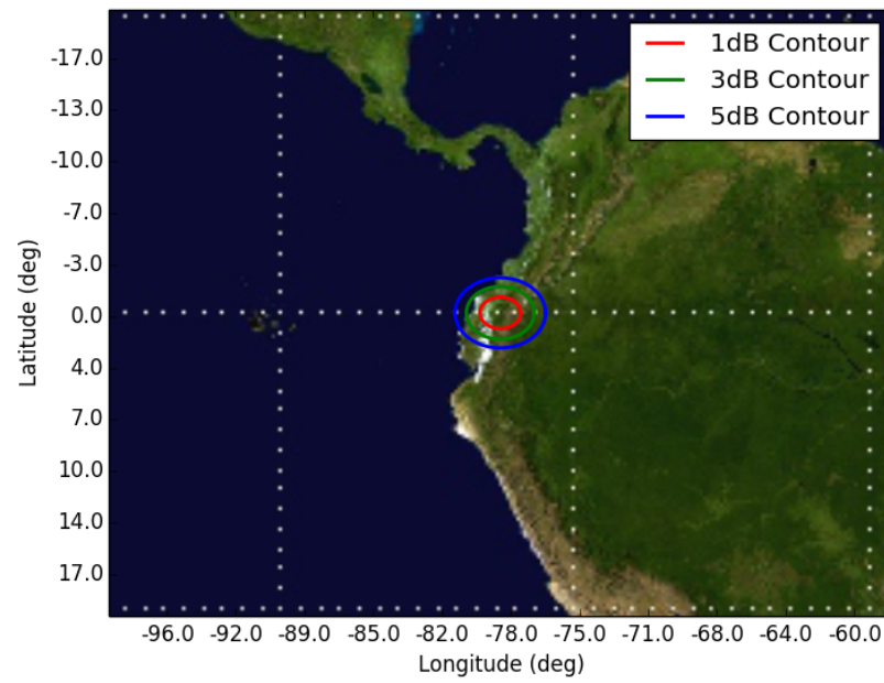
Figure 10: Orbit 10, Beam GPR1 GPR1 - Orbit 10 Apogee (500km)
