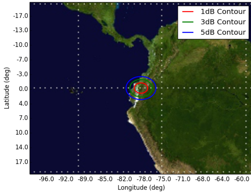
Figure 2: Orbit 2, Beam GPR4 GPR4 - Orbit 2 Apogee (580km)
