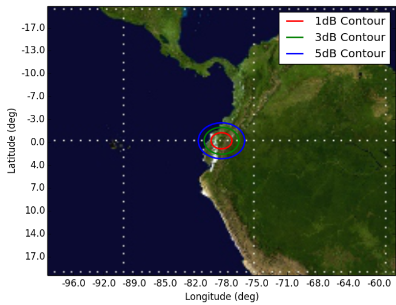
Figure 11: Orbit 11, Beam GPR4 GPR4 - Orbit 11 Apogee (575km)
