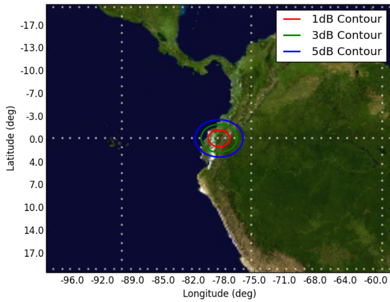
Figure 6: Orbit 6, Beam GPR4 GPR4 - Orbit 6 Apogee (600km)
