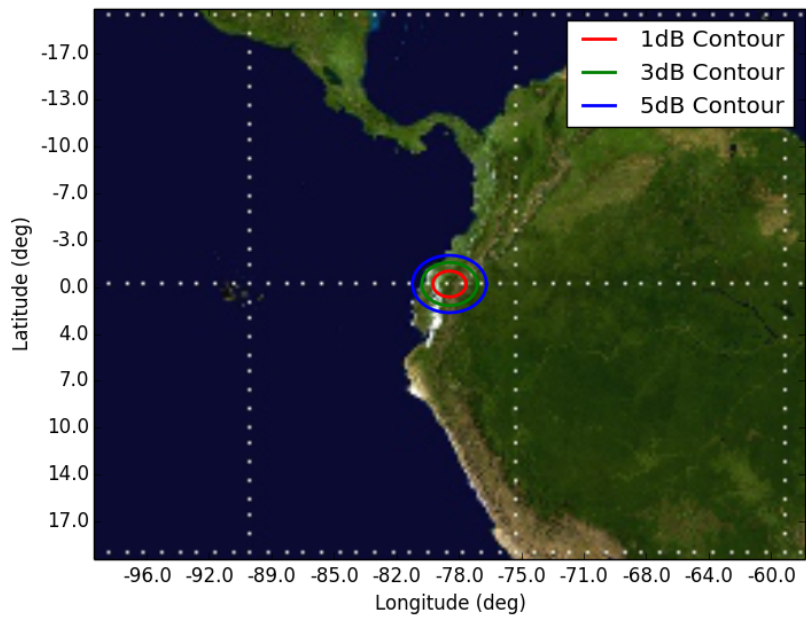
Figure 13: Orbit 13, Beam GPR4 GPR4 - Orbit 13 Apogee (450km)
