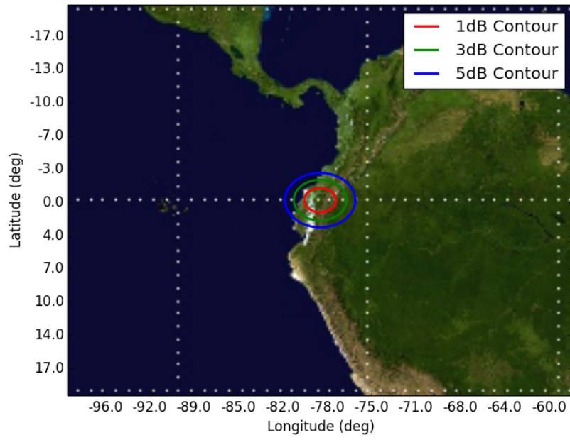
Figure 7: Orbit 7, Beam GPR4 GPR4 - Orbit 7 Apogee (600km)
