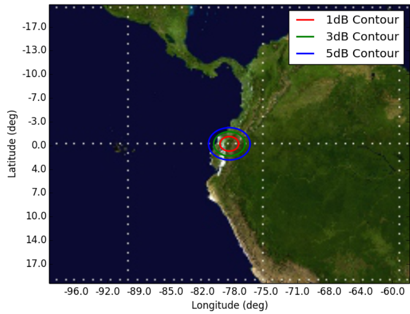
Figure 10: Orbit 10, Beam GPR4 GPR4 - Orbit 10 Apogee (500km)
