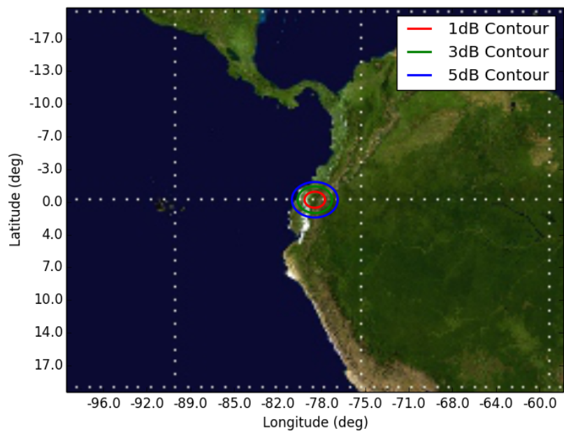
Figure 16: Orbit 16, Beam GPR4 GPR4 - Orbit 16 Apogee (400km)
