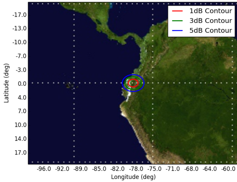
Figure 9: Orbit 9, Beam GPR4 GPR4 - Orbit 9 Apogee (450km)
