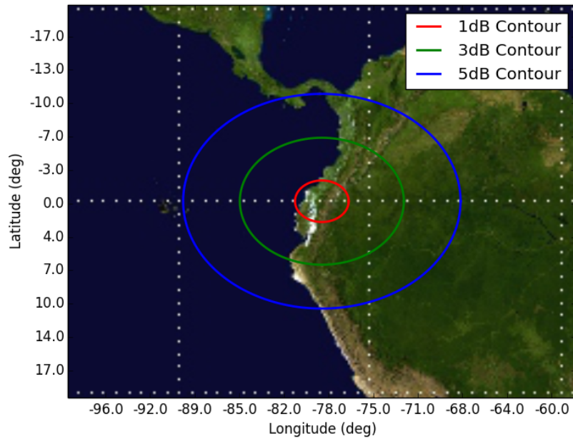
Figure 15: Orbit 15, Beam SD2 SD2 - Orbit 15 Apogee (500km)
