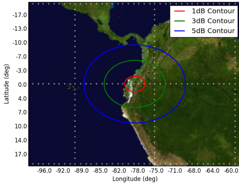
Figure 9: Orbit 9, Beam SD2 SD2 - Orbit 9 Apogee (450km)
