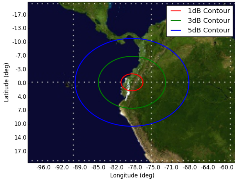
Figure 10: Orbit 10, Beam SD2 SD2 - Orbit 10 Apogee (500km)
