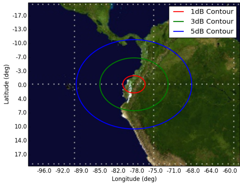
Figure 12: Orbit 12, Beam SD2 SD2 - Orbit 12 Apogee (500km)
