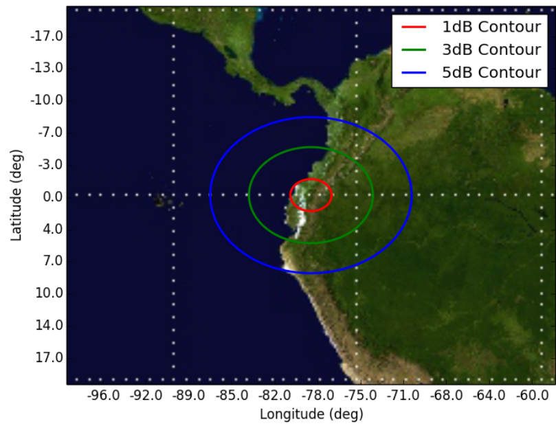
Figure 16: Orbit 16, Beam SD2 SD2 - Orbit 16 Apogee (400km)
