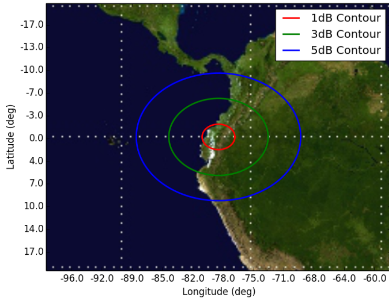
Figure 13: Orbit 13, Beam SD2 SD2 - Orbit 13 Apogee (450km)
