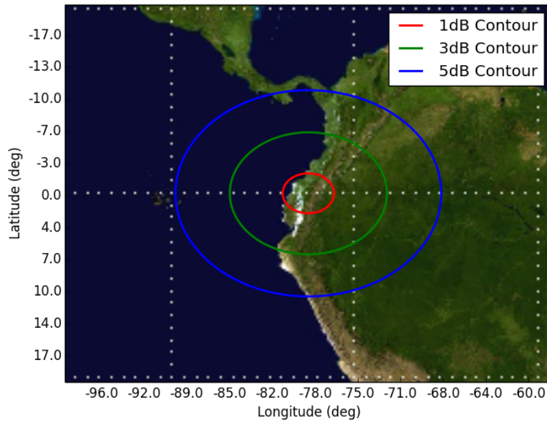
Figure 4: Orbit 4, Beam SD2 SD2 - Orbit 4 Apogee (500km)
