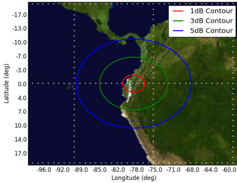
Figure 14: Orbit 14, Beam SD2 SD2 - Orbit 14 Apogee (500km)
