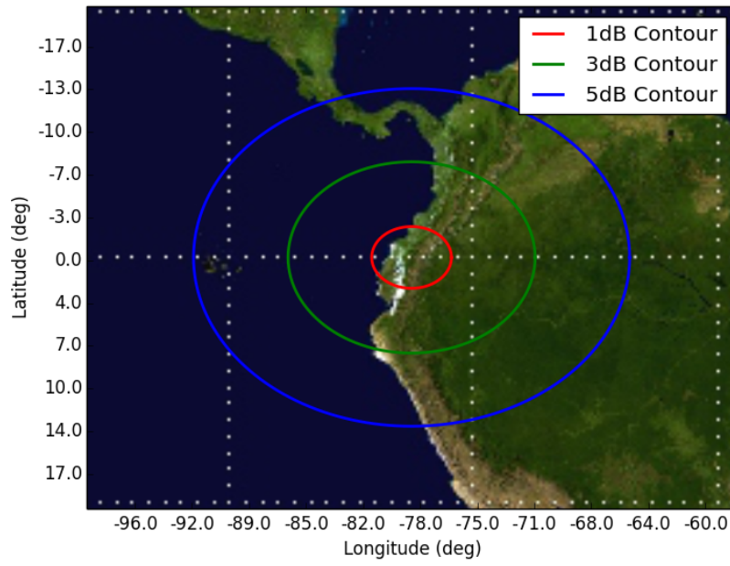
Figure 2: Orbit 2, Beam SD2 SD2 - Orbit 2 Apogee (580km)
