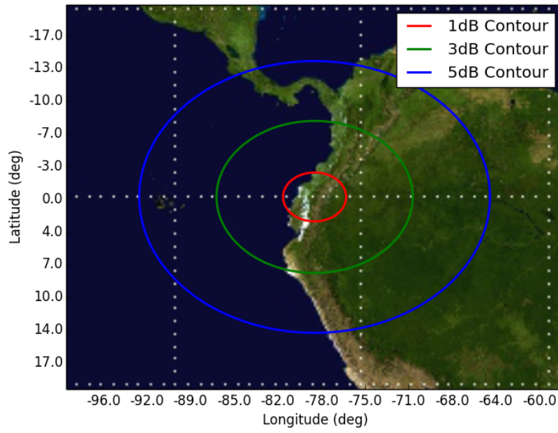
Figure 6: Orbit 6, Beam SD2 SD2 - Orbit 6 Apogee (600km)
