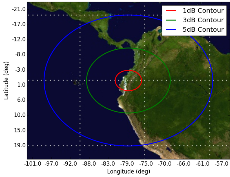
Figure 1: Orbit 1, Beam SD2 SD2 - Orbit 1 Apogee (720km)
