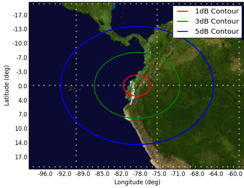
Figure 7: Orbit 7, Beam SD2 SD2 - Orbit 7 Apogee (600km)
