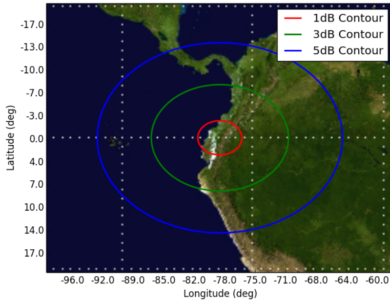
Figure 3: Orbit 3, Beam SD2 SD2 - Orbit 3 Apogee (600km)
