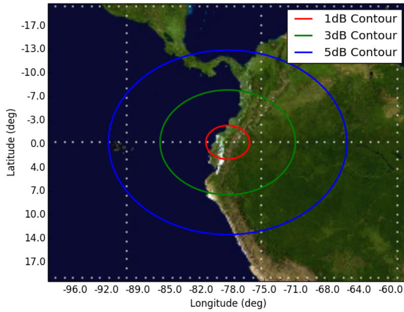
Figure 11: Orbit 11, Beam SD2 SD2 - Orbit 11 Apogee (575km)
