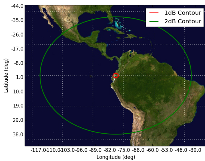
Figure 8: Orbit 8, Beam UD2B UD2B - Orbit 8 Apogee (450km)
