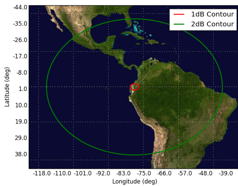
Figure 7: Orbit 7, Beam UD2B UD2B - Orbit 7 Apogee (600km)
