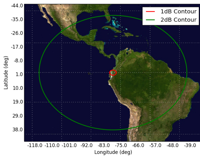
Figure 2: Orbit 2, Beam UD2B UD2B - Orbit 2 Apogee (580km)
