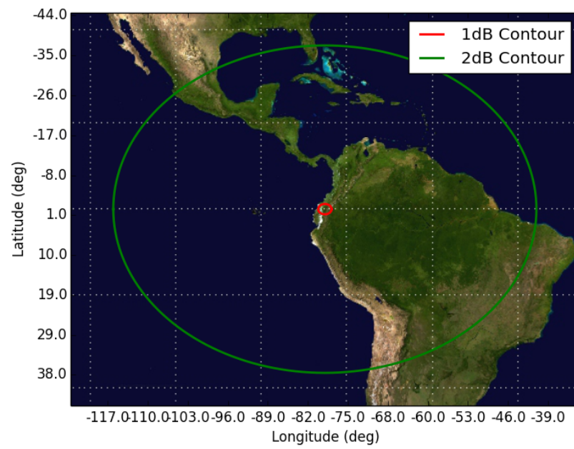
Figure 16: Orbit 16, Beam UD2B UD2B - Orbit 16 Apogee (400km)
