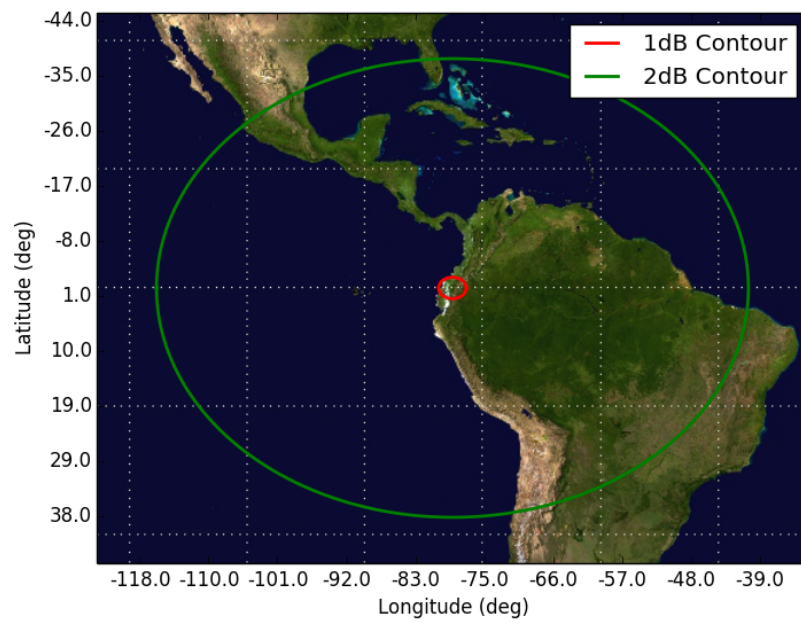
Figure 3: Orbit 3, Beam UD2B UD2B - Orbit 3 Apogee (600km)
