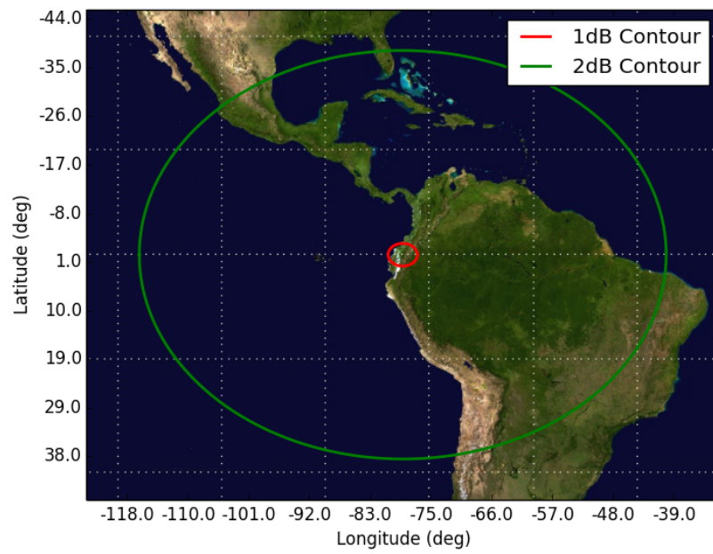
Figure 1: Orbit 1, Beam UD2B UD2B - Orbit 1 Apogee (720km)
