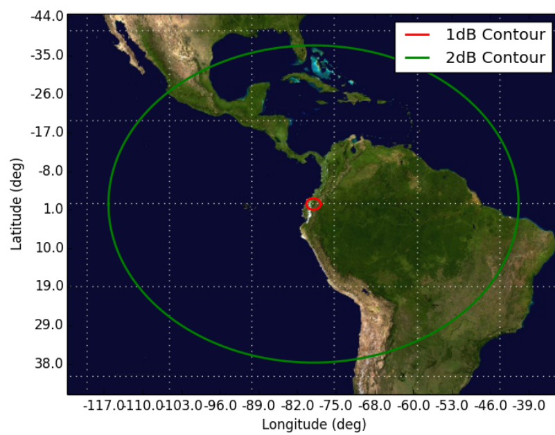
Figure 9: Orbit 9, Beam UD2B UD2B - Orbit 9 Apogee (450km)
