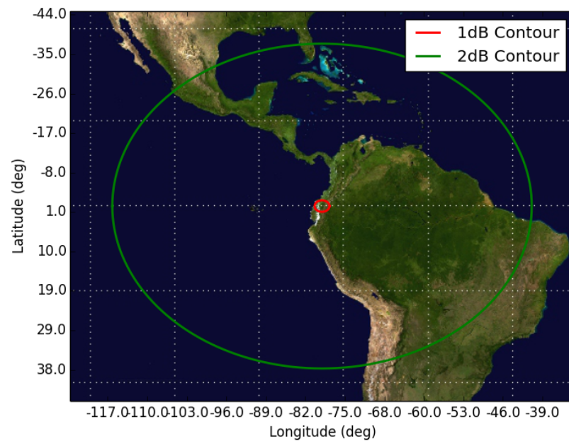
Figure 13: Orbit 13, Beam UD2B UD2B - Orbit 13 Apogee (450km)
