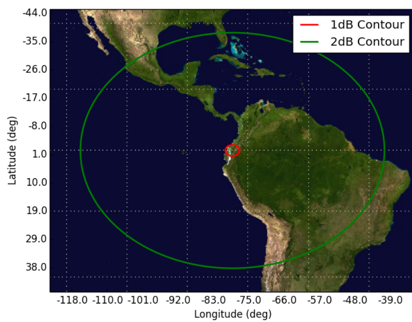
Figure 6: Orbit 6, Beam UD2B UD2B - Orbit 6 Apogee (600km)
