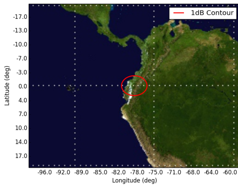
Figure 10: Orbit 10, Beam UD2P UD2P - Orbit 10 Apogee (500km)
