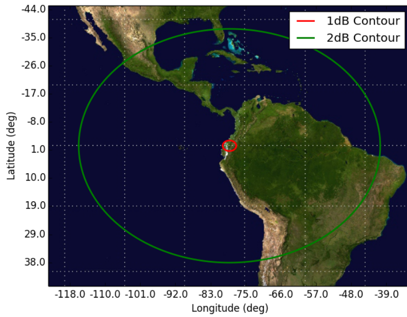
Figure 2: Orbit 2, Beam UD3B UD3B - Orbit 2 Apogee (580km)
