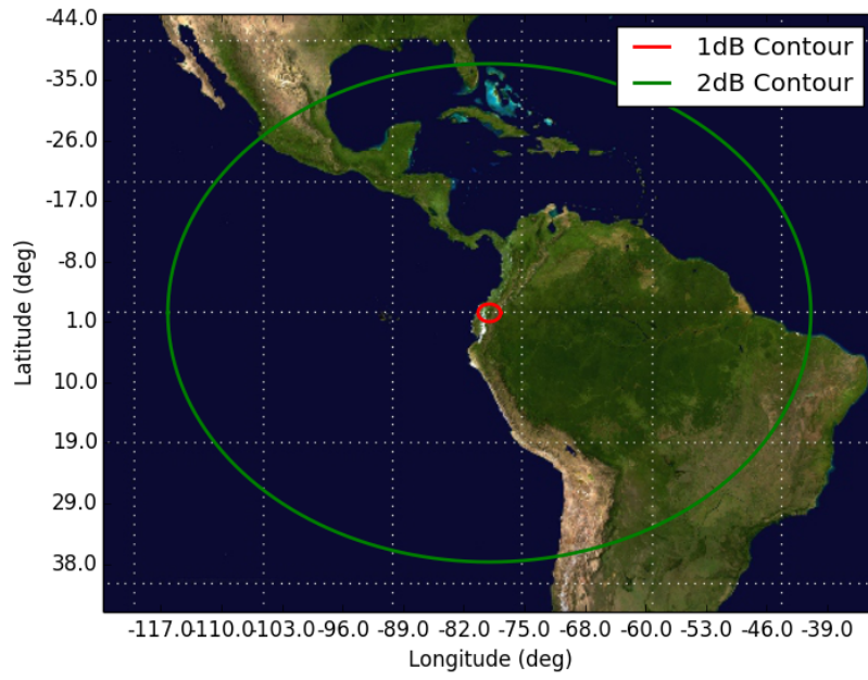
Figure 8: Orbit 8, Beam UD3B UD3B - Orbit 8 Apogee (450km)
