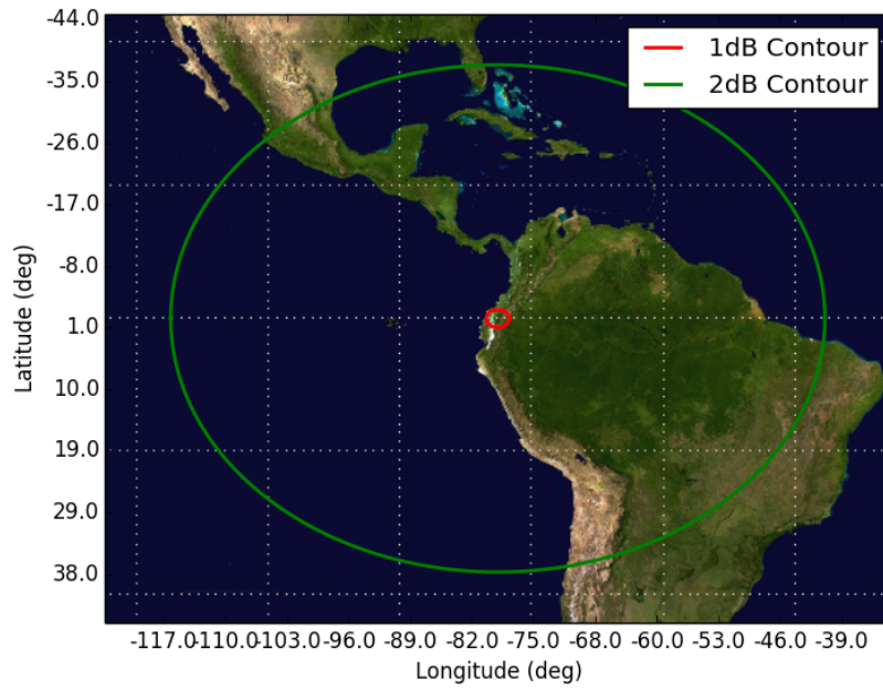
Figure 9: Orbit 9, Beam UD3B UD3B - Orbit 9 Apogee (450km)
