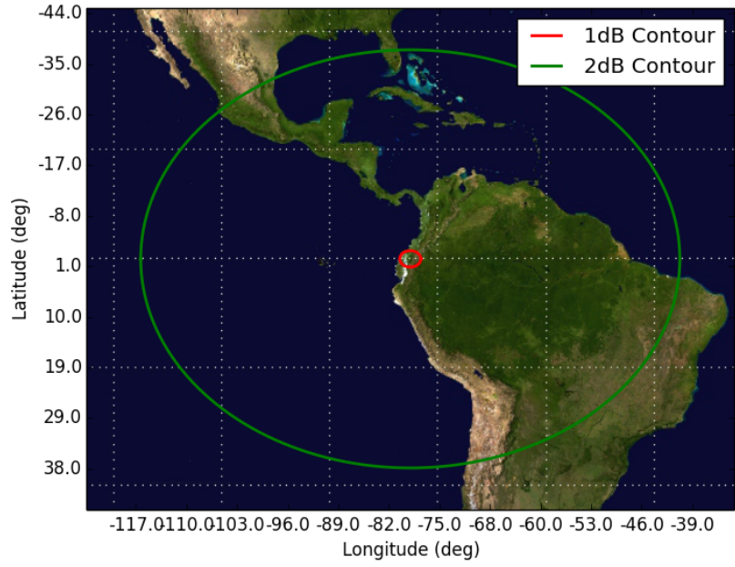
Figure 15: Orbit 15, Beam UD3B UD3B - Orbit 15 Apogee (500km)
