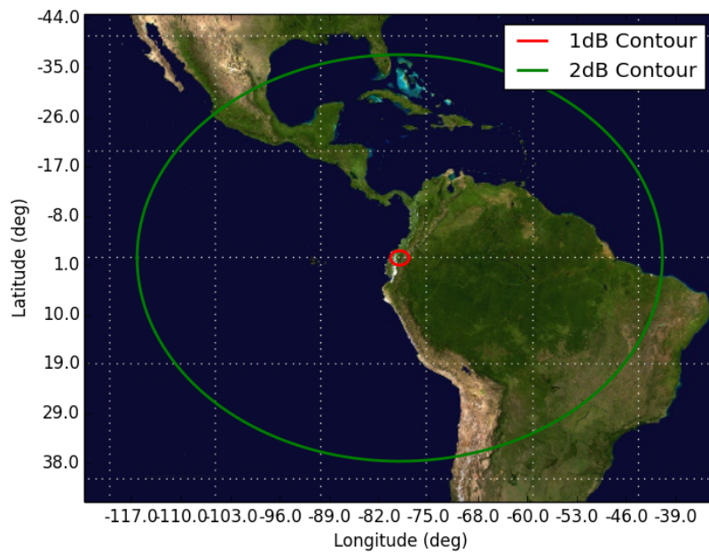
Figure 13: Orbit 13, Beam UD3B UD3B - Orbit 13 Apogee (450km)
