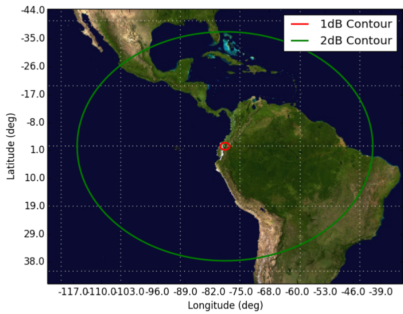
Figure 16: Orbit 16, Beam UU3B UU3B - Orbit 16 Apogee (400km)
