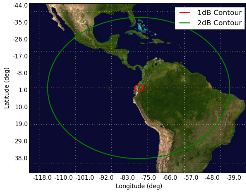
Figure 2: Orbit 2, Beam UU3B UU3B - Orbit 2 Apogee (580km)
