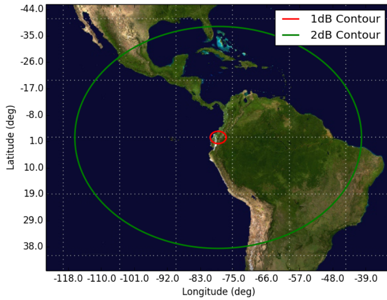
Figure 1: Orbit 1, Beam UU3B UU3B - Orbit 1 Apogee (720km)
