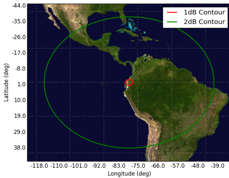
Figure 11: Orbit 11, Beam UU3B UU3B - Orbit 11 Apogee (575km)
