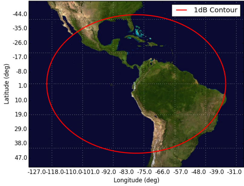
Figure 12: Orbit 12, Beam ASM1 ASM1 - Orbit 12 Apogee (500km)
