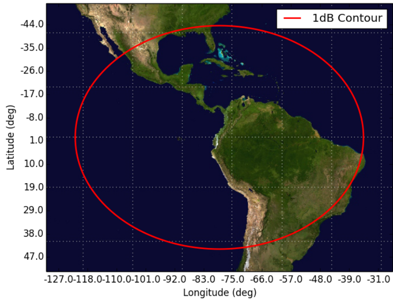
Figure 9: Orbit 9, Beam ASM1 ASM1 - Orbit 9 Apogee (450km)
