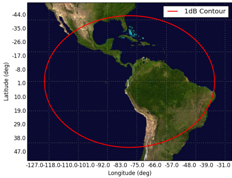
Figure 8: Orbit 8, Beam ASM1 ASM1 - Orbit 8 Apogee (450km)
