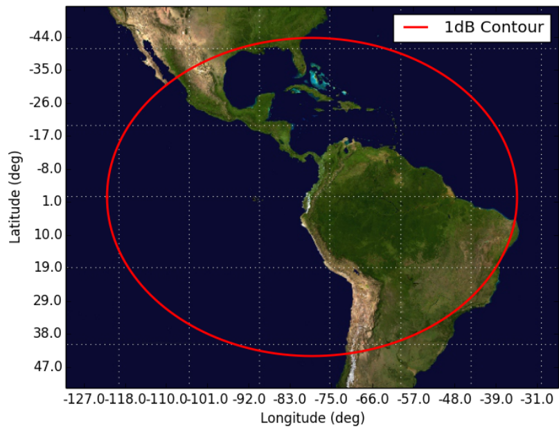
Figure 15: Orbit 15, Beam ASM1 ASM1 - Orbit 15 Apogee (500km)
