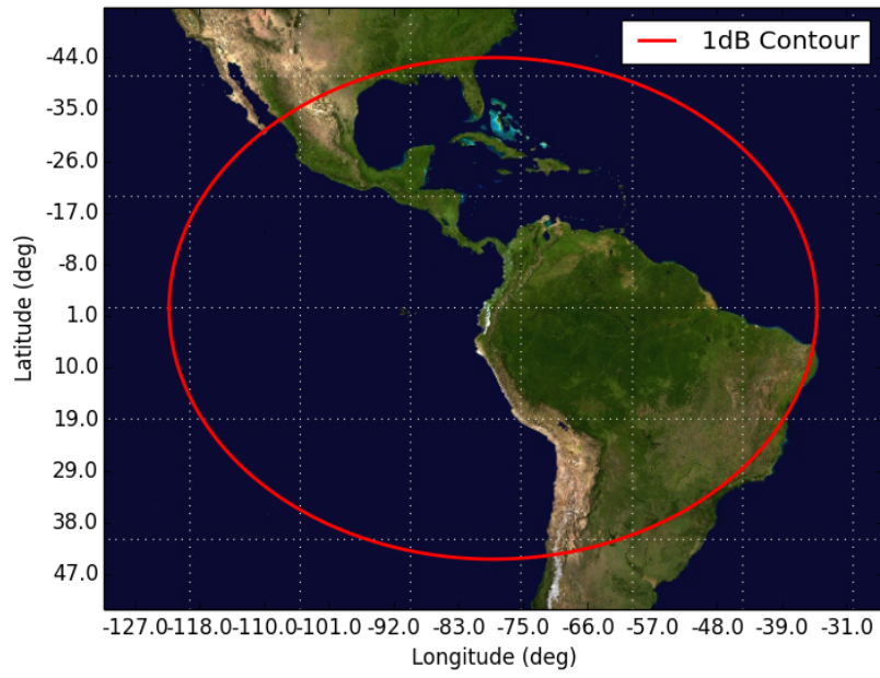
Figure 2: Orbit 2, Beam ASM1 ASM1 - Orbit 2 Apogee (580km)
