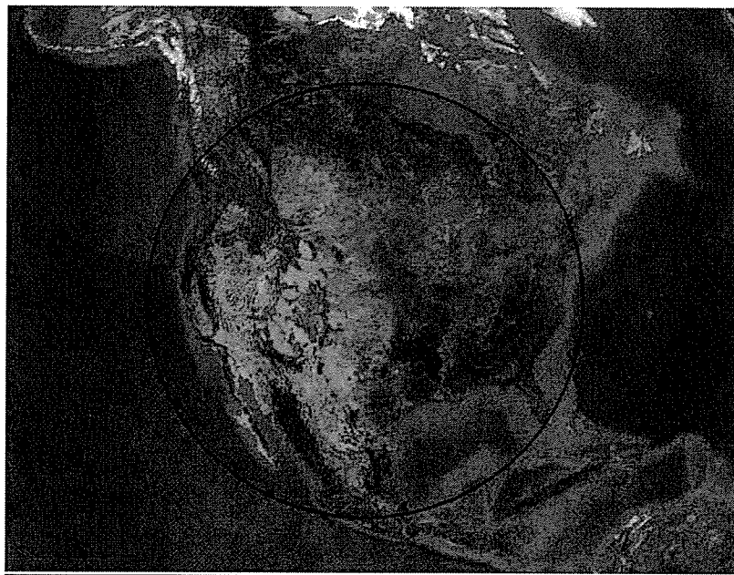
Figure 1 Representative Single OG2 Satellite Footprint Altitude = 715 km, User Minimum Elevation Angle Mask = 5°
