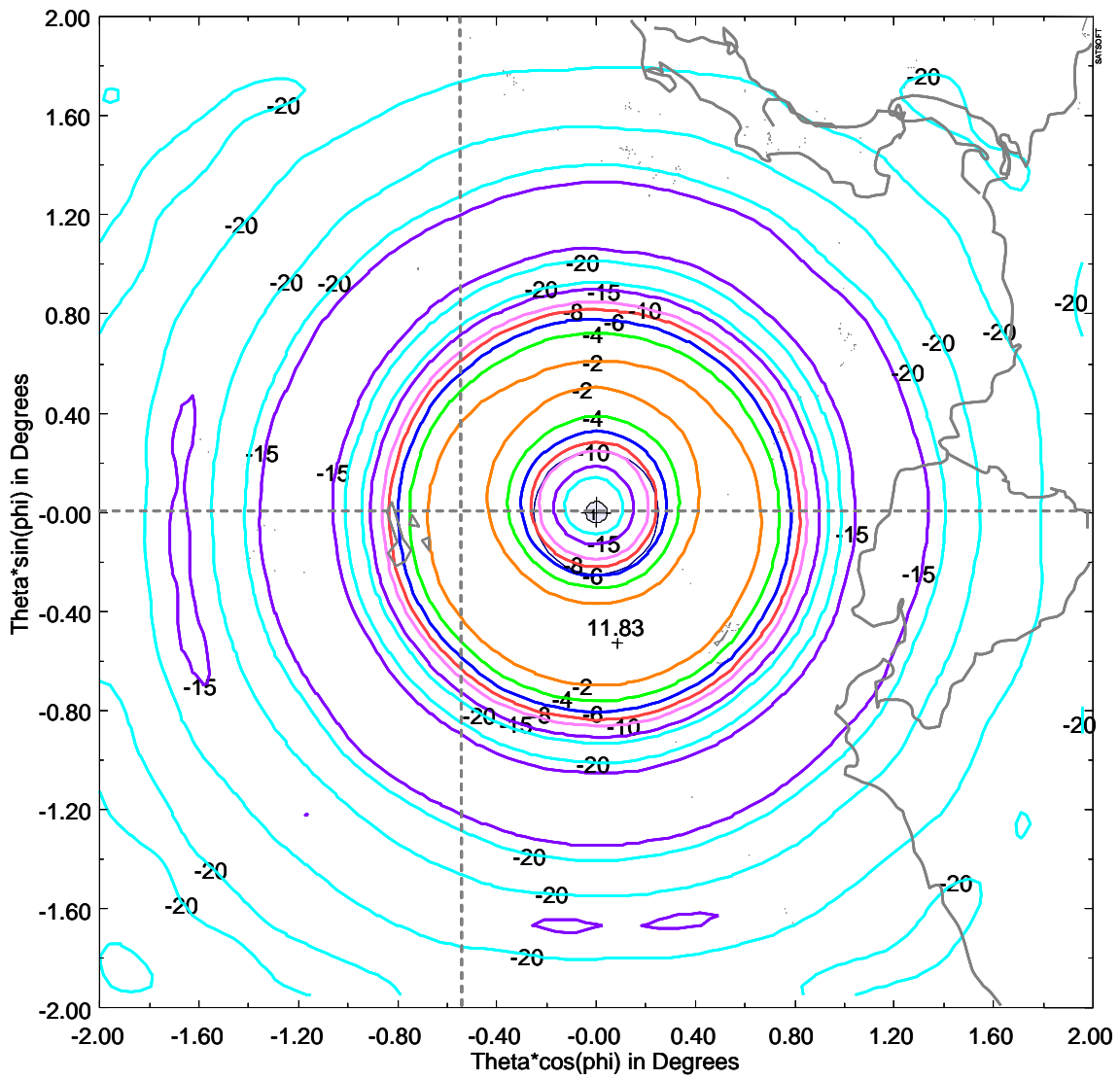
GSO Satellite at 87W Transmit Antenna Contours – XPol (Contour Levels: -2, -4, -6, -8, -10, -15, -20 dB)
