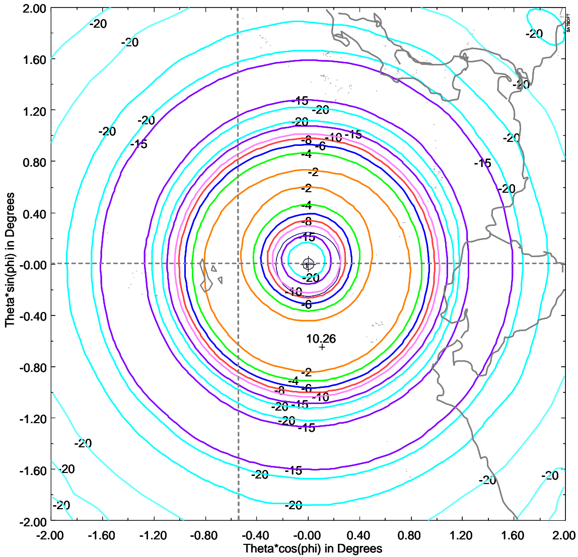
GSO Satellite at 87W Receive Antenna Contours – XPol (Contour Levels: -2, -4, -6, -8, -10, -15, -20 dB)
