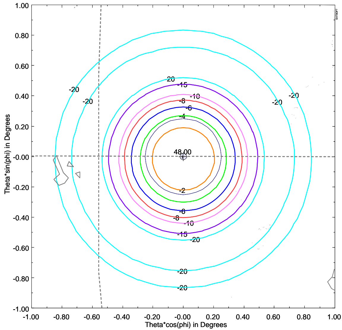
GSO Satellite at 87W Transmit Antenna Contours – CoPol (Contour Levels: -2, -4, -6, -8, -10, -15, -20 dB)
