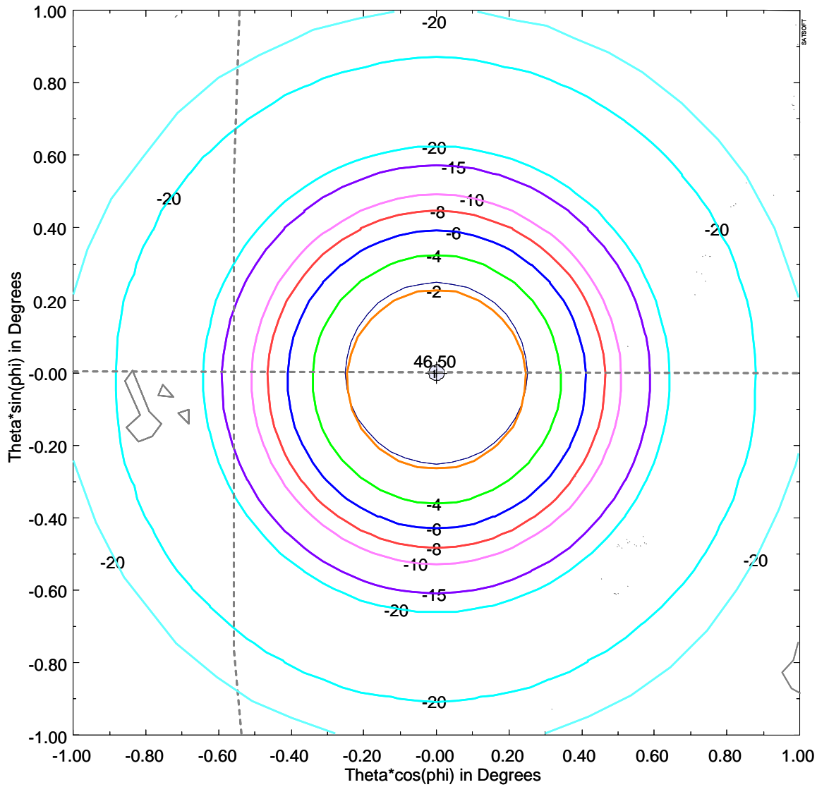
Figure C3: Receive Antenna Contours (Copol)
