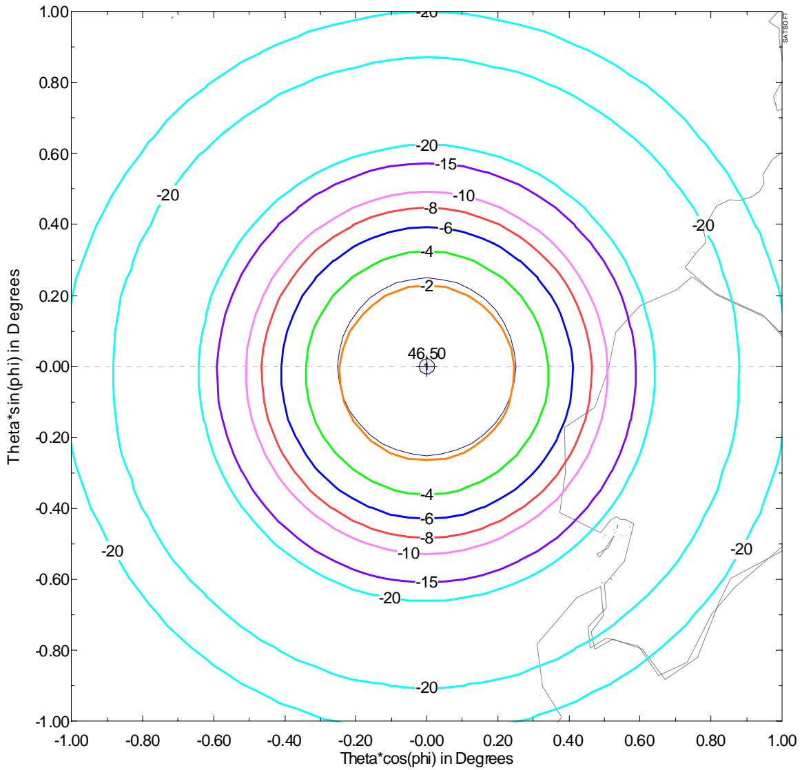
GSO Satellite at 83W Receive Antenna Contours – CoPol (Contour Levels: -2, -4, -6, -8, -10, -15, - 20 dB)
