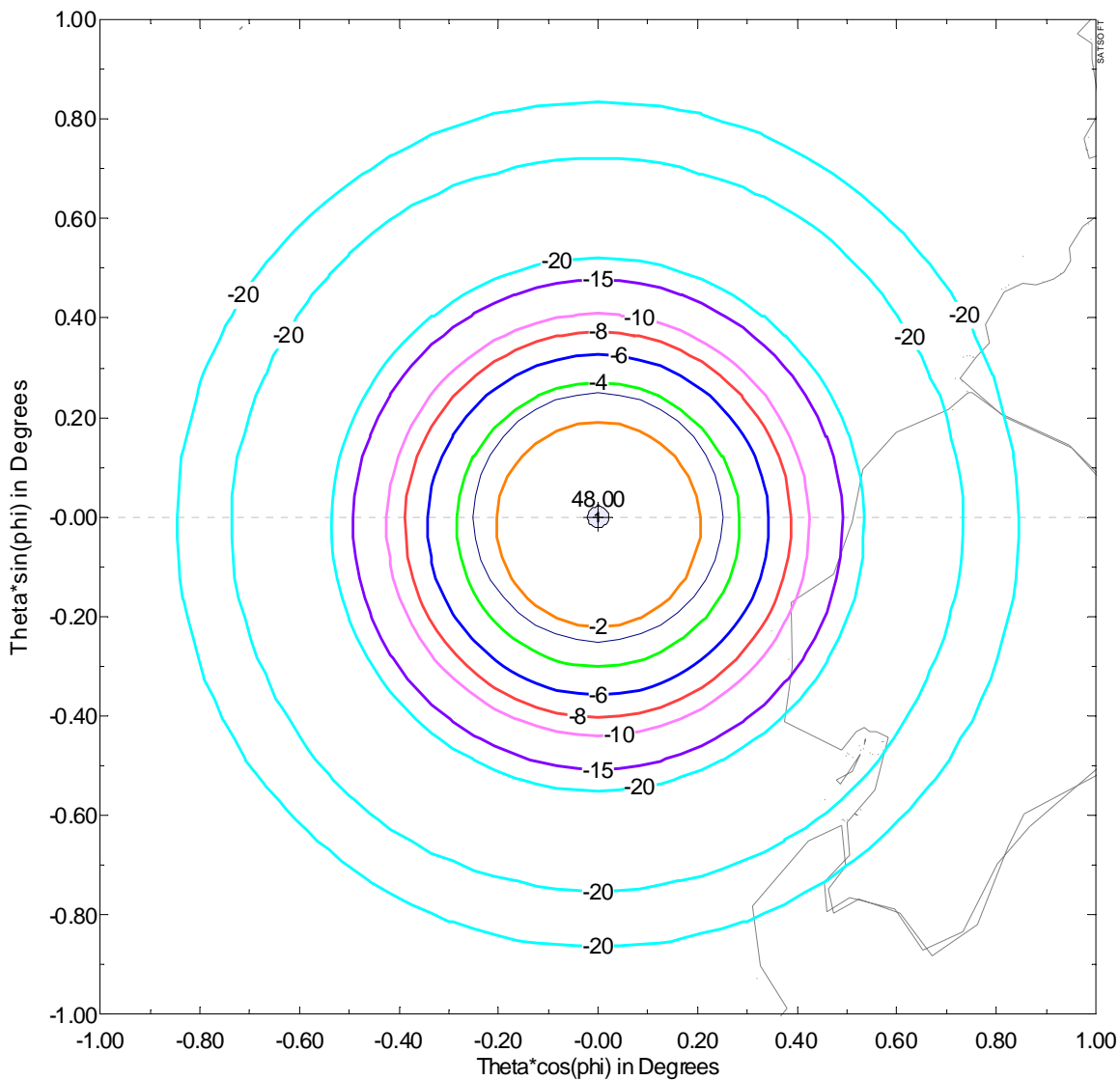
GSO Satellite at 83W Transmit Antenna Contours – CoPol (Contour Levels: -2, -4, -6, -8, -10, -15, - 20 dB)
