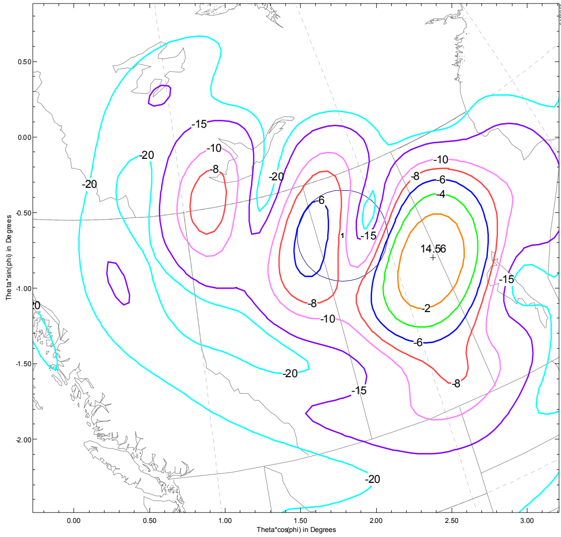
HEO 30 GHz Rx Antenna Beam XPol
