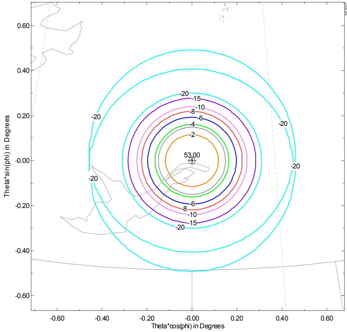
HEO 40 GHz Tx Antenna Beam - CoPol
