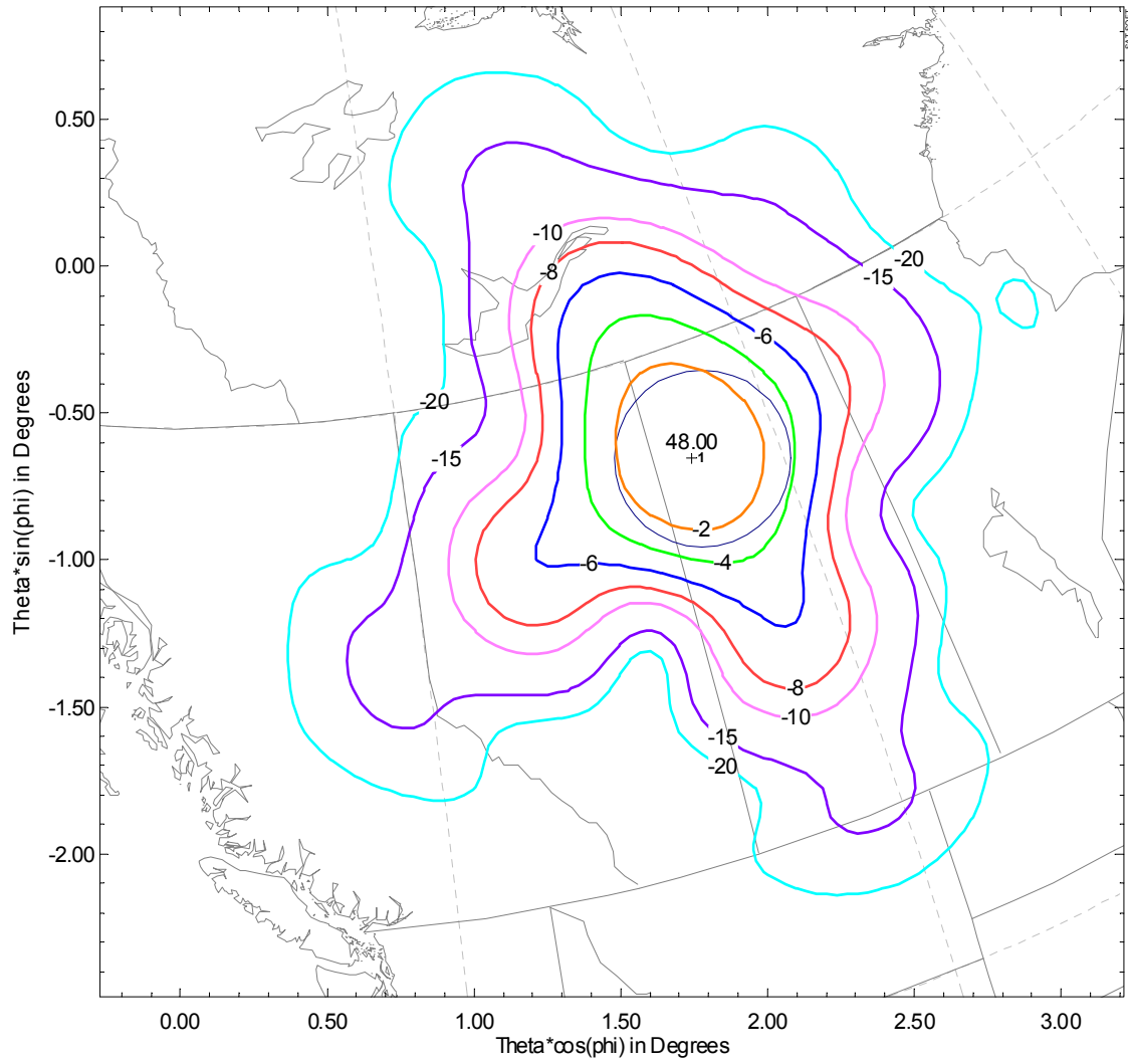
HEO 20 GHz Tx Antenna Beam CoPol
