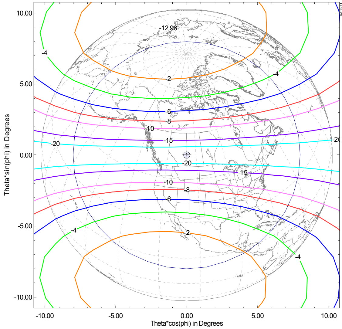
HEO 20 GHz Tx Beacon Antenna Beam - XPol
