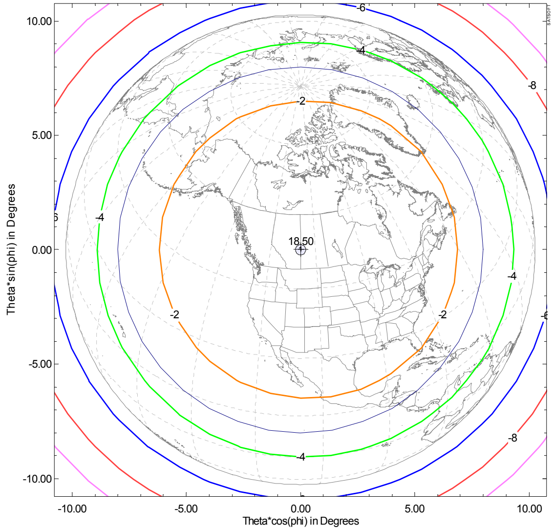
HEO 20 GHz Tx Beacon Antenna Beam - CoPol
