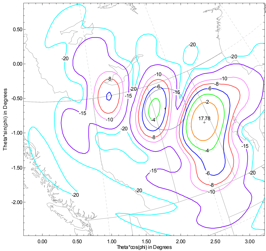
HEO 20 GHz Tx Antenna Beam XPol
