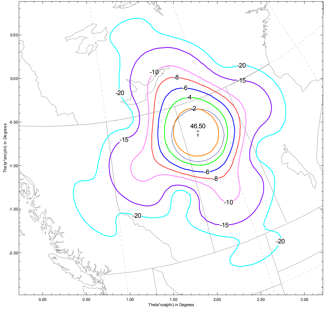
HEO 30 GHz Rx Antenna Beam CoPol
