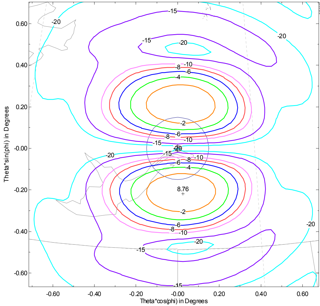
HEO 50 GHz Rx Antenna Beam - XPol
