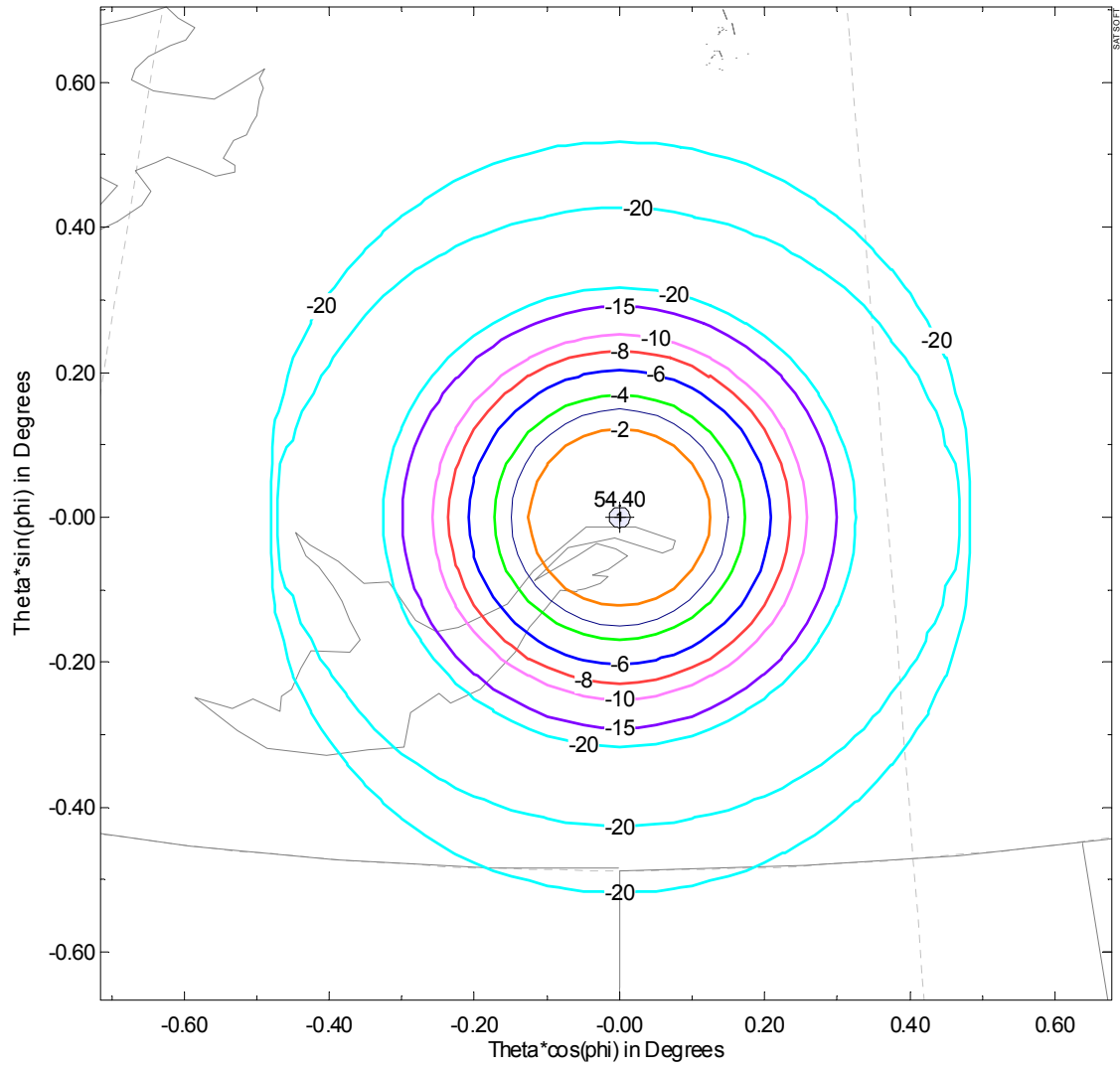
HEO 50 GHz Rx Antenna Beam CoPol
