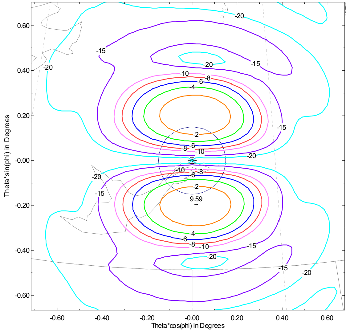
HEO 40 GHz Tx Antenna Beam - XPol
