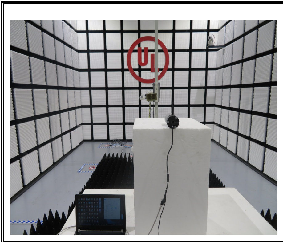
RADIATED RF MEASUREMENT SETUP (ABOVE 1 GHz)
