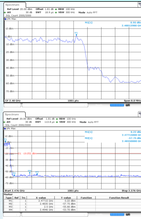
Hopping mode
