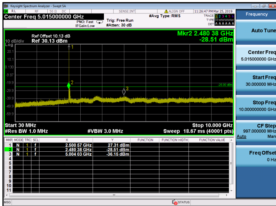
LTE Band 41 / 5MHz / 16QAM - RB Size/Offset (1/14) – Low Channel
