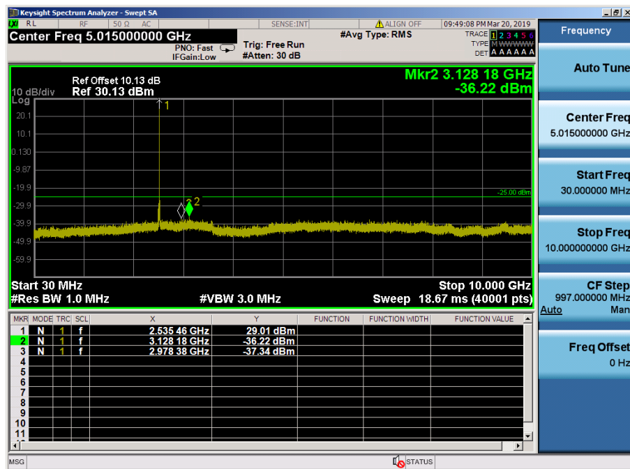
LTE Band 7 / 5MHz / 16QAM - RB Size/Offset (1/12) – Mid Channel
