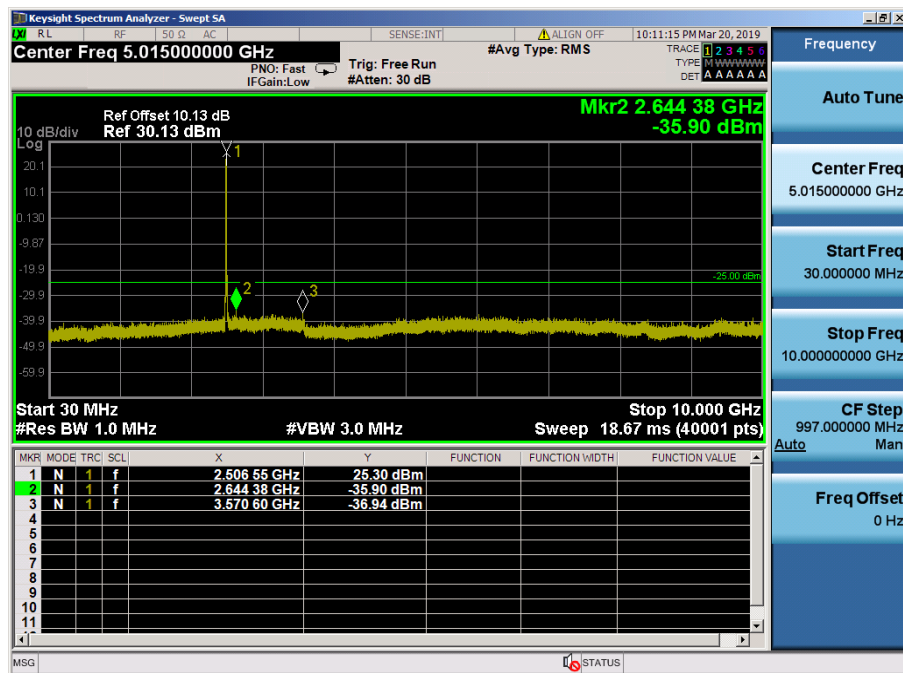
LTE Band 7 / 10MHz / 16QAM - RB Size/Offset (25/12) – Low Channel
