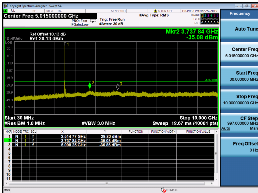
LTE Band 41 / 20MHz / QPSK - RB Size/Offset (1/99) – Low Channel
