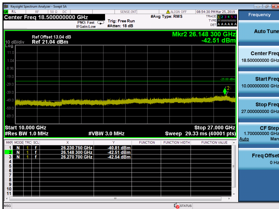
LTE Band 41 / 5MHz / QPSK - RB Size/Offset (1/24) – High Channel
