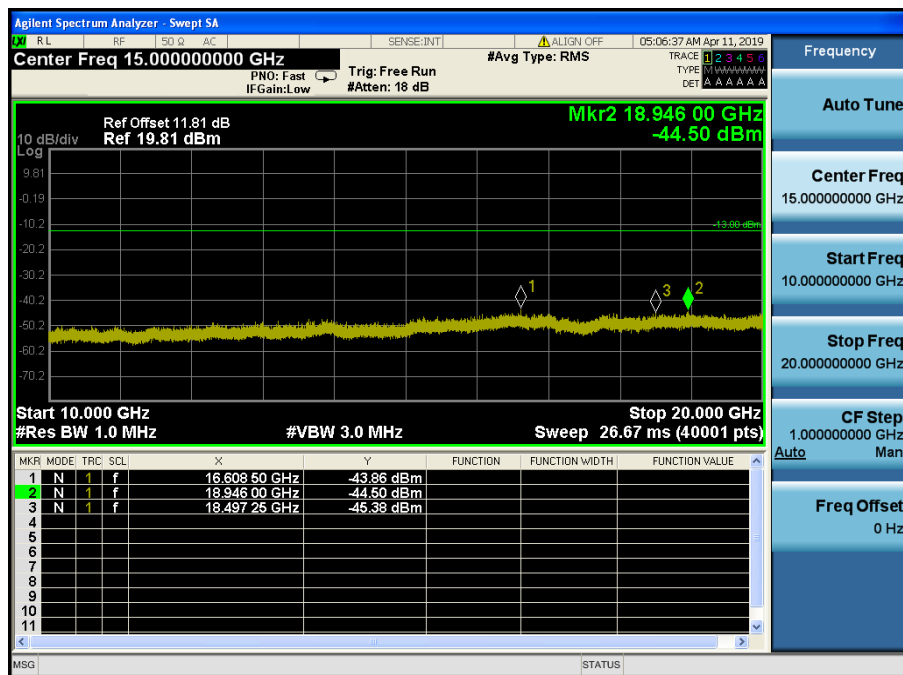
LTE Band 2 / 5MHz / 64QAM - RB Size/Offset (1/0) – Low Channel
