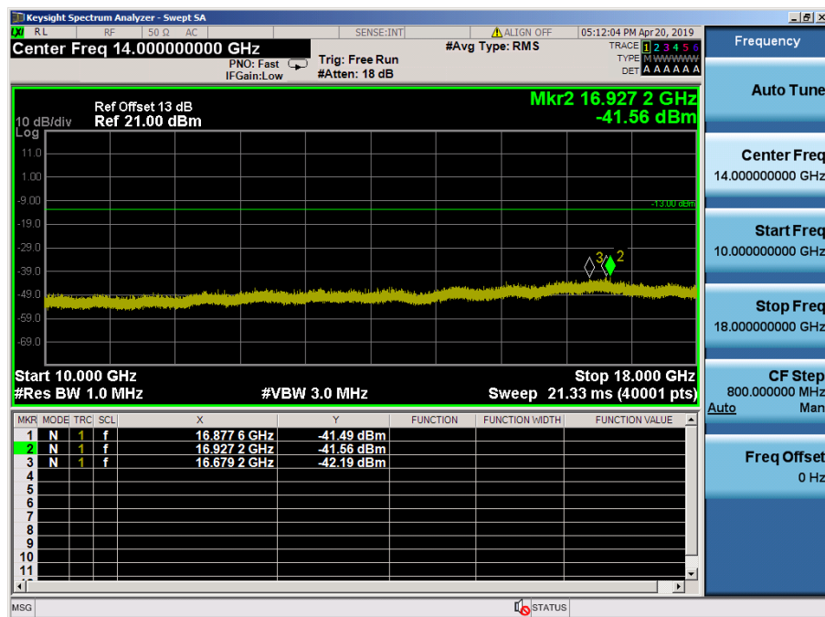
LTE Band 66, 4 / 1.4MHz / 16QAM - RB Size/Offset (3/0) – Low Channel
