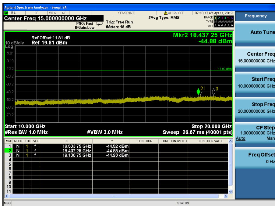
LTE Band 2 / 20MHz / 64QAM - RB Size/Offset (1/0)–Mid Channel
