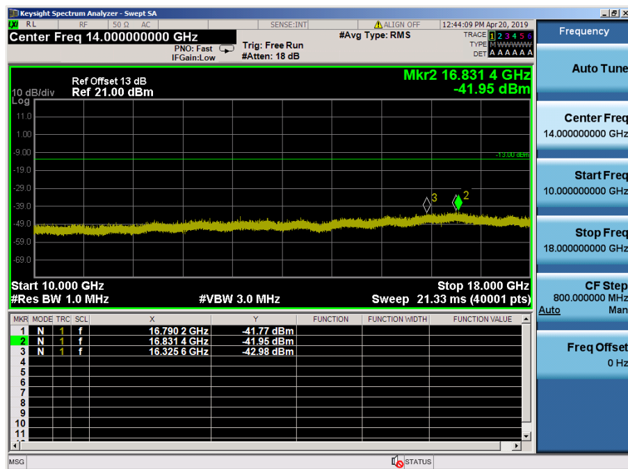
LTE Band 66, 4 / 1.4MHz / QPSK - RB Size/Offset (3/3) – High Channel
