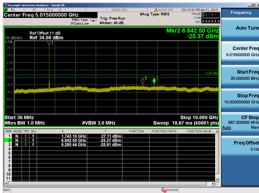
LTE Band 66, 4 / 5MHz / 64QAM - RB Size/Offset (1/0) – Mid Channel
