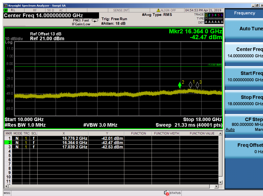
LTE Band 66, 4 / 1.4MHz / 64QAM - RB Size/Offset (6/0) – Mid Channel
