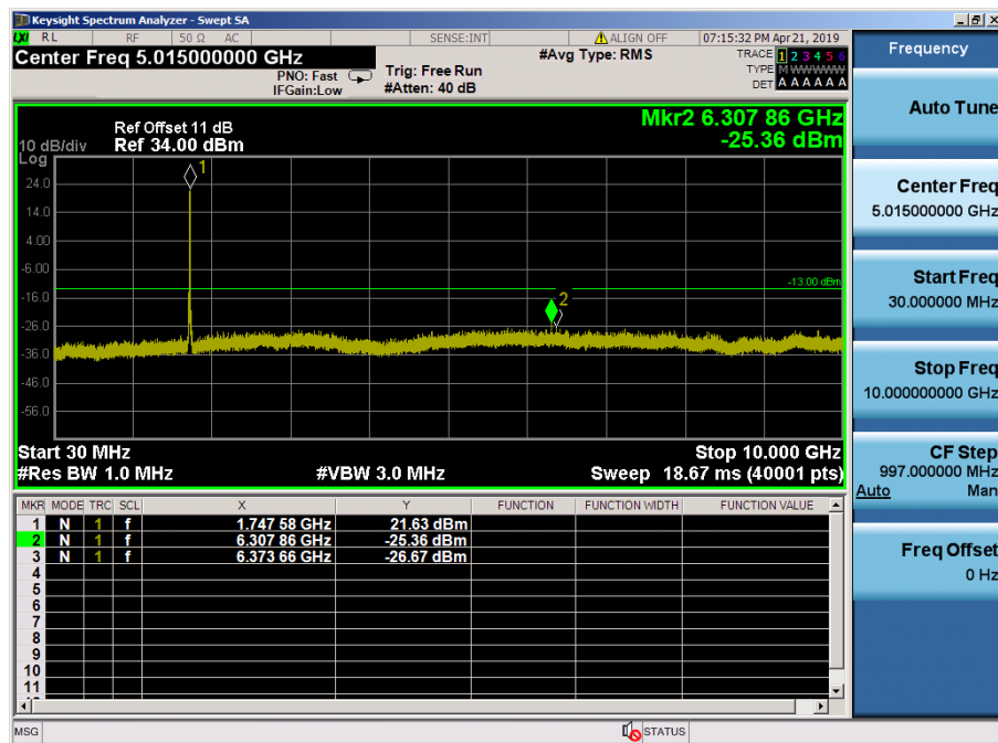
LTE Band 66, 4 / 10MHz / 64QAM - RB Size/Offset (50/0)– Mid Channel
