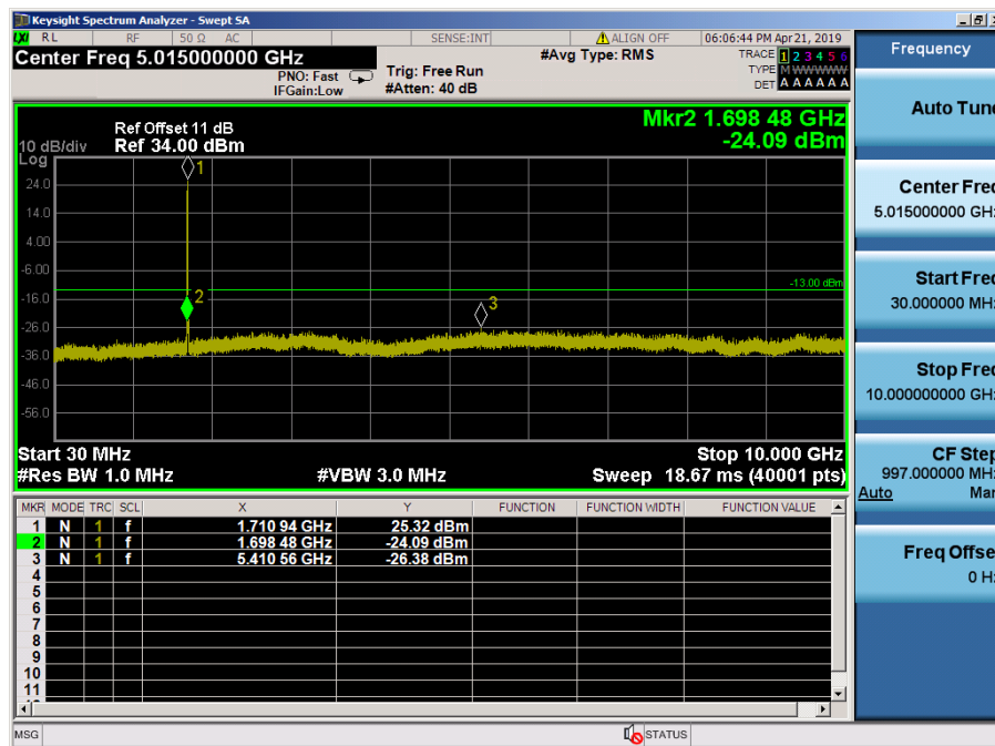
LTE Band 66, 4 / 5MHz / 64QAM - RB Size/Offset (12/0) – Low Channel
