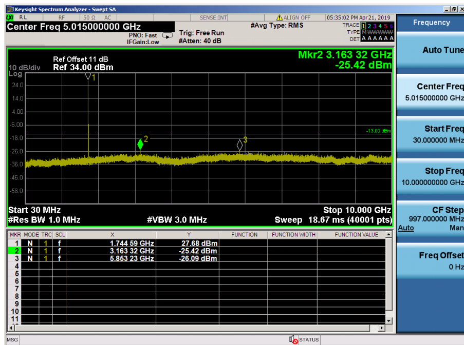
LTE Band 66, 4 / 3MHz / 64QAM - RB Size/Offset (8/0) – Mid Channel
