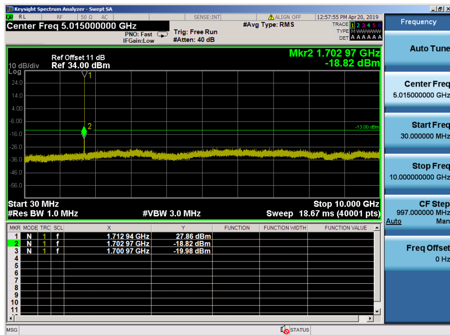
LTE Band 66, 4 / 3MHz / QPSK - RB Size/Offset (1/14) – Low Channel
