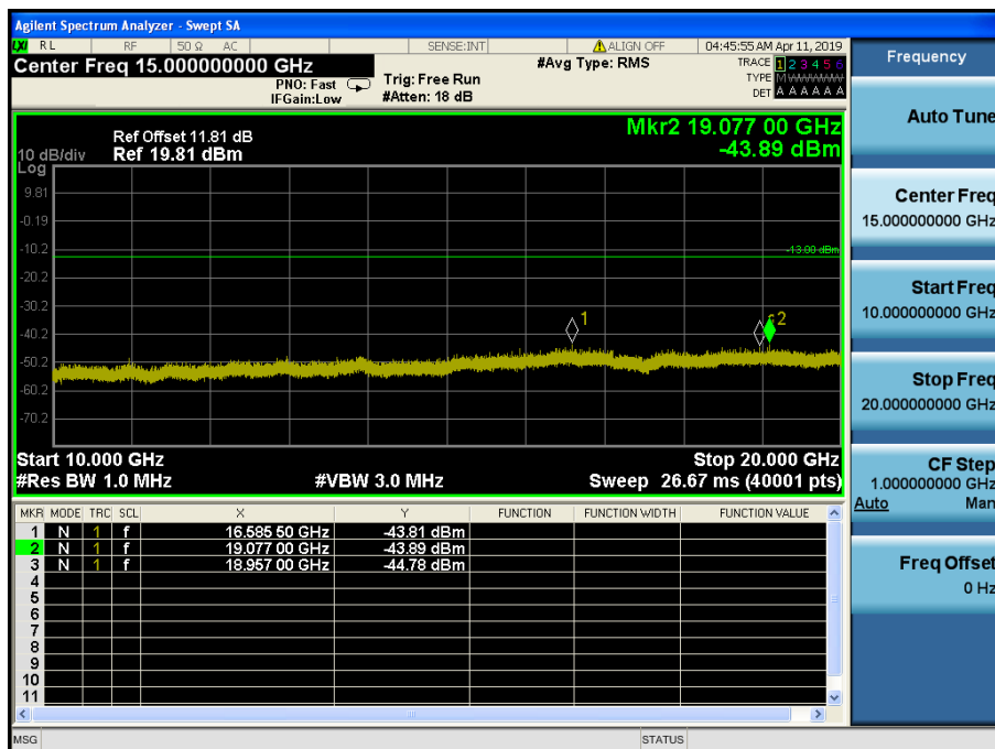
LTE Band 2 / 3MHz / 64QAM - RB Size/Offset (15/0) – Mid Channel
