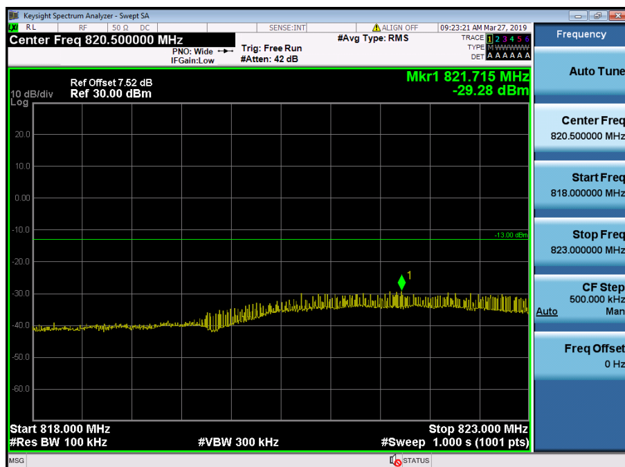
LTE Band 5, 26 / 5MHz / QPSK - RB Size/Offset (25/0)
