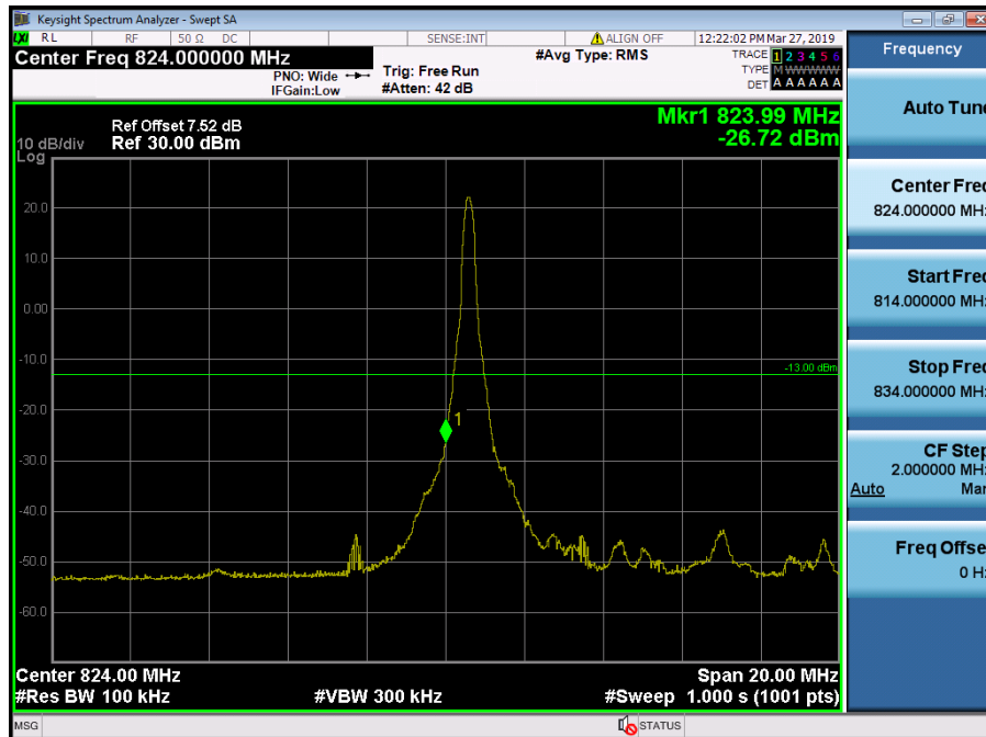
LTE Band 5, 26 / 10MHz / 16QAM - RB Size/Offset (1/0)
