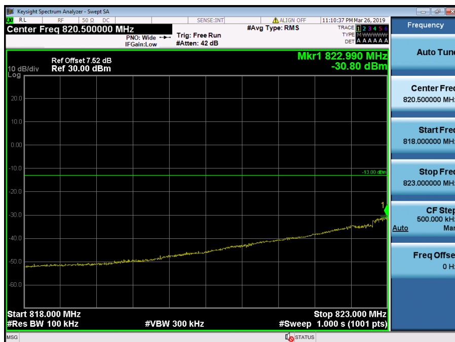
LTE Band 5, 26 / 1.4MHz / 64QAM - RB Size/Offset (6/0)
