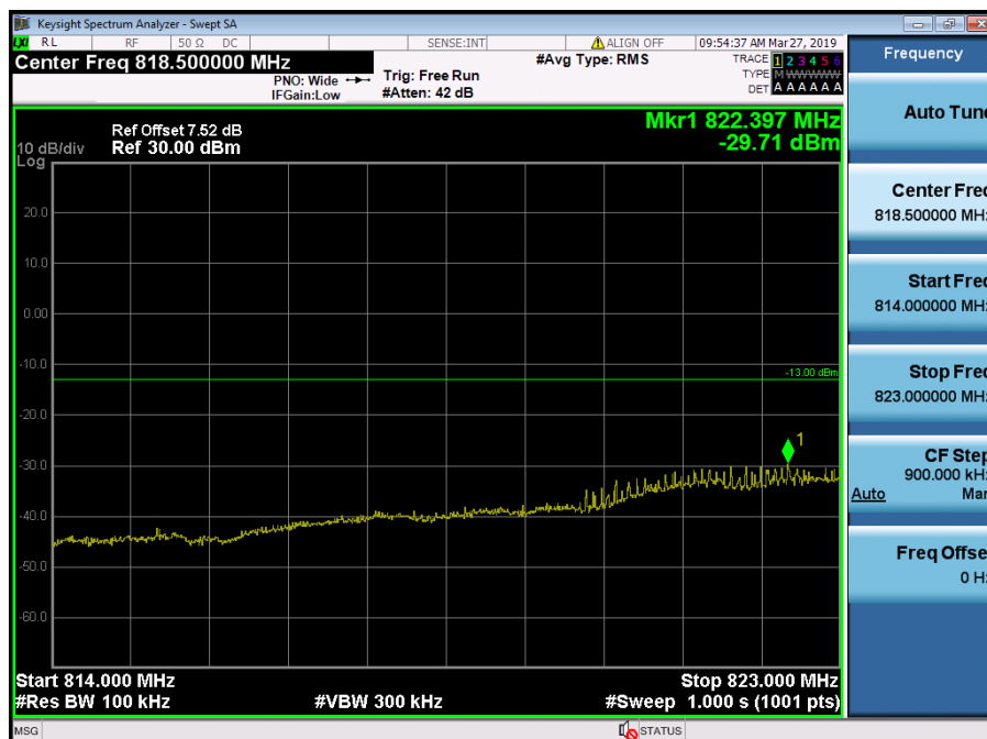
LTE Band 5, 26 / 10MHz / QPSK - RB Size/Offset (25/0)
