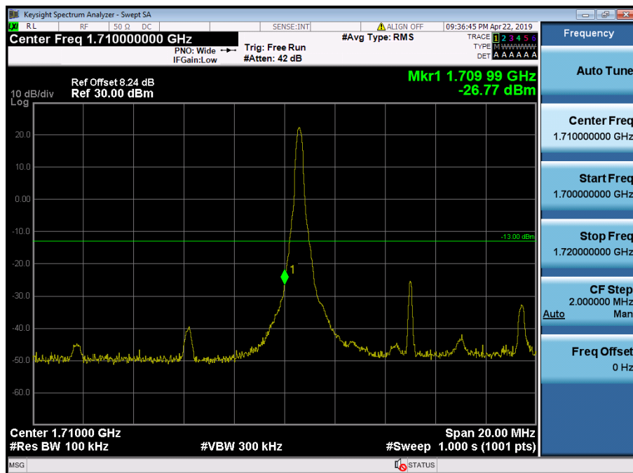
LTE Band 66, 4 / 10MHz / 16QAM - RB Size/Offset (1/0)
