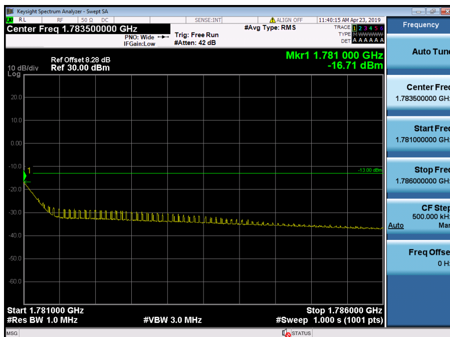
LTE Band 66, 4 / 5MHz / 64QAM - RB Size/Offset (25/0)
