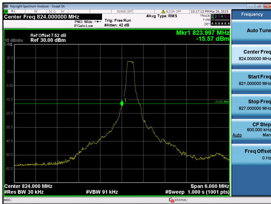
LTE Band 5, 26 / 3MHz / 16QAM - RB Size/Offset (1/0)
