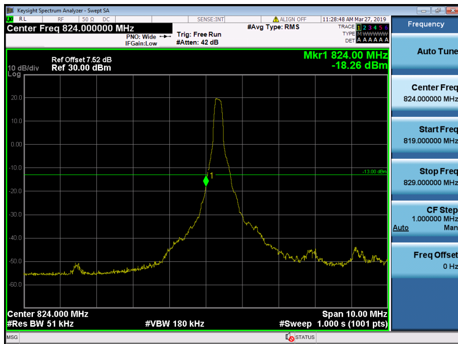
LTE Band 5, 26 / 5MHz / 16QAM- RB Size/Offset (1/0)
