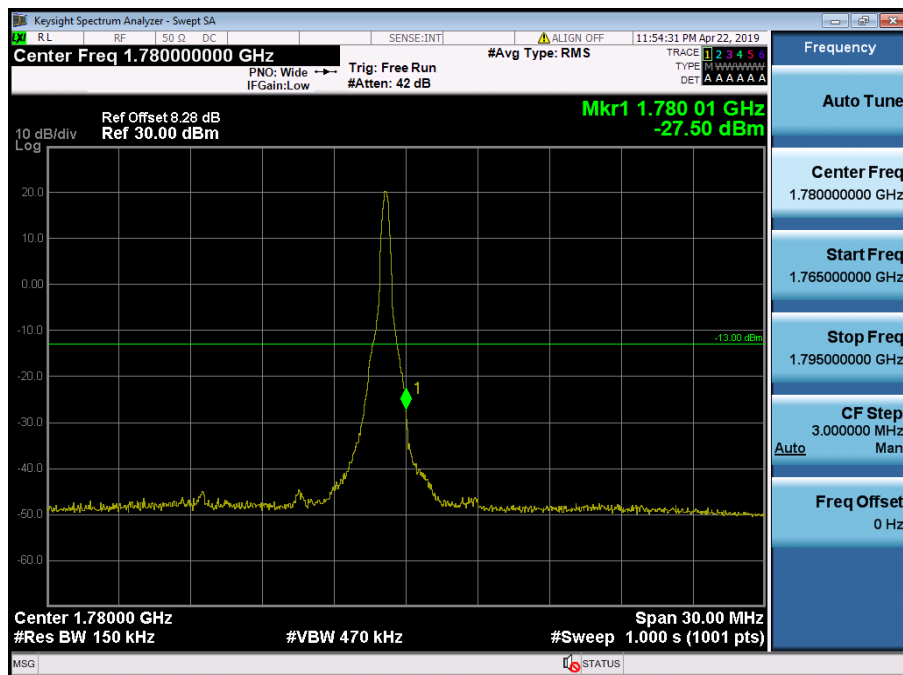
LTE Band 66, 4 / 15MHz / 16QAM - RB Size/Offset (1/74)
