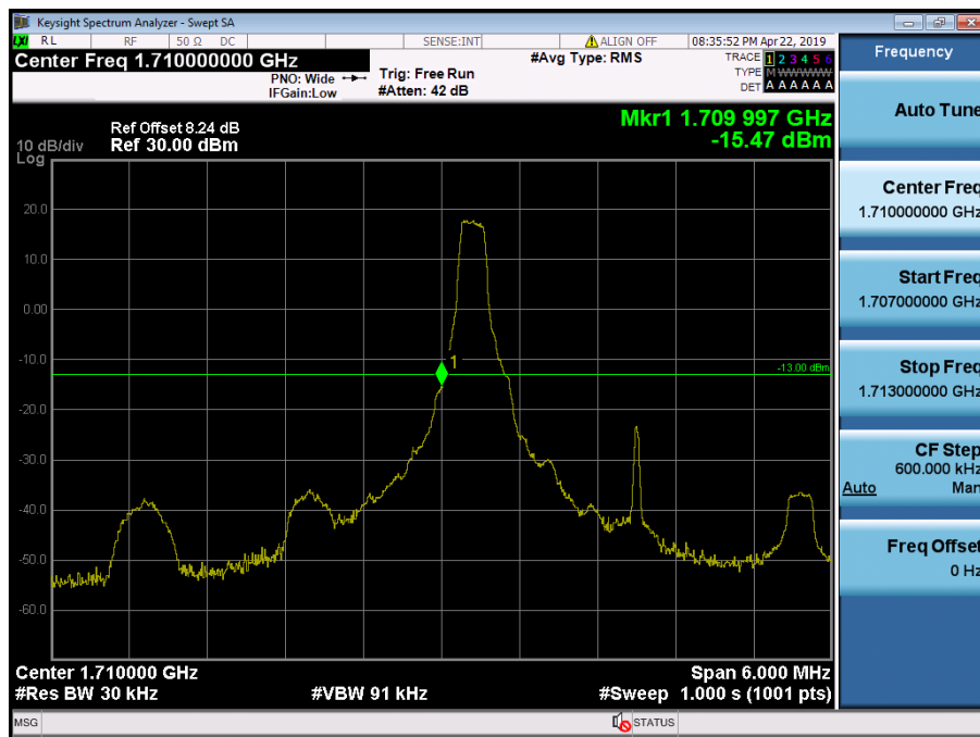
LTE Band 66, 4 / 3MHz / 16QAM - RB Size/Offset (1/0)
