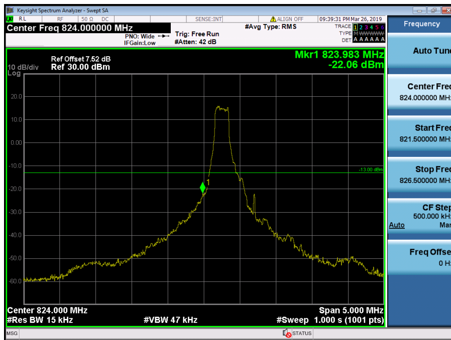
LTE Band 5, 26 / 1.4MHz / 16QAM - RB Size/Offset (1/0)
