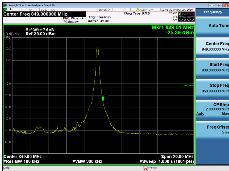
LTE Band 5, 26 / 10MHz / 16QAM - RB Size/Offset (1/49)
