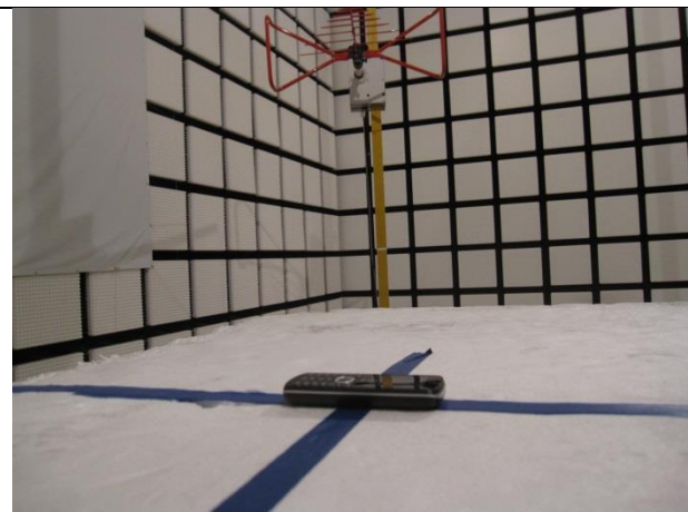
RADIATED PHOTO (BELOW 1 GHz)
