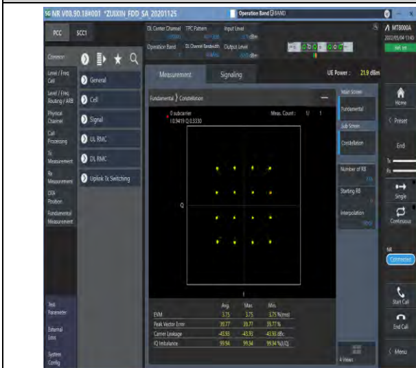
1-N7-PC3-15-40-M-3-DFT-16QAM-Outer_Full-216 @0-Ant1-see graph-PASS
