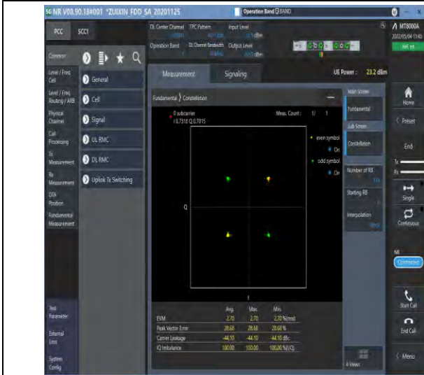
1-N7-PC3-15-40-M-1-DFT-PI2BPSK-Outer_Full-216 @0-Ant1-see graph-PASS
