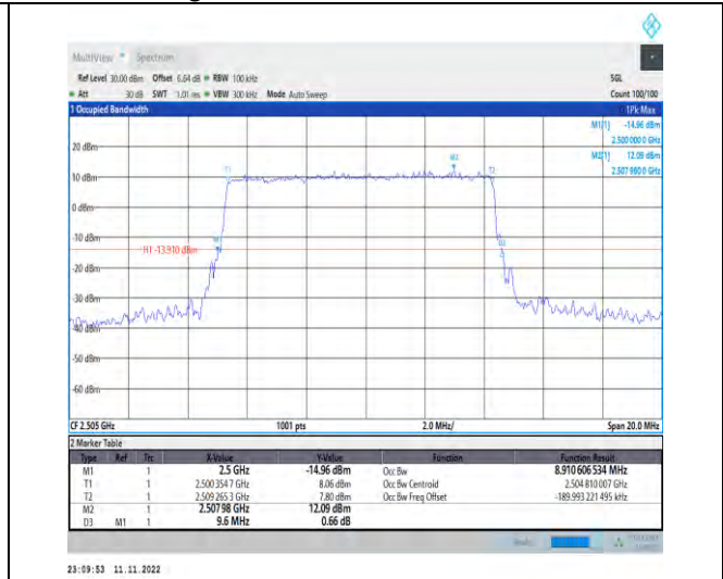
1-N7-PC3-15-10-L-3-DFT-16QAM-Outer_Full-50@0- Ant1-8.911-9.600-≤10-PASS
