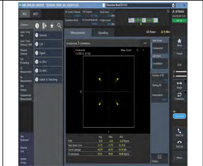
1-N7-PC3-15-40-M-2-DFT-QPSK-Outer_Full-216 @0-Ant1-see graph-PASS
