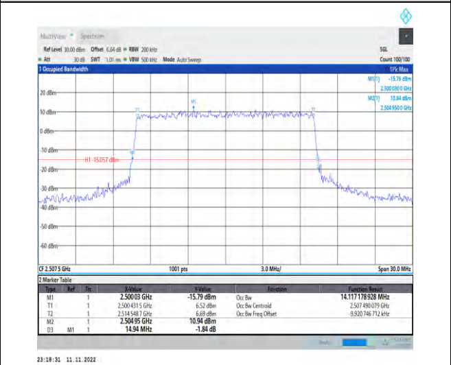
1-N7-PC3-15-15-L-6-CP-QPSK-Outer_Full-79@0-Ant1-14.117-14.940-≤15-PASS
