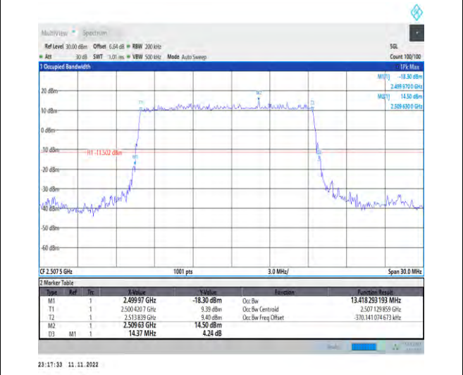
1-N7-PC3-15-15-L-2-DFT-PI2BPSK-Outer_Full-75@0-Ant1-13.418-14.370-≤15-PASS
