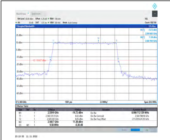
1-N7-PC3-15-10-H-4-DFT-64QAM-Outer_Full-50@0 -Ant1-8.906-9.580-≤10-PASS
